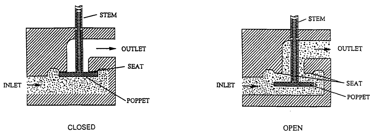
Figure 6.2 Poppet Valve Assembly
