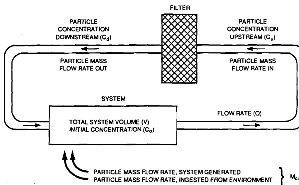
Figure 11.1 Simplified Fluid System with Filter
