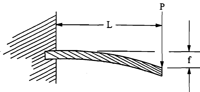
Figure 4.6 Typical Cantilever Spring
