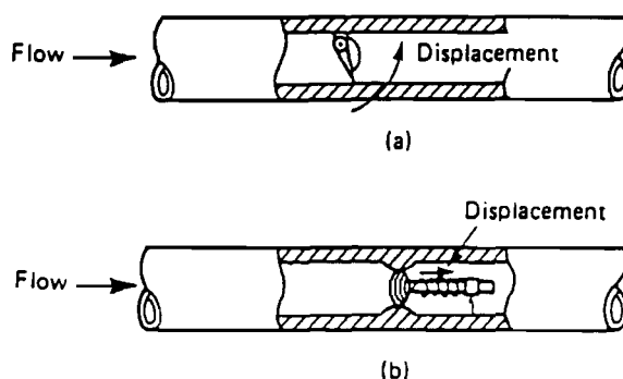
Figure 19.2 Typical Flow Transducer Units
