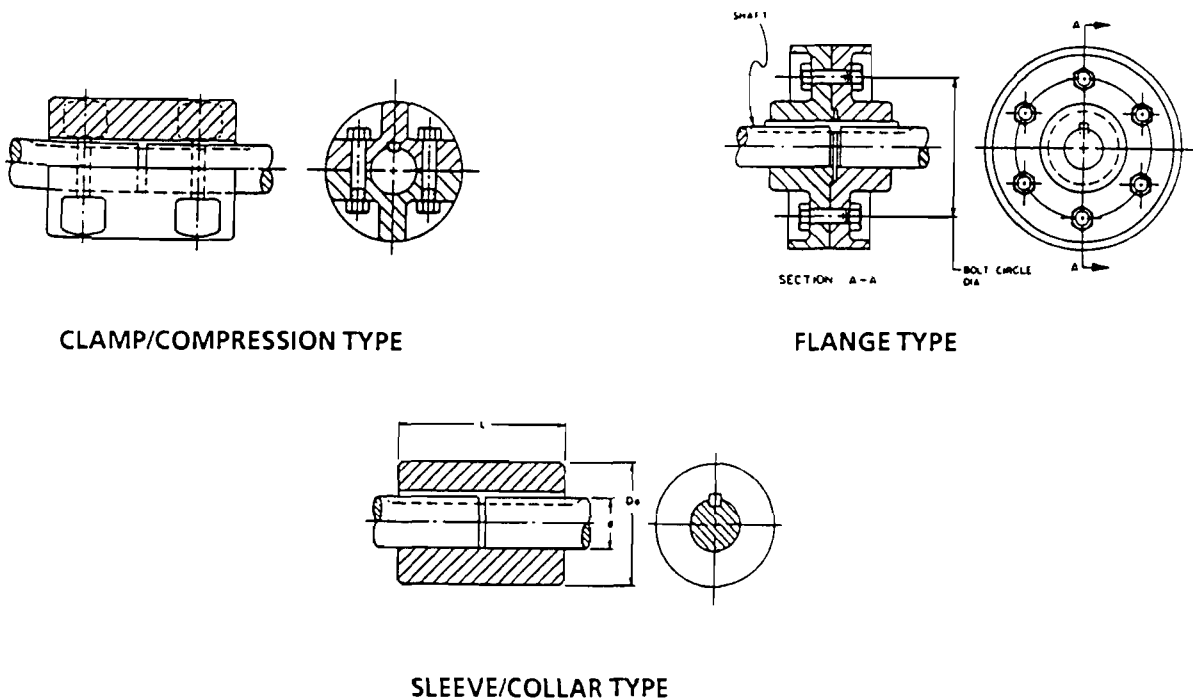
Figure 17.2 Rigid Couplings (Ref. 76)
