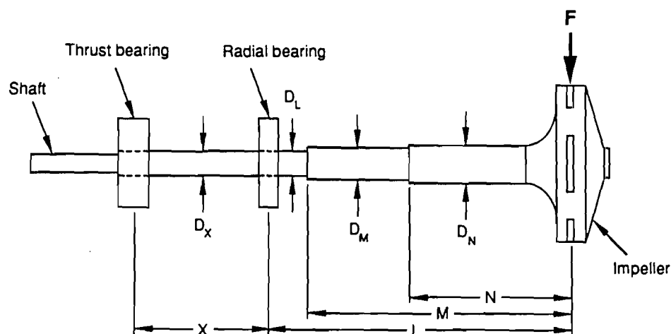
Figure 10.4 Typical Pump Shaft Assembly (Ref. 8)
