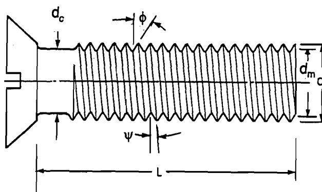
Figure 16.1 Typical Bolt and General Symbols
