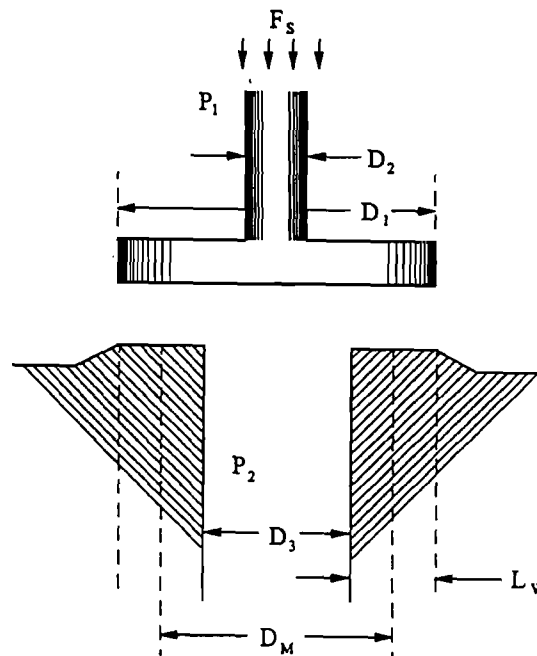
Figure 6.3 Typical Poppet/Valve Seat Configuration
