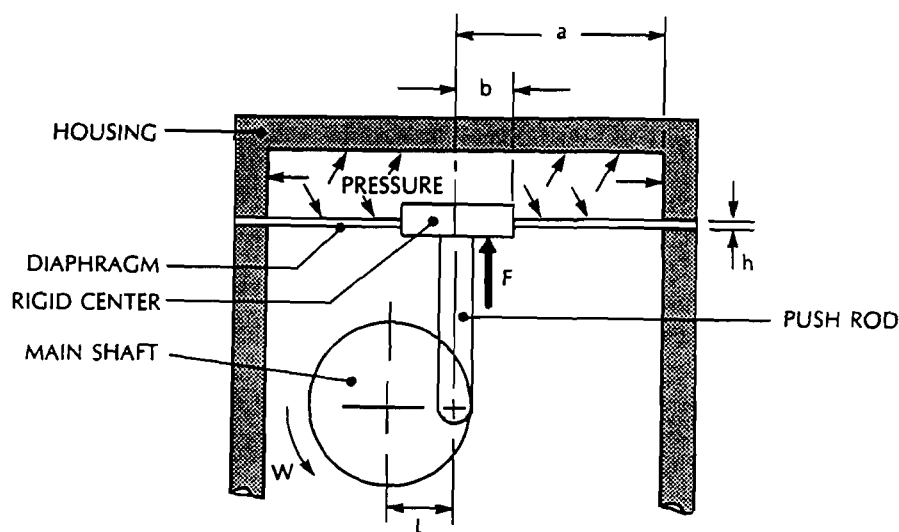
Figure 13.3 Compressor Diaphragm Model
