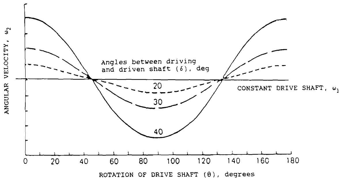
Figure 17.8 Velocity Characteristics of a Universal Joint
