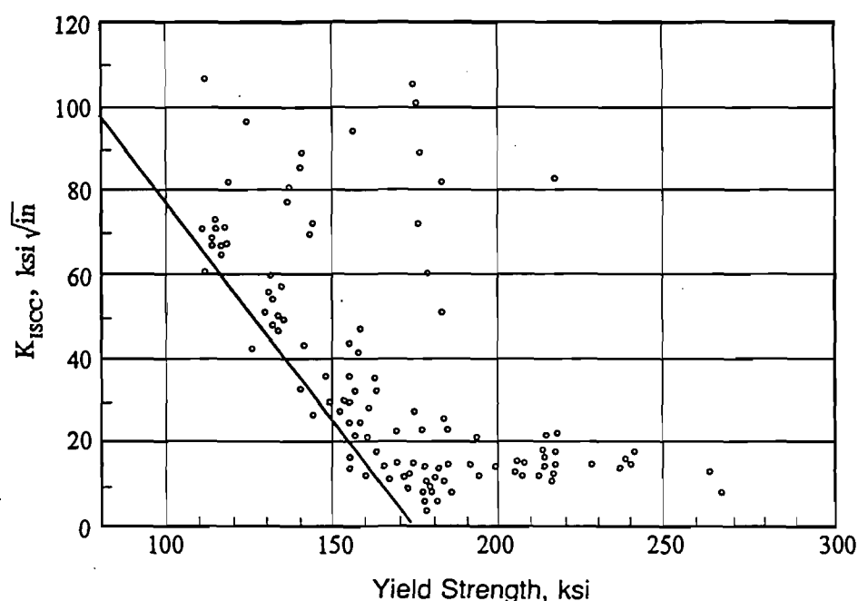
Figure 16.5 K_{ISCC} Factor vs. Material Yield Strength. (Low alloy, quenched & tempered material, in humid environment) (Ref.63)
