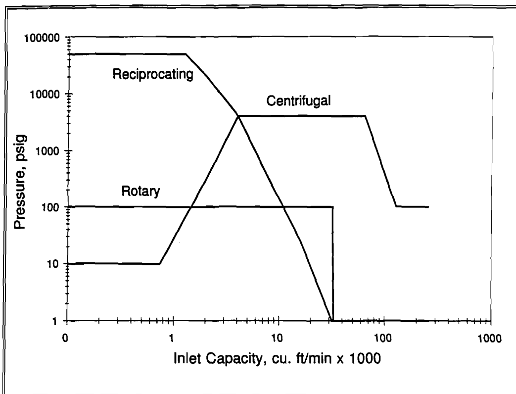
Figure 13.2 Operating Range of the Most Widely Used Compressors for Process Use (Boundaries are not absolute)
