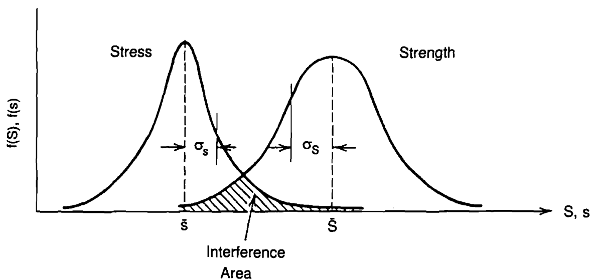
Figure 15.3 Stress Strength Relationship
