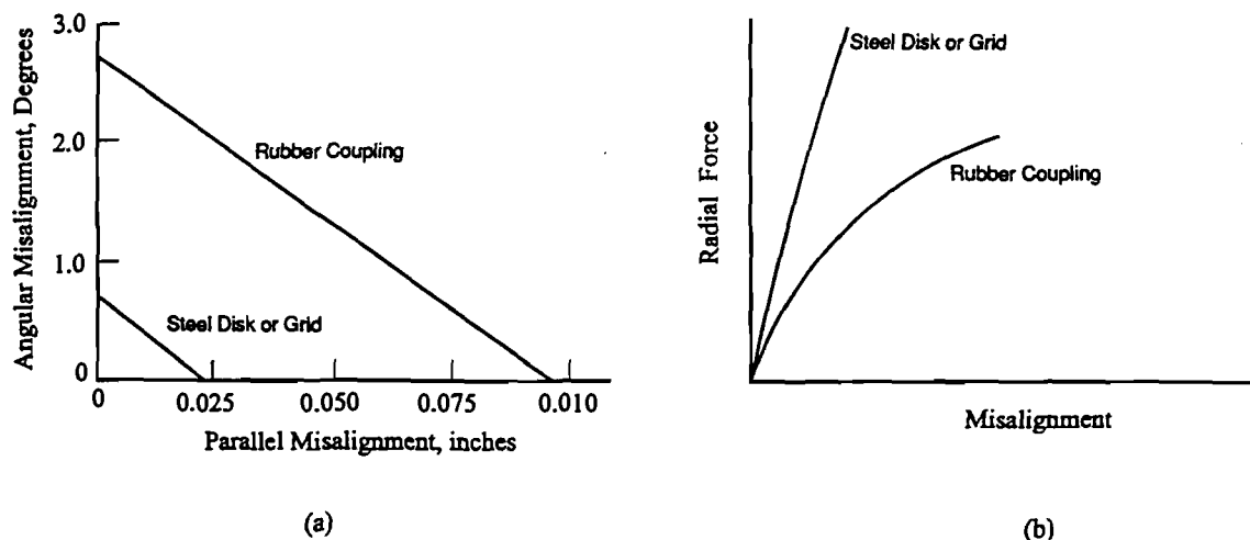
Figure 17.4 Coupling Characteristics
