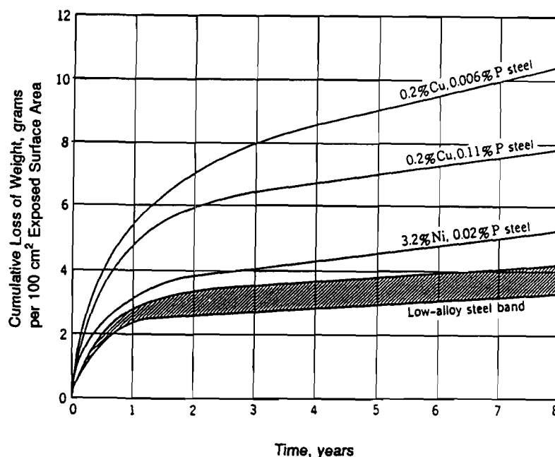
Figure 16.6 Typical Coupon Corrosion Penetration Test Results, (Low alloy steel in humid air) (Ref. 64)
