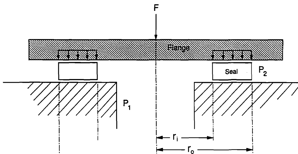
Figure 3.5 Typical Seal Installation
