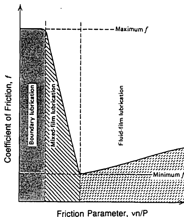
Figure 18.4 Variation of Friction Coefficient with the vn/P factor (Ref. 19)
