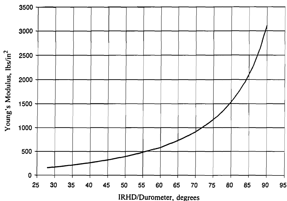
Figure 3.4 Seal Hardness and Young's Modulus
