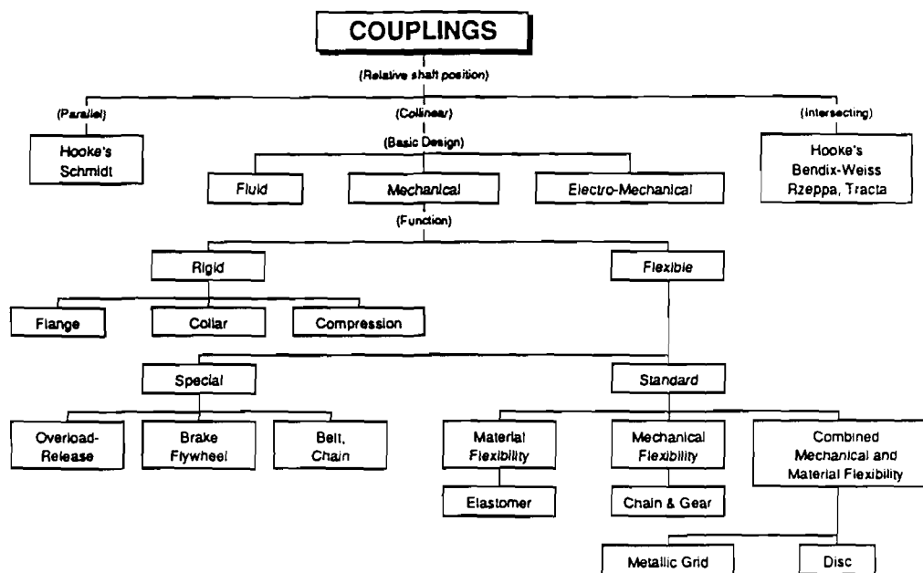
Figure 17.1 Common Classifications for Shaft Couplings (Ref. 75)
