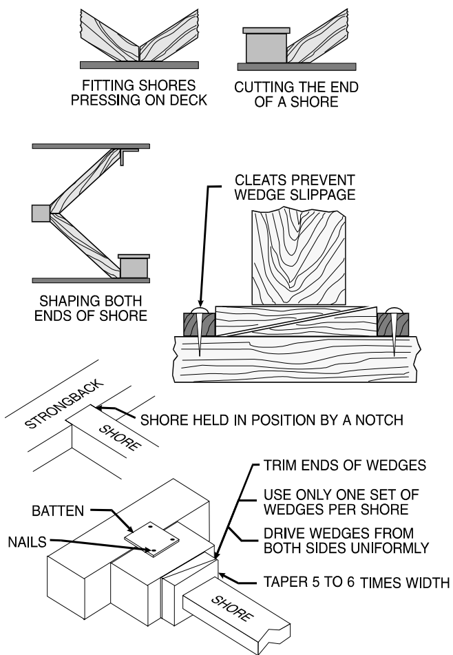
Figure 5-14. Anchoring Shores.
