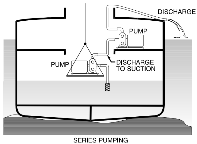
Figure 5-19A. Pumping Arrangements.
