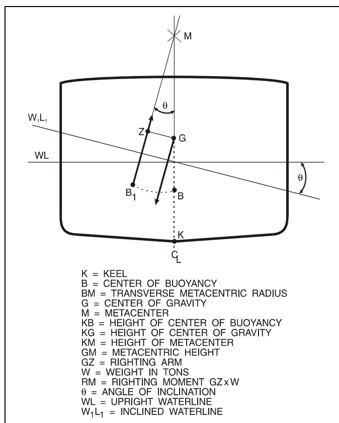
Figure 2-1. Centers, Heights and Righting Arm.
