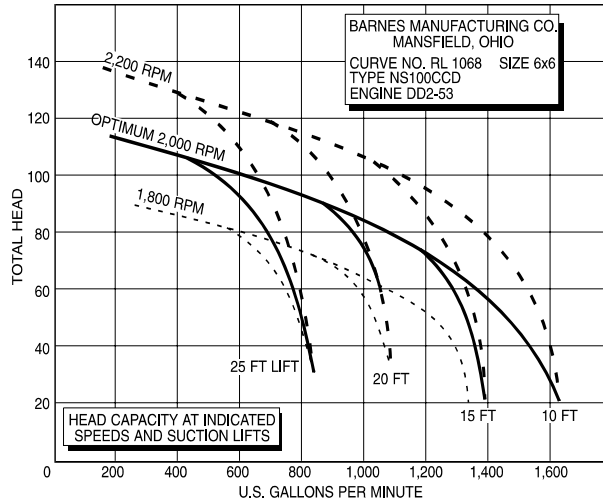
Figure 7-4B. Performance Curve, 6-inch Diesel Pump.
