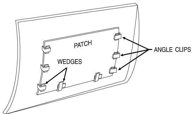
(b) WELDED STEEL PATCH (HELD IN PLACE WITH ANGLE CLIPS AND WEDGES FOR WELDING)
