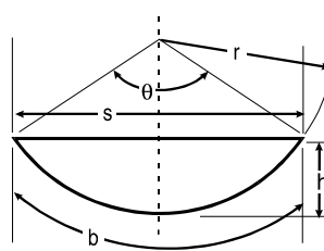
Figure 7-2B. Properties of Plane Surfaces.
