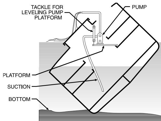
Figure 5-19C. Pumping Arrangements.
