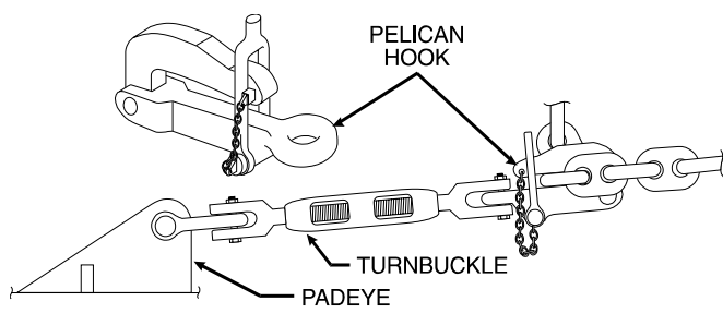
Figure 6-2. Chain Stopper.
