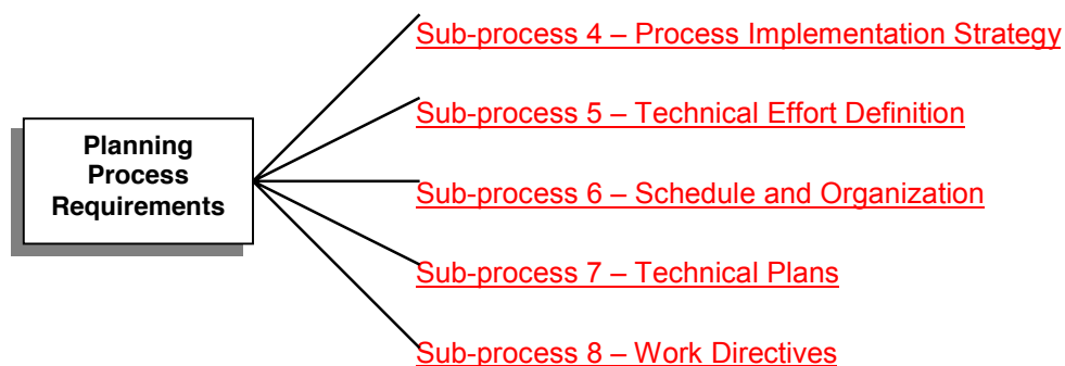
Figure 4.2.1 – Planning Process/Sub-processes
