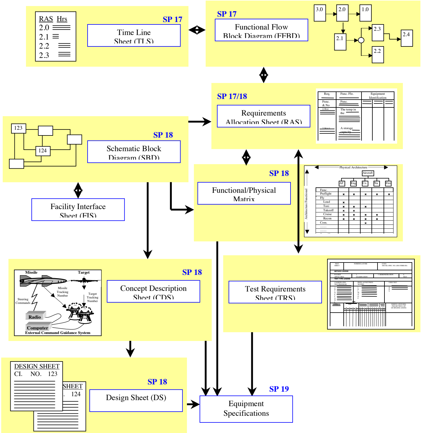
The three sub-processes associated with the Solution Definition Process are shown in Figure 4.3.2.
