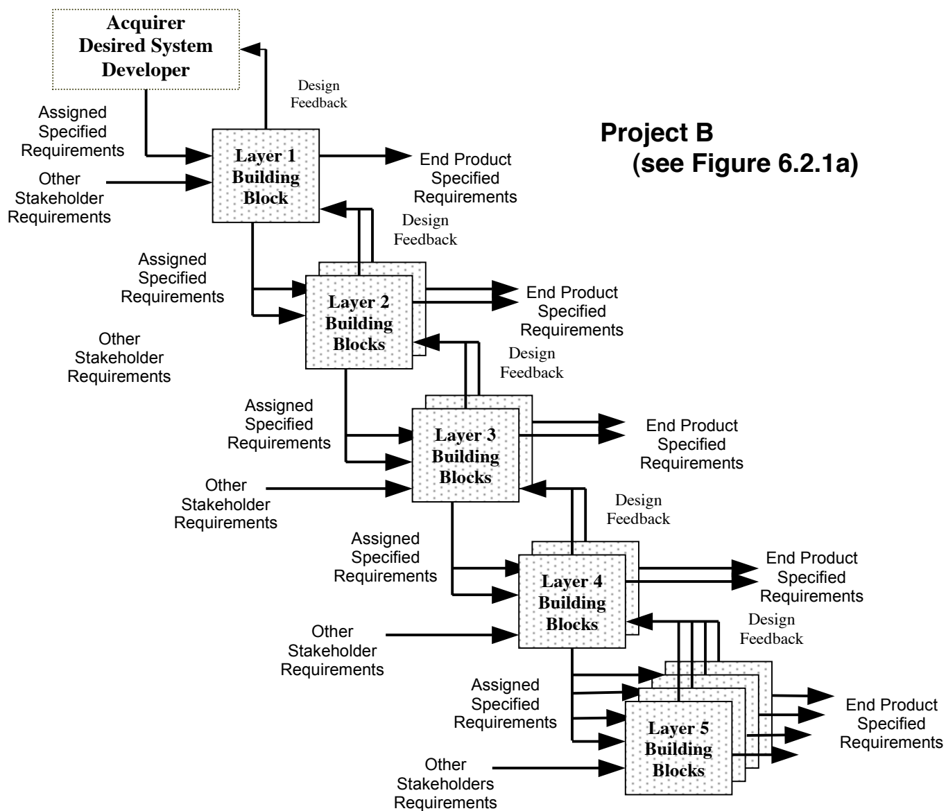
Figure 6.2.1b—Top-down development
