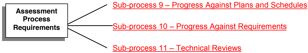
Figure 4.2.2 – Assessment Process/Sub-processes
