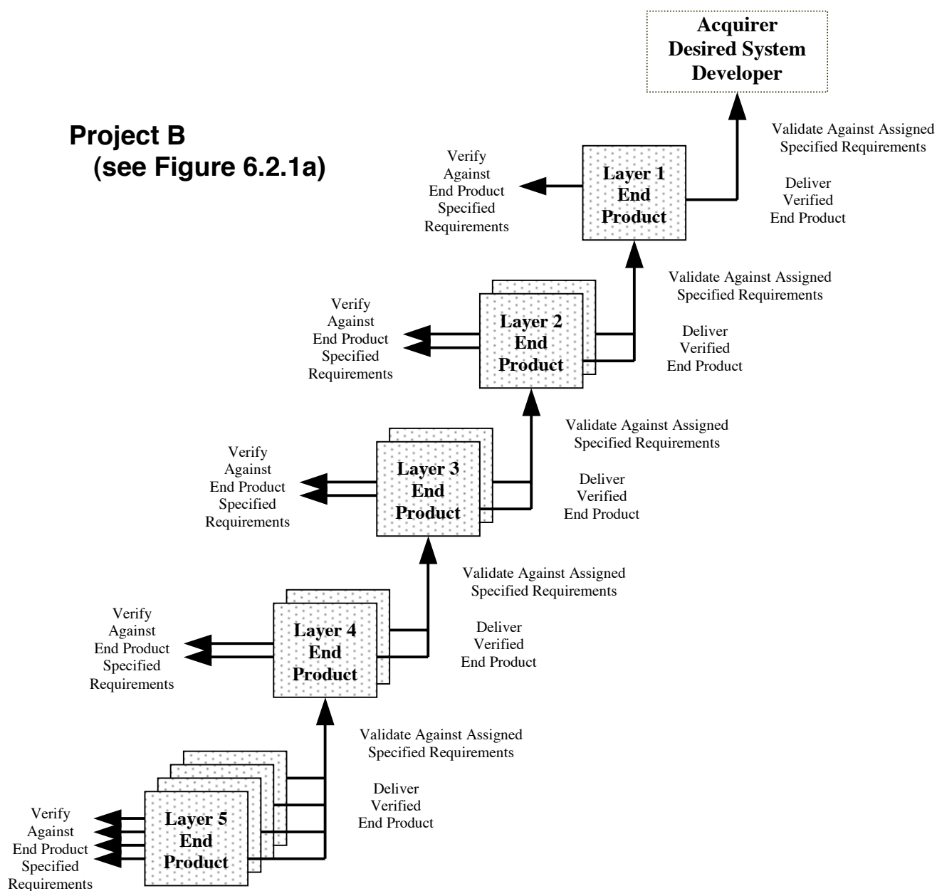
Figure 6.2.2—Bottom-up realization
