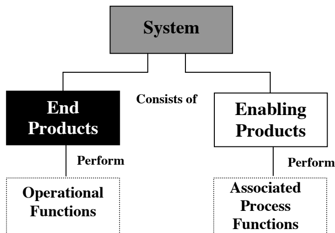
Figure 6.1 – System concept
