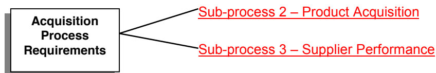
Figure 4.1.2 – Acquisition Process/Sub-processes
