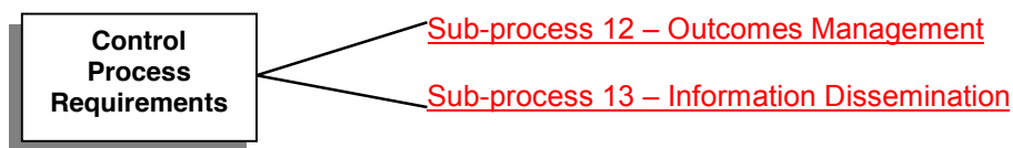
Figure 4.2.3 – Control Process/Sub-processes
