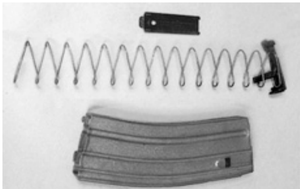
Figure 2-19. Magazine Disassembled.
