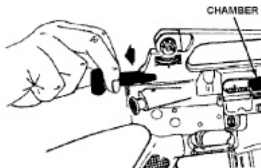
Figure 2-5. Charging Handle.
