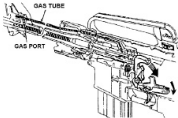
Figure 2-6. Firing.
