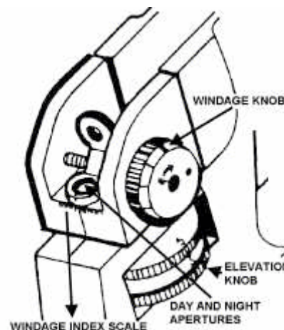
Figure 9-4. Rear Sight.
