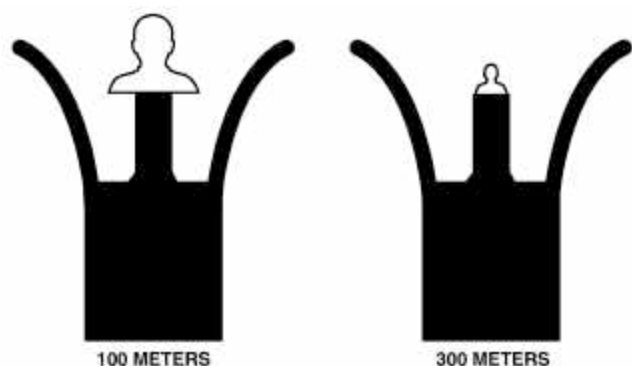
Figure 10-3. Front Sight Post Method.
