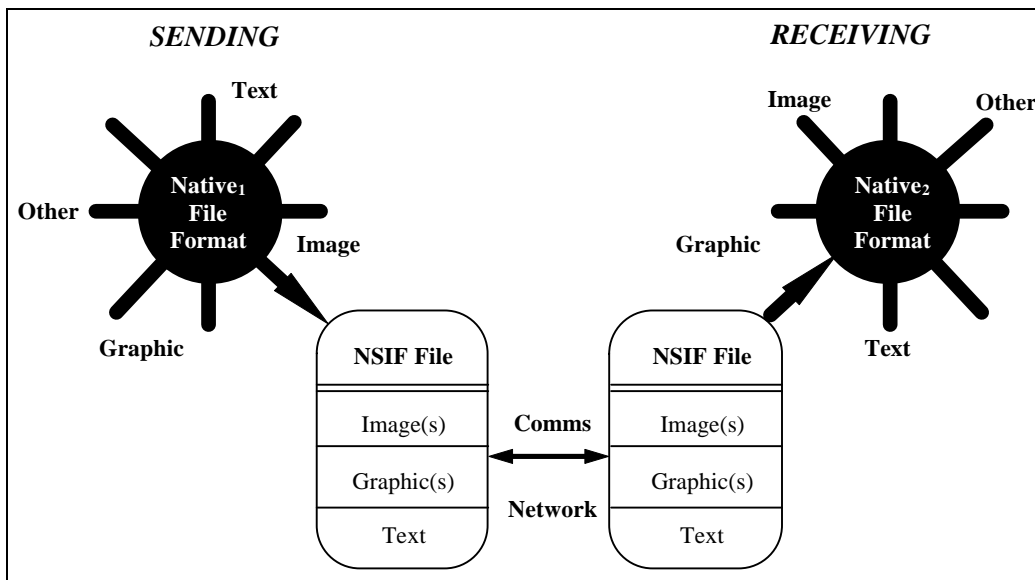
Figure B-2. NSIF Functional Architecture
