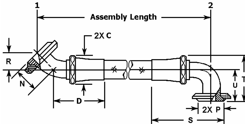
FIGURE 11. Style M hose assembly.
