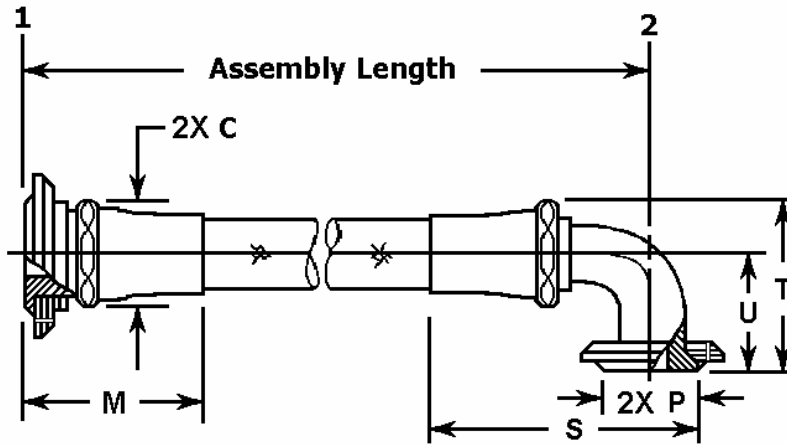
FIGURE 9. Style J hose assembly.
