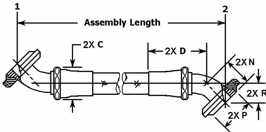
FIGURE 10. Style K hose assembly.
