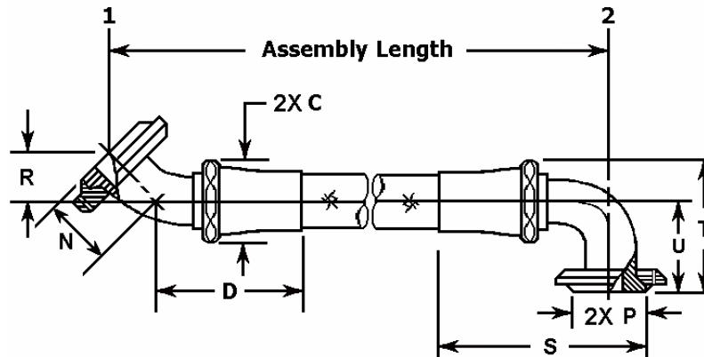
FIGURE 5. Style E hose assembly.
