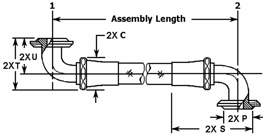
FIGURE 6. Style F hose assembly.
