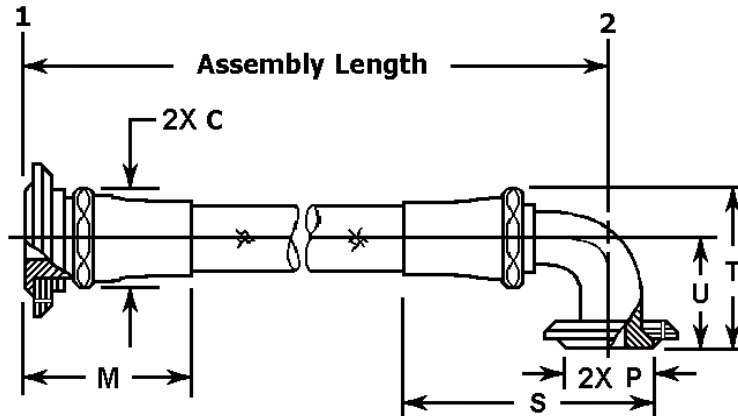
FIGURE 3. Style C hose assembly.
