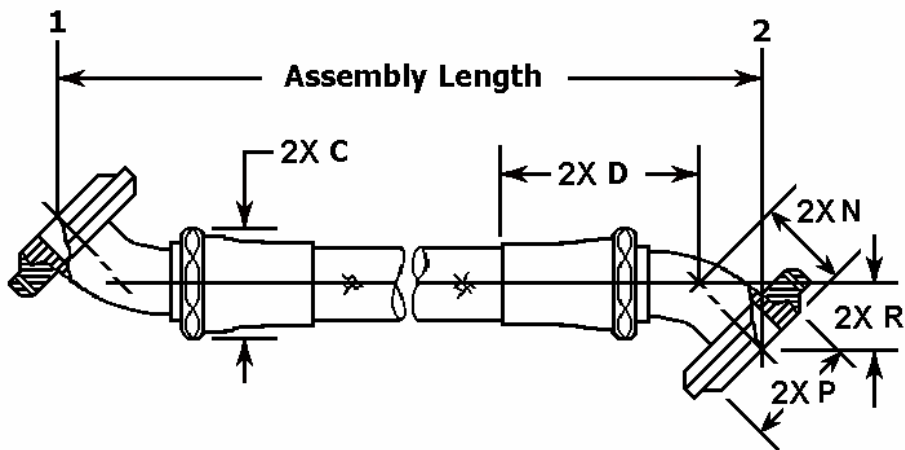
FIGURE 4. Style D hose assembly.
