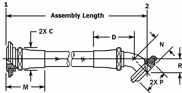
FIGURE 8. Style H hose assembly.
