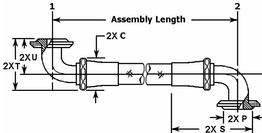
FIGURE 12. Style N hose assembly.
