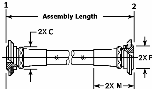
FIGURE 1. Style A hose assembly.
