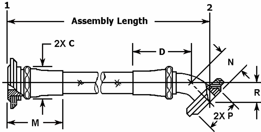
FIGURE 2. Style B hose assembly.
