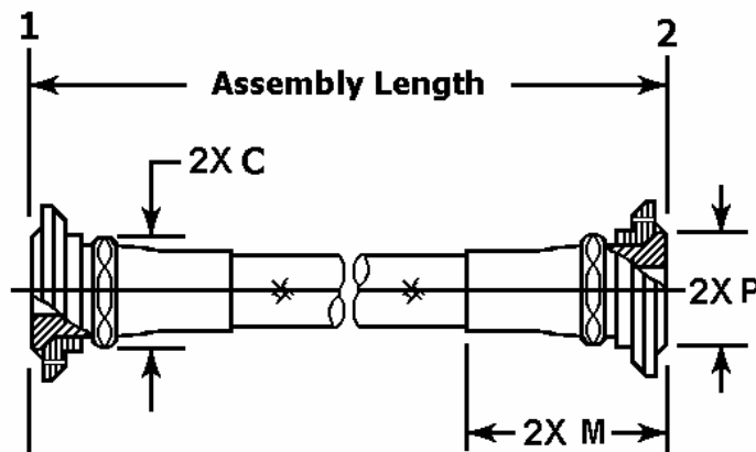
FIGURE 7. Style G hose assembly.
