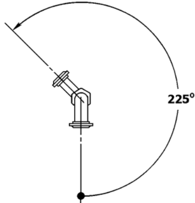
FIGURE 13. Measurement of angular alignment between elbow fittings.
