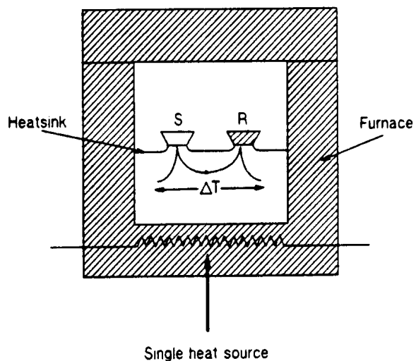
FIGURE 2. Heat flow DSC schematic diagram.
