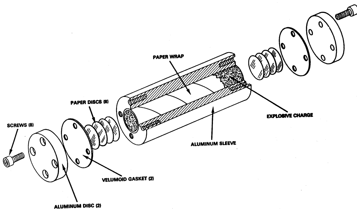
FIGURE 1. Apparatus for exudation test
