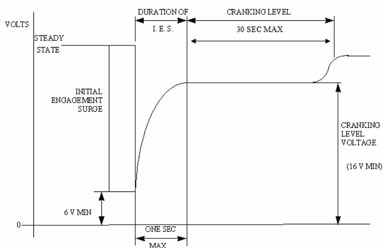
FIGURE 4. Starting Disturbances .
