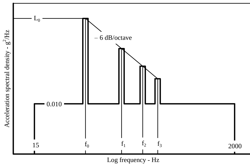
FIGURE 514.5C-9. Propeller aircraft vibration exposure.
