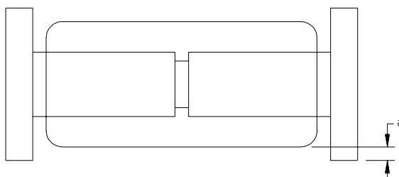
FIGURE 2074-D10. End-cap clearance.
