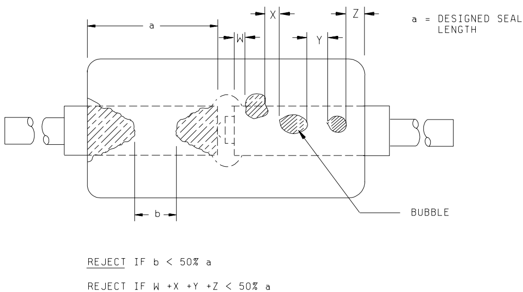
FIGURE 2074-C3. Insufficient seal .
