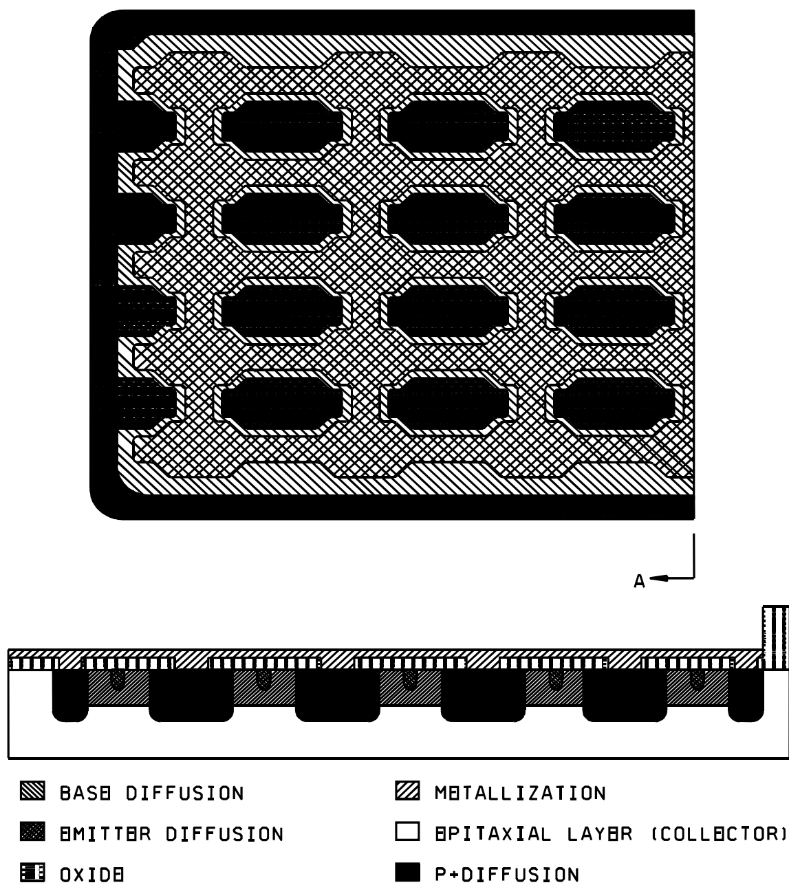
FIGURE 2070-5. Mesh geometry.
