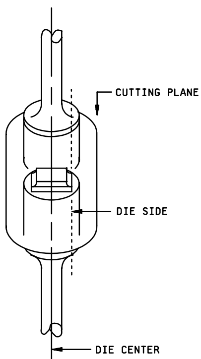
FIGURE 2101-1. Axial lead or surface mount construction.
