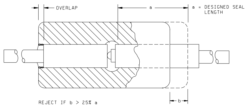
FIGURE 2074-C2. High seal .
