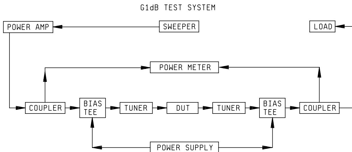
FIGURE 3510-1. Test system .
