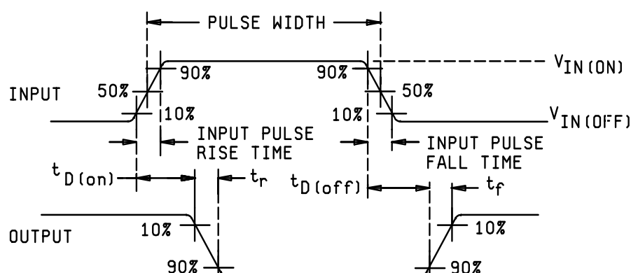
FIGURE 3459-1. Pulse characteristics .
