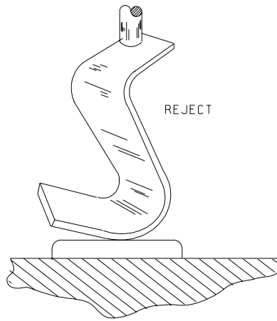
FIGURE 2074-A7. Heel contact.
