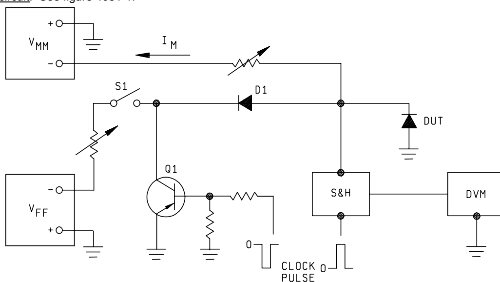
FIGURE 4081-1. Test circuit.
