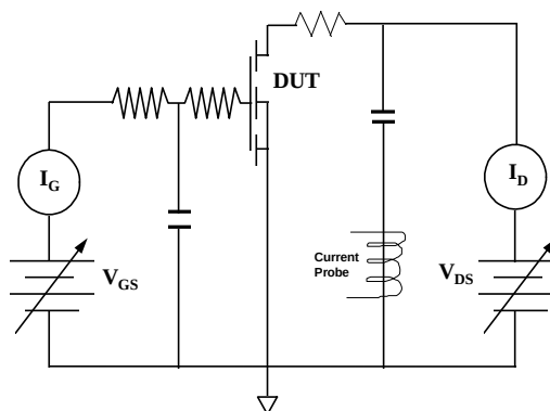
FIGURE 1080-2. SEB circumvention and monitoring circuit .
