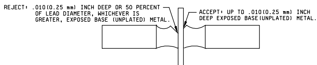
FIGURE 2071-8. Chip outs.
