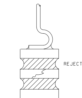
FIGURE 2074-G6. Die cracks.
