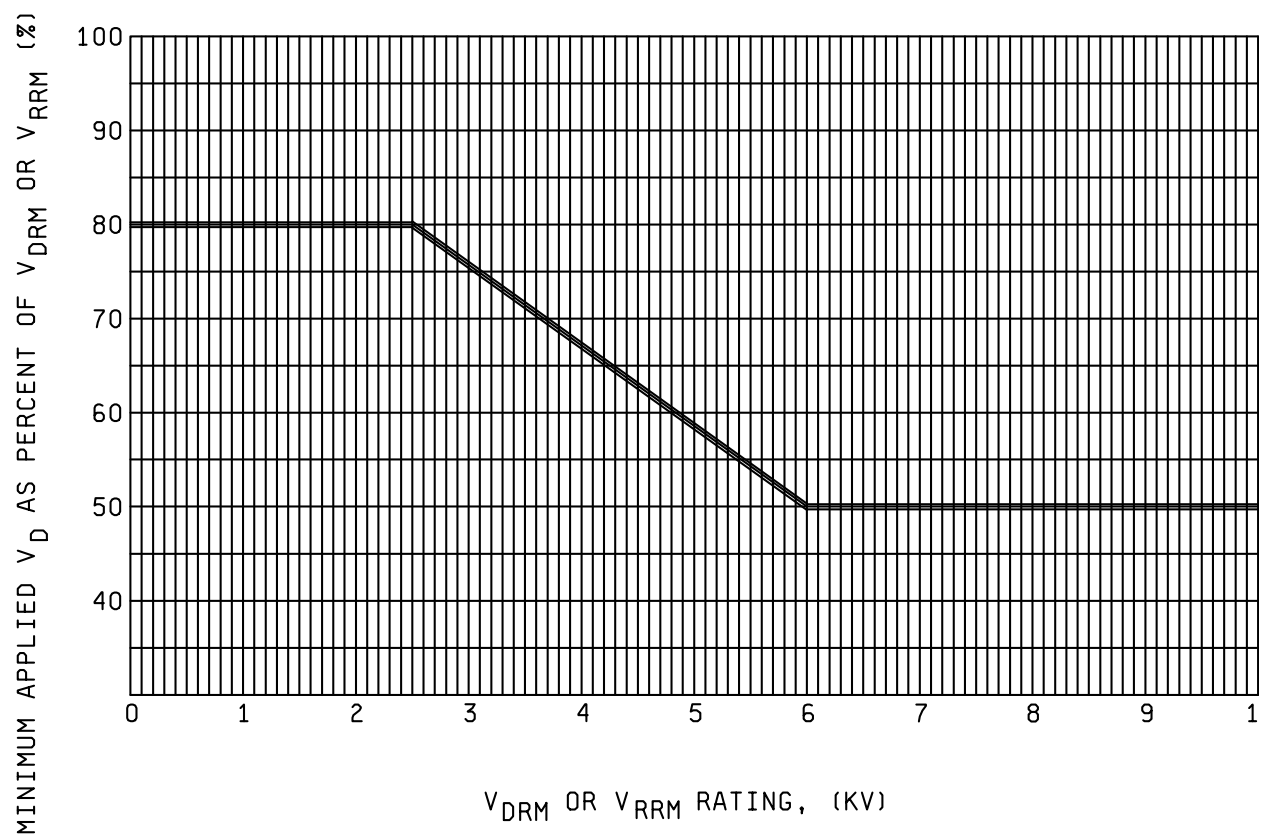
FIGURE 1038-1. Voltage requirement.
