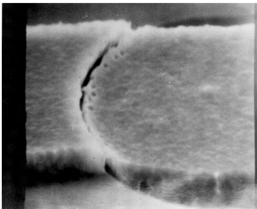
FIGURE 2077-15. (9,500X) Steep oxide step (MOS) (reject).
