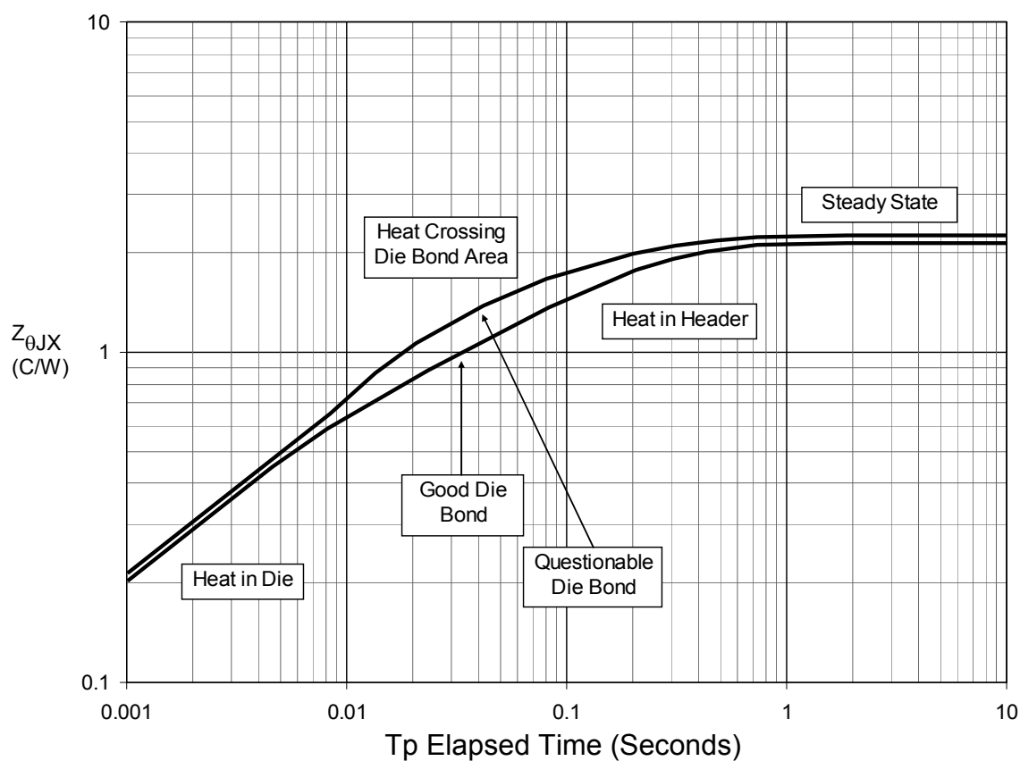
FIGURE 3131-4. Heating curves for two extreme devices.
