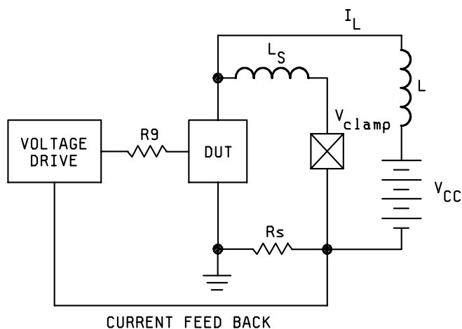
FIGURE 3490-1. Inductive load circuit.
