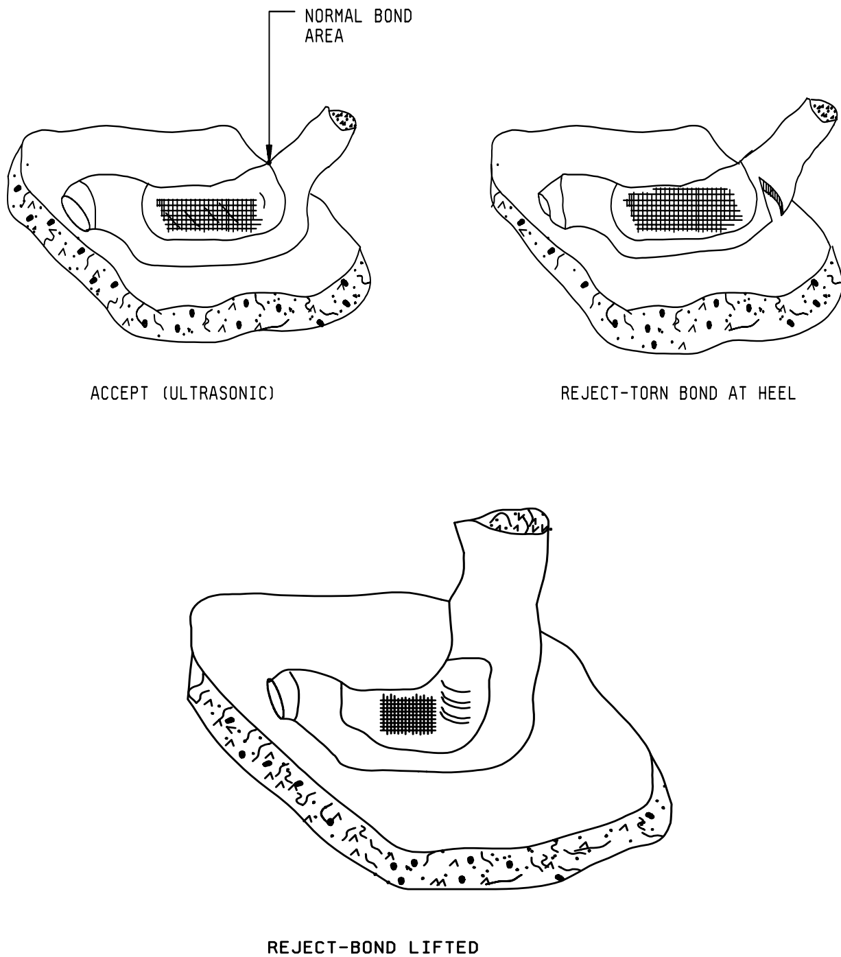
FIGURE 2072-5. Lift/torn bonds.
