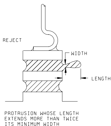
FIGURE 2074-G1. Solder protrusion.
