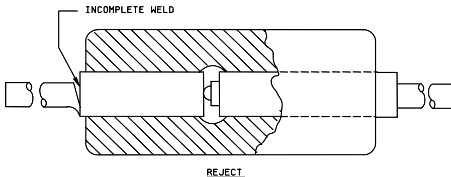
FIGURE 2074-C6. Incomplete weld.
