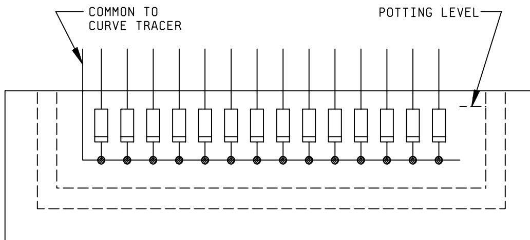
FIGURE 1054-1. Potted diodes .
