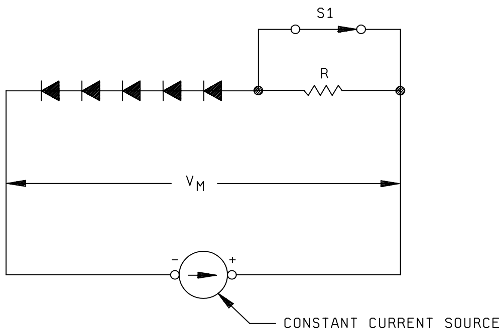
FIGURE 1055-2. Monitored mission cycle.
