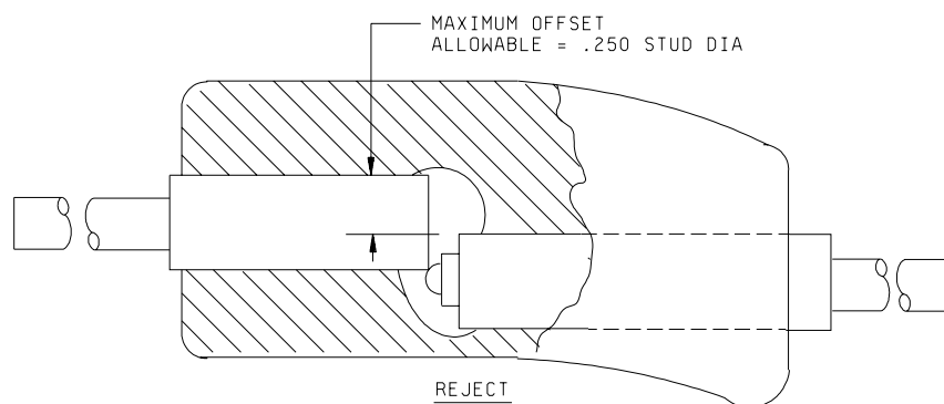
FIGURE 2074-C4. Plug alignment.
