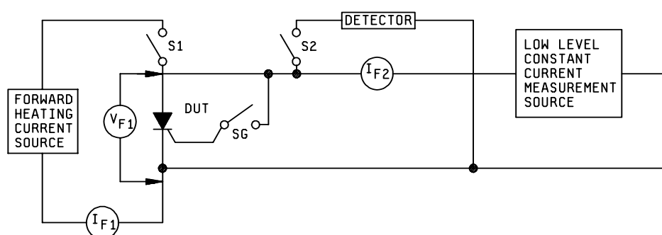
FIGURE 3181-1. Thermal resistance test circuit .
