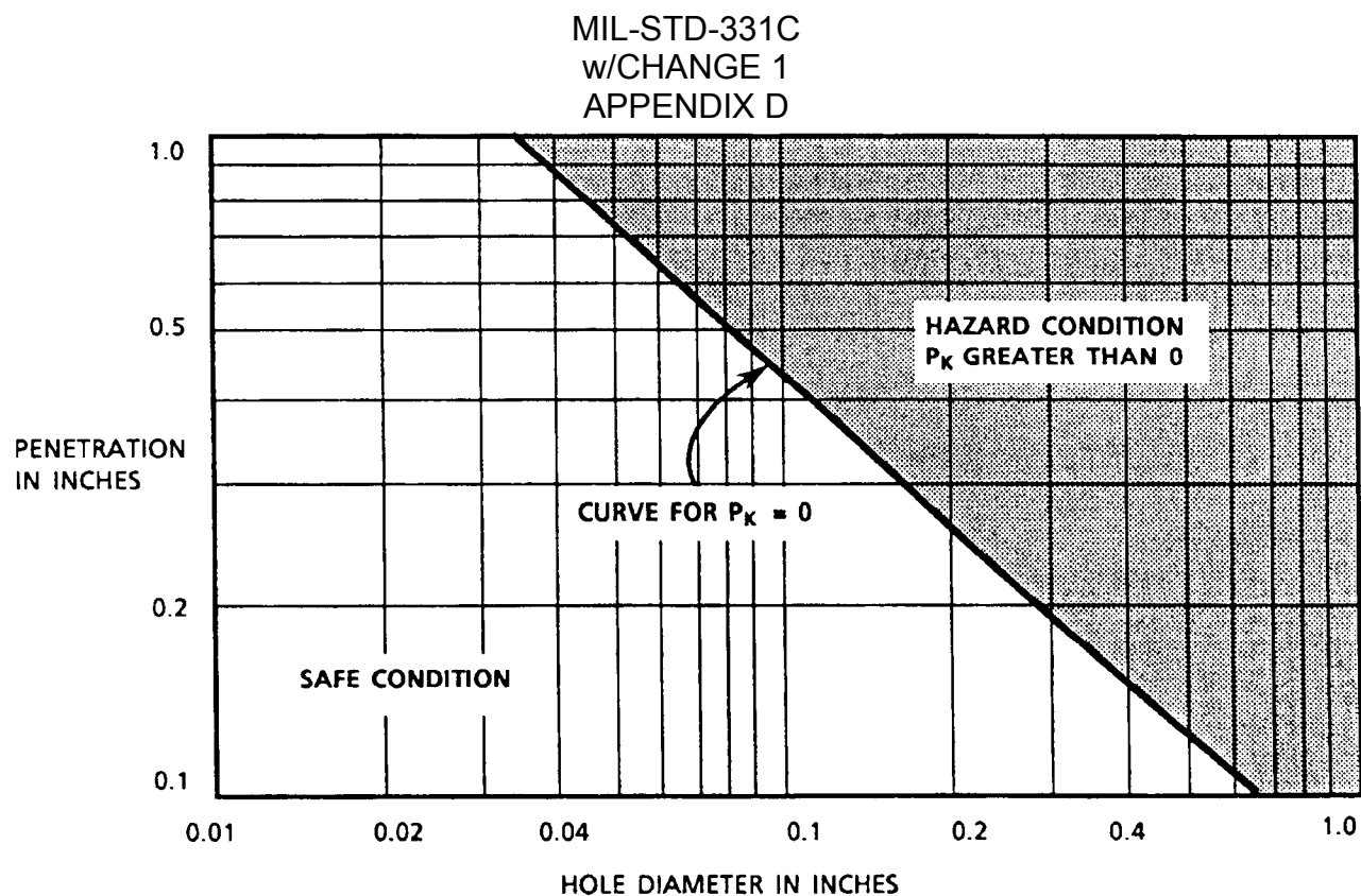
FIGURE D1-2. Penetration in Fiberboard Vs. Fragment Hole Size
