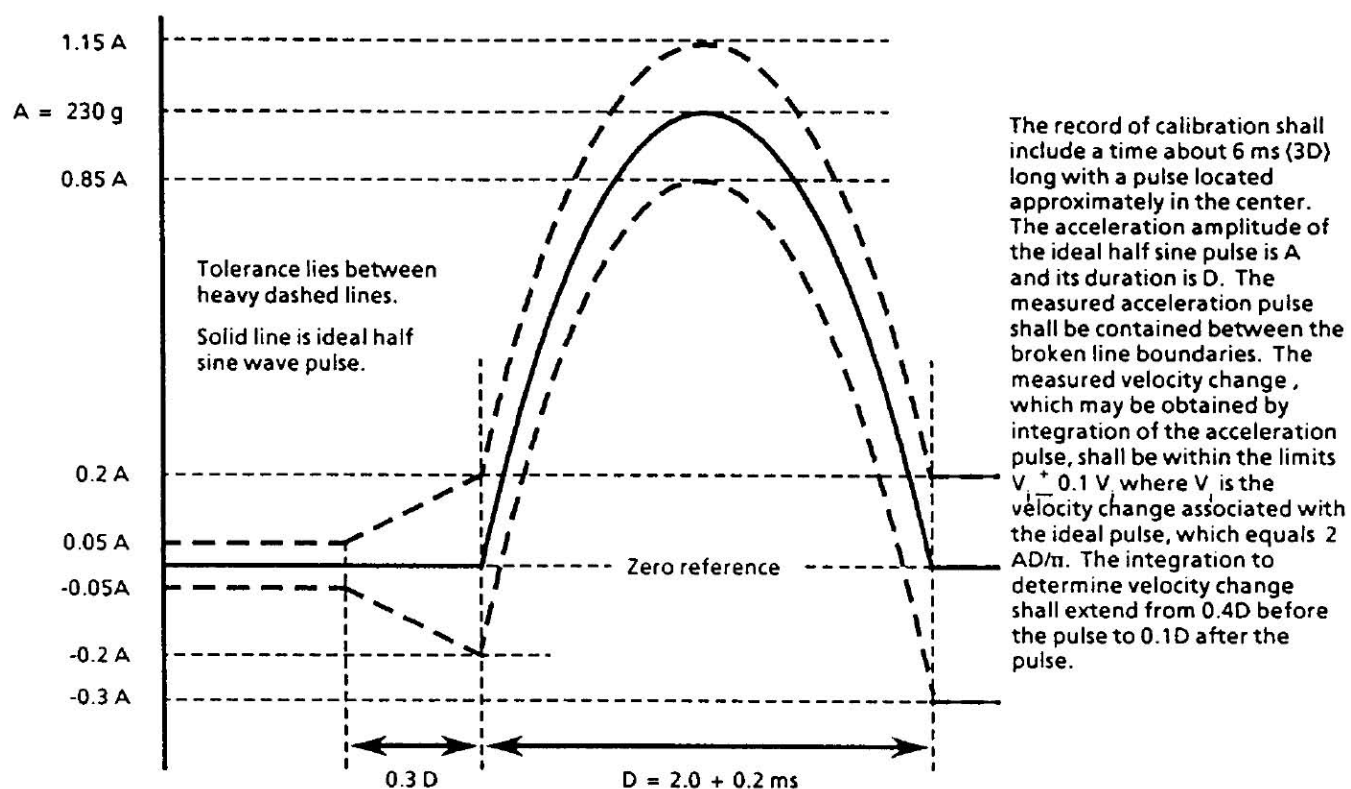
FIGURE A1-2. Half-Sine Shock Pulse and Tolerance
