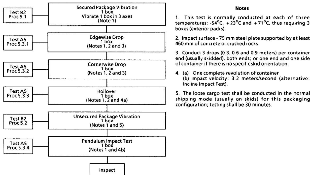
FIGURE A5-5. Typical Sequential Vibration-Handling (Packaged Fuzes) Test For Artillery, Mortar And Recoilless Rifle Ammunition, Cartridges And Fuzes (for exterior packages more than 68 kg (150 lb))
