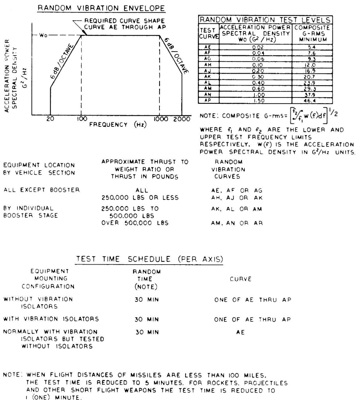
FIGURE B3-3. Random Vibration Frequencies, Levels And Test Times For Fuzes Installed In Shipboard-Launched Munitions
