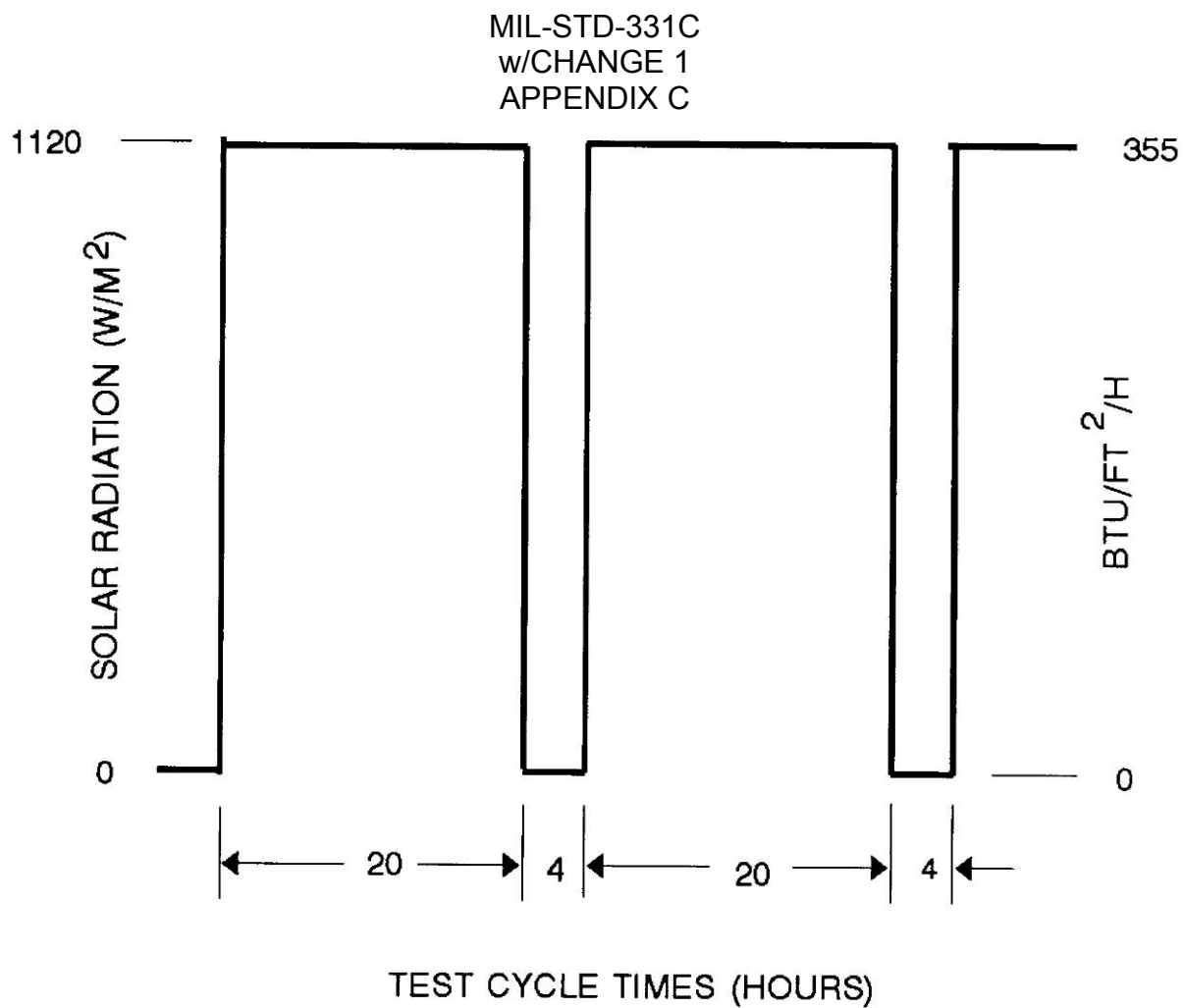
FIGURE C10-2. Two Steady State Cycles
