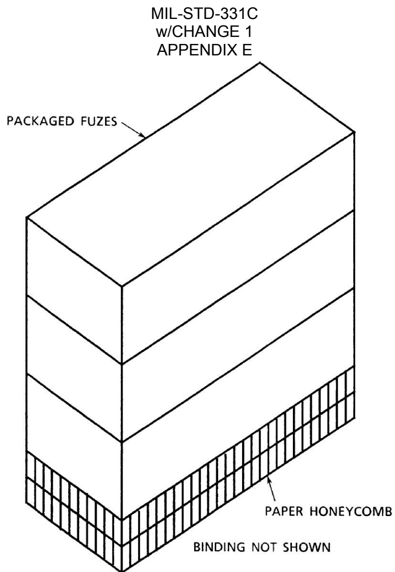
FIGURE E5-1. Example of Simulated Load
