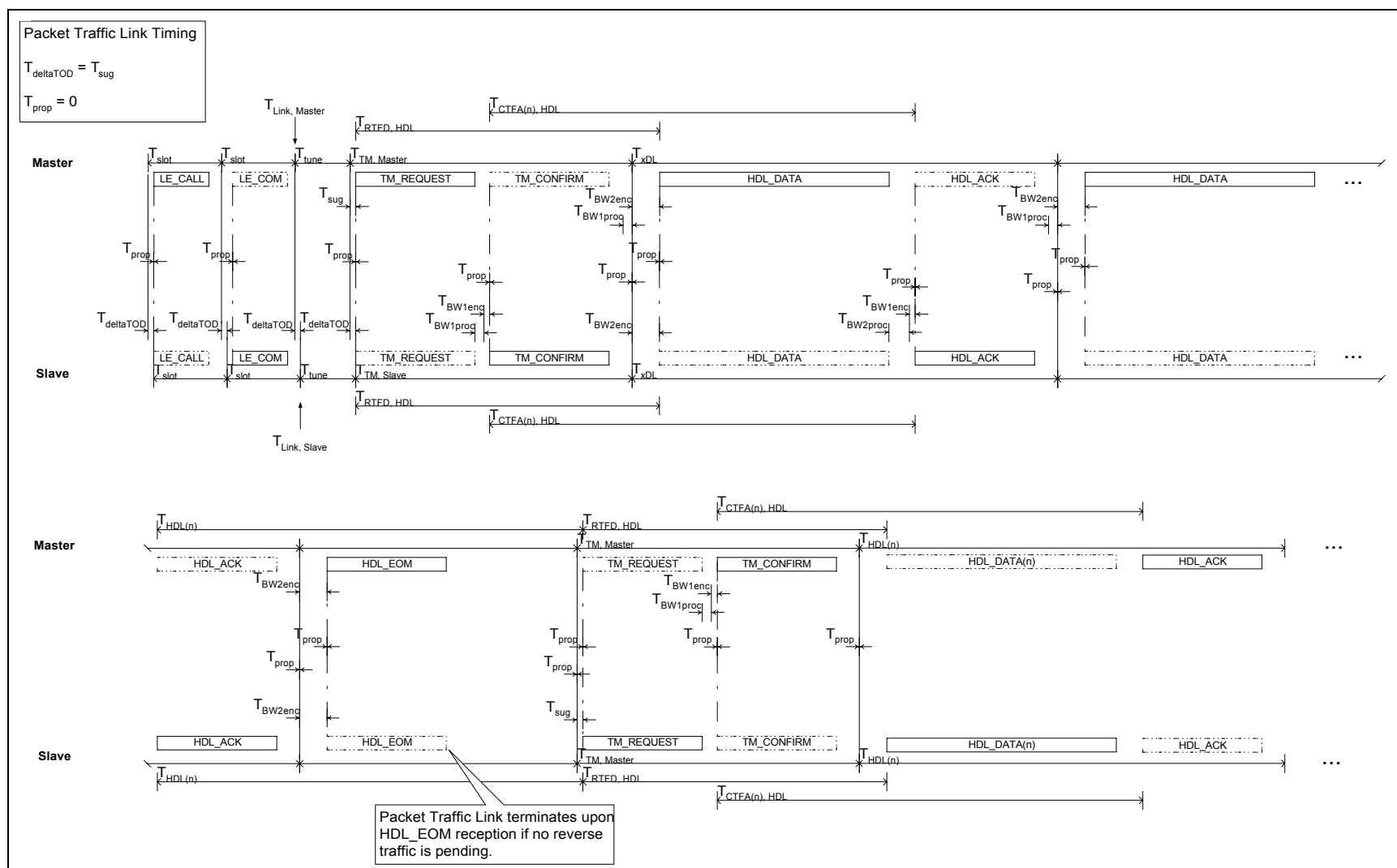
FIGURE C-30. Point-to-point packet link timing example for T_{\text{deltaTOD}} = T_{\text{sug}} , T_{\text{prop}} = 0 .
