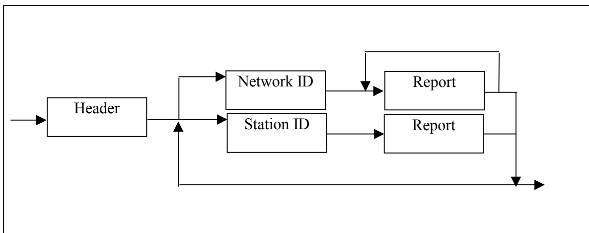
FIGURE D-6. Structure of CONEX message.
