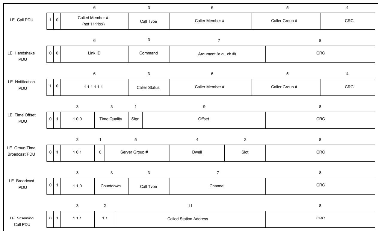
FIGURE C-17. 3G-ALE PDUs.
