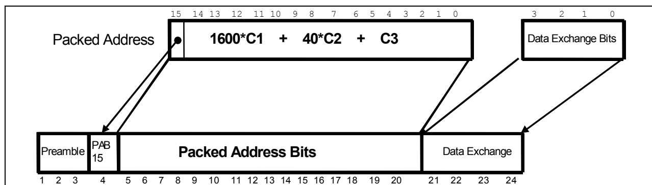
FIGURE A-52. AQC-ALE data exchange word.
