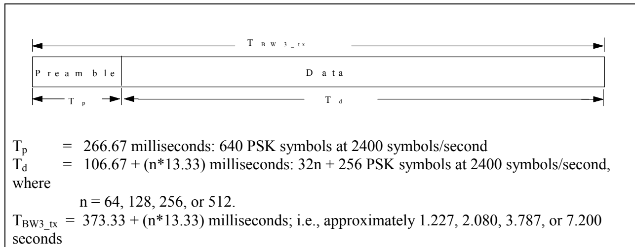
FIGURE C-13. BW3 timing.
