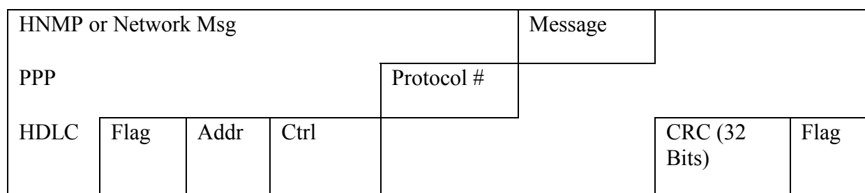
FIGURE D-16. SDLP frame structure.
