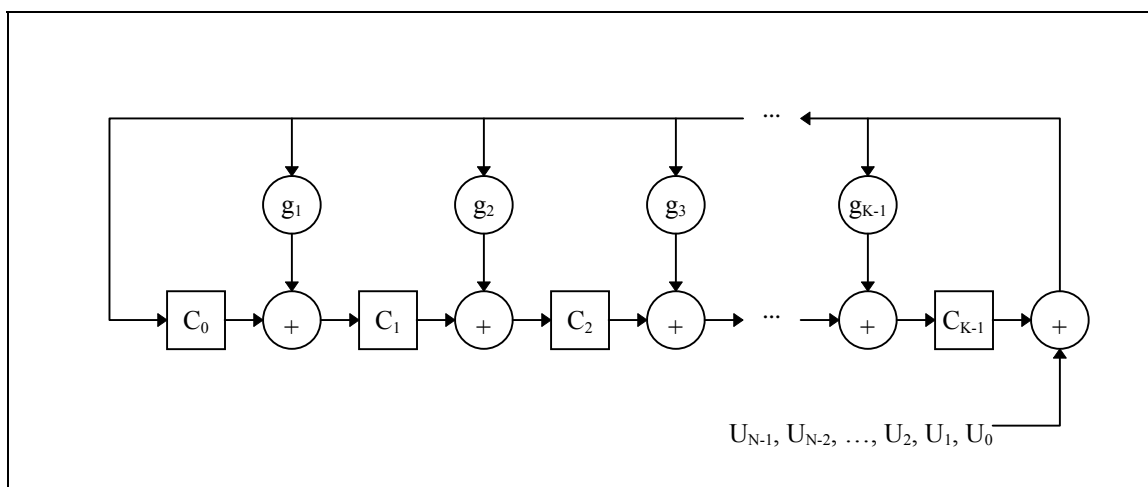
FIGURE C-4. CRC computation structure.
