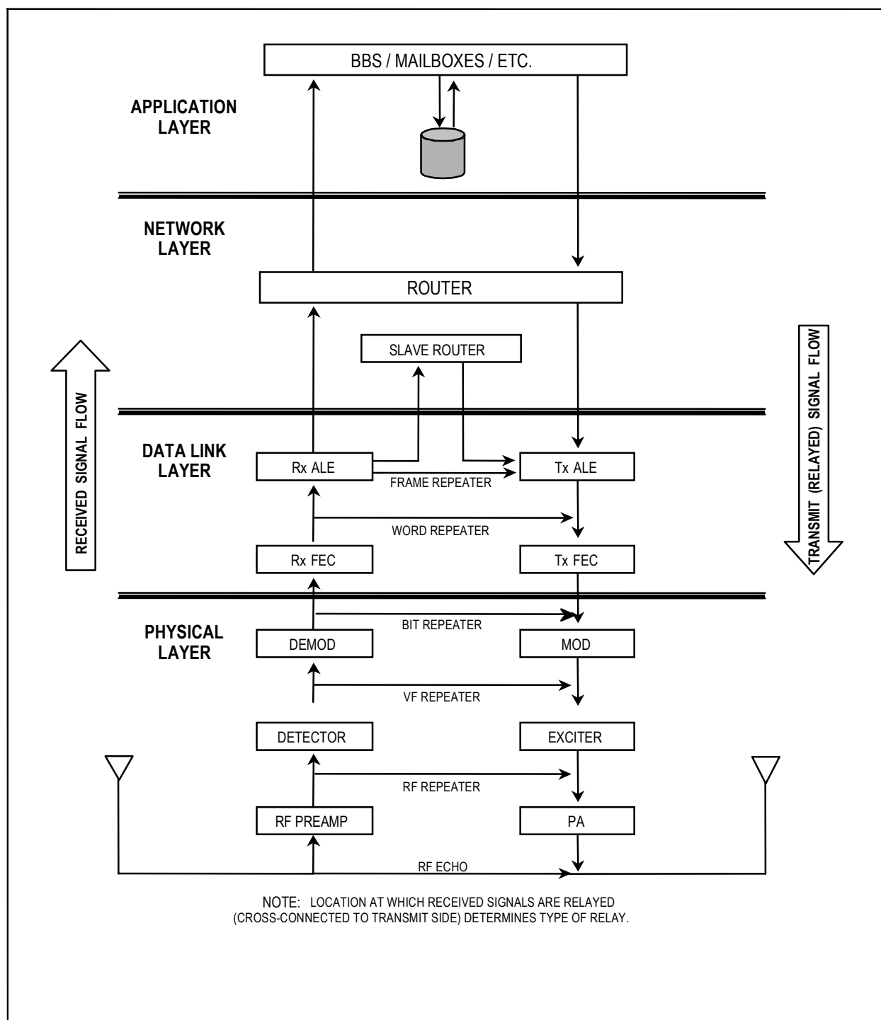
FIGURE 3. Relaying alternatives.
