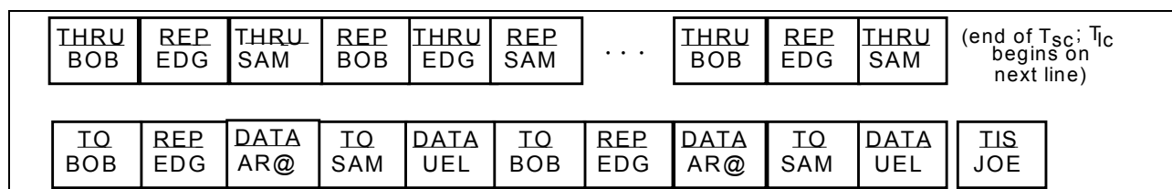
FIGURE A-35. Group call.
