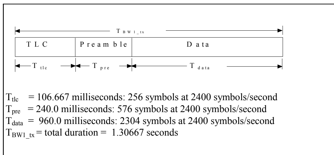
FIGURE C-7. BW1 timing.
