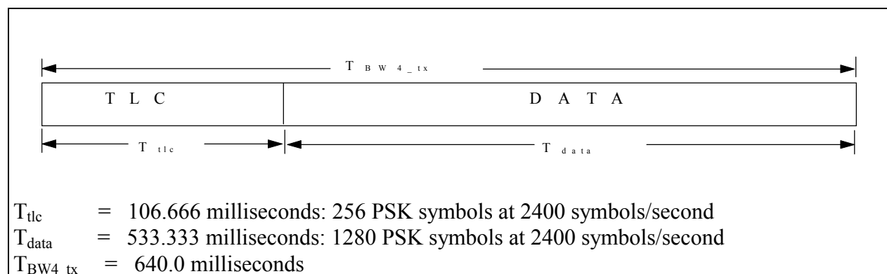
FIGURE C-15. BW4 timing.
