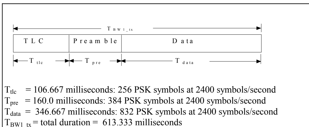
FIGURE C-5. BW0 timing.
