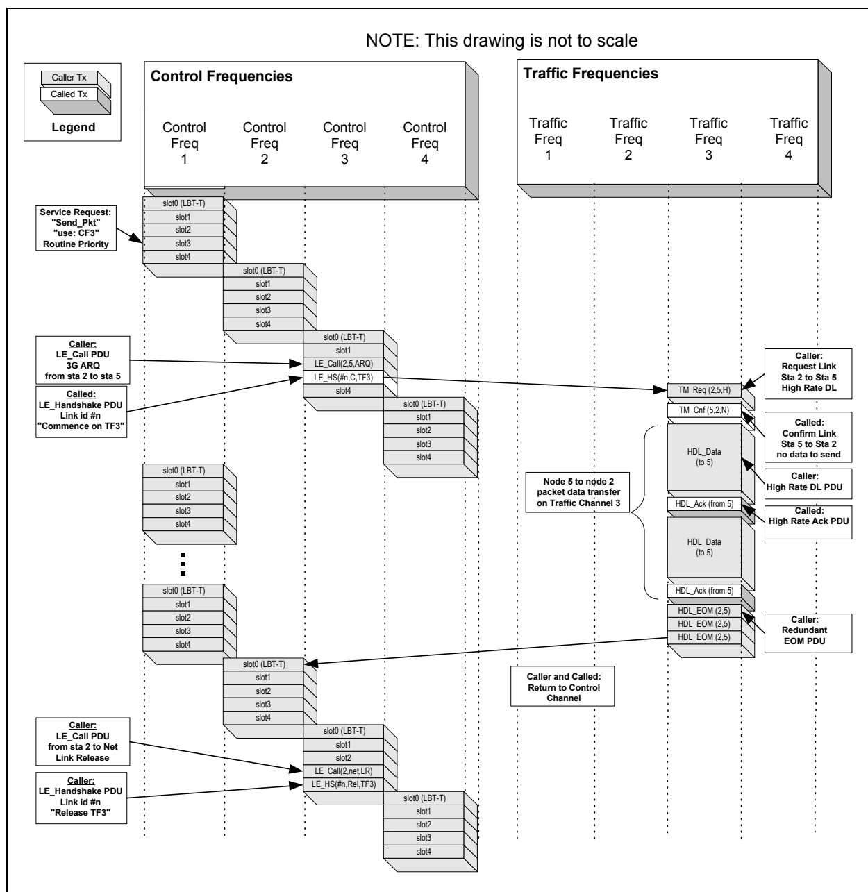
FIGURE C-45. Packet linking and traffic exchange: on-air signalling overview.
