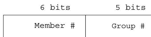
FIGURE C-3. Synchronous mode address structure.
