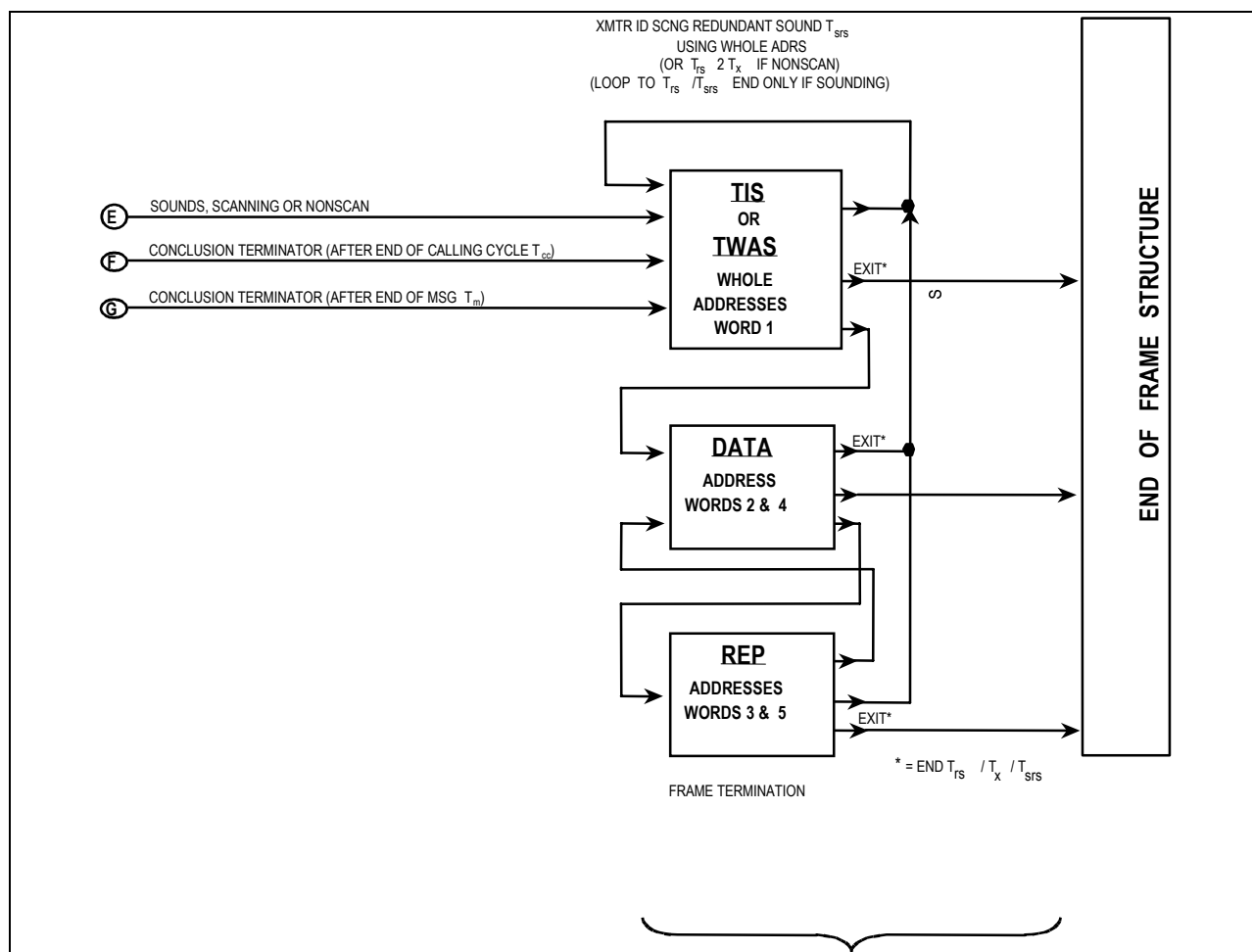
FIGURE A-20. Valid word sequence (conclusion section).
