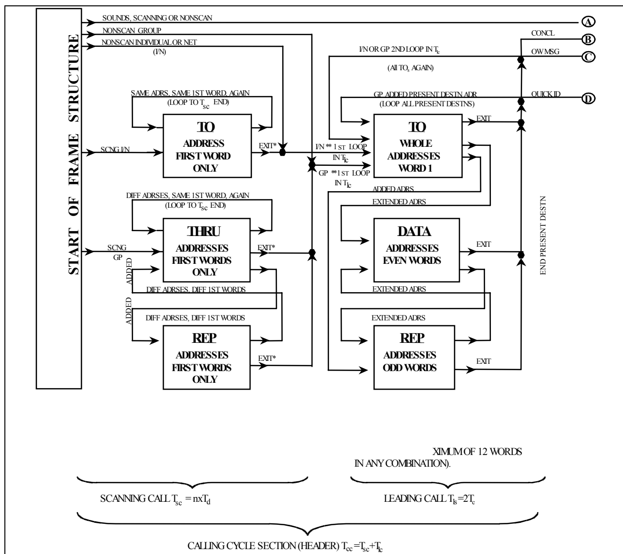
FIGURE A-18. Valid word sequence (calling cycle section).
