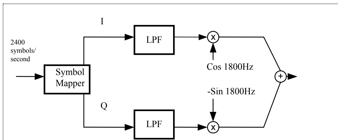
FIGURE C-16. Carrier modulation.
