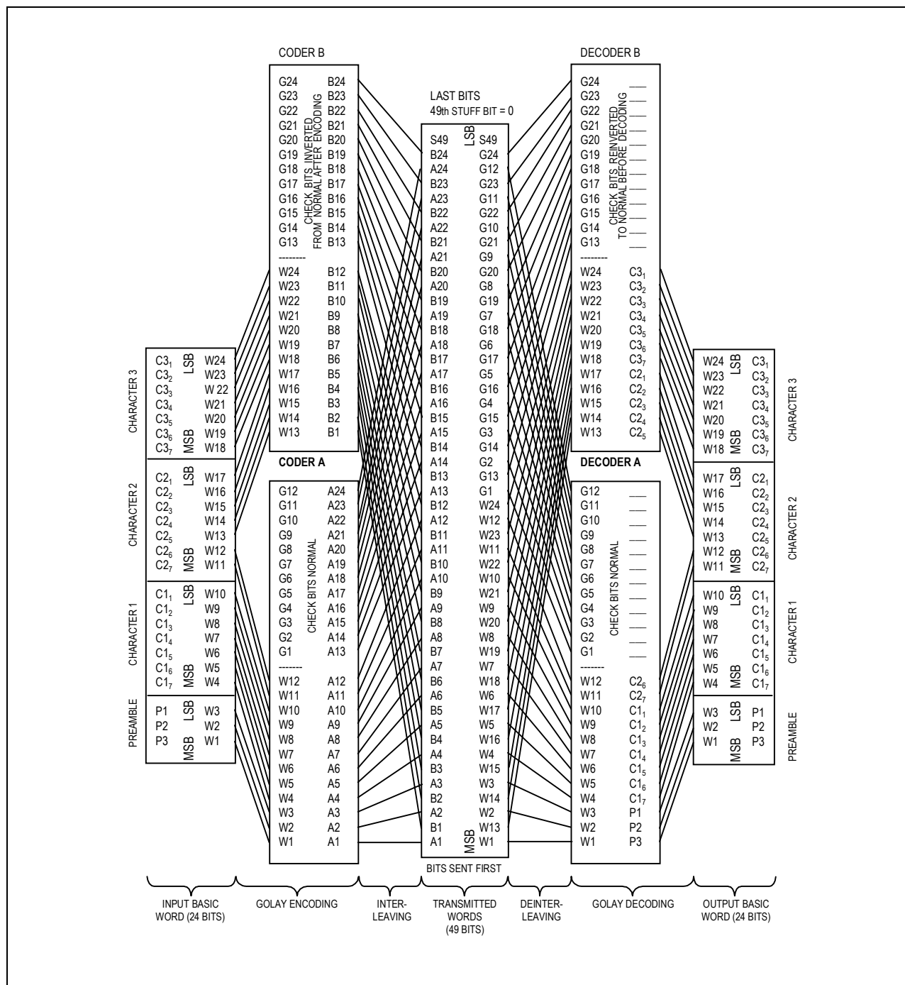
FIGURE A-10. Word bit coding and interleaving.
