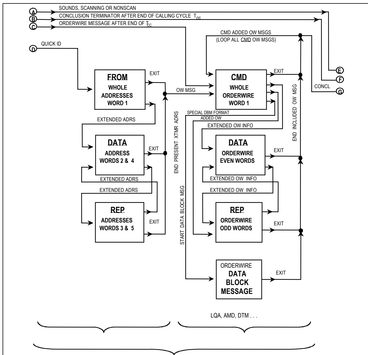
FIGURE A-19. Valid word sequence (message section).
