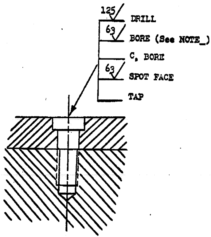
FIGURE 13. Symbol Placement.
