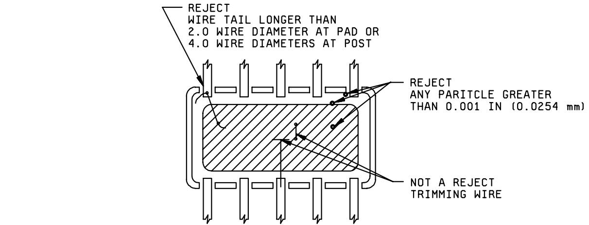
(a) PARTICLE LOCATIONS, PIGTAILS, AND TRIMMING WIRES
