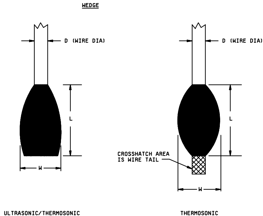
FIGURE 17-4a. Bond Dimensions .
