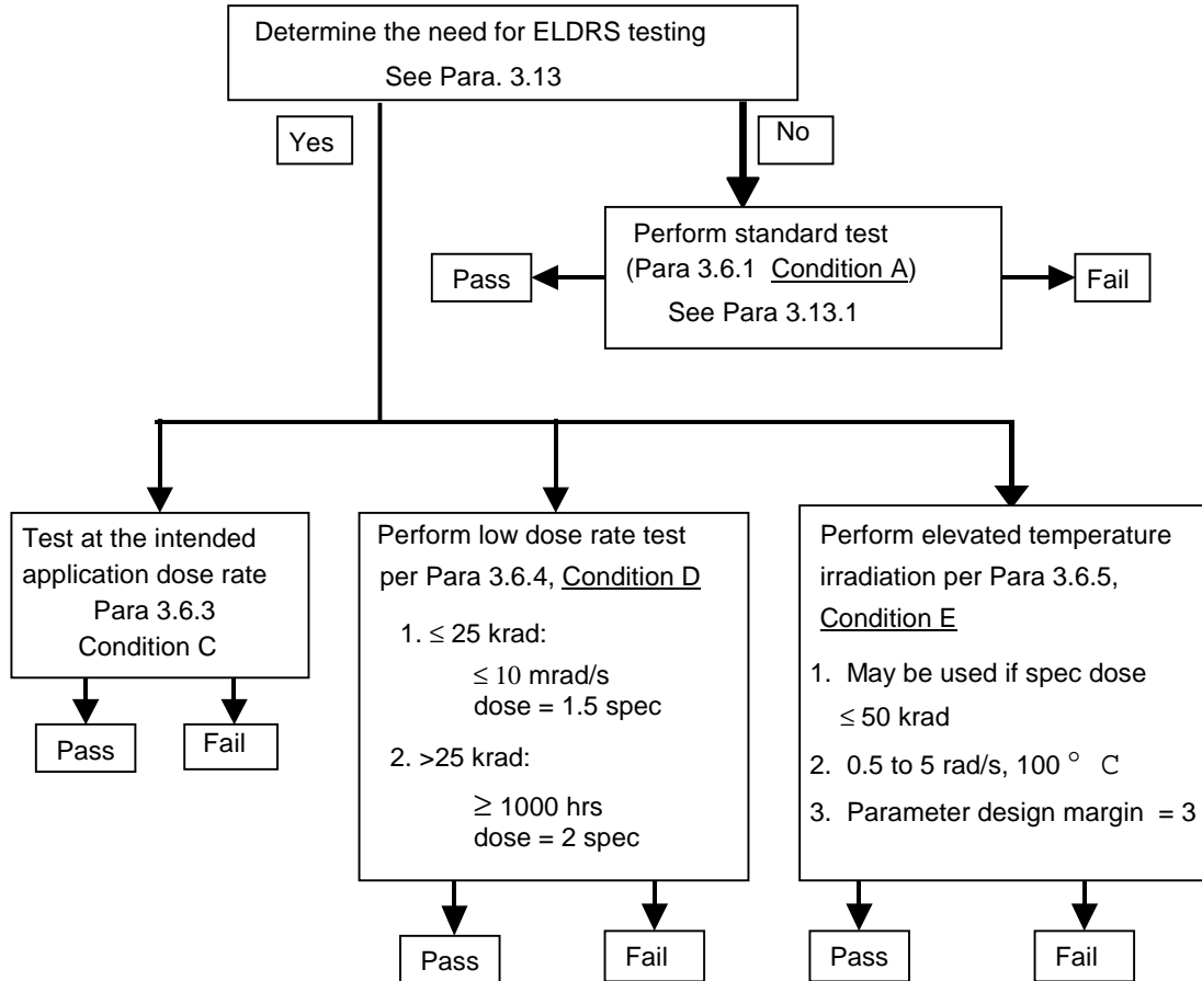
Figure 1019-2. Flow diagram for ionizing radiation test procedure for bipolar (or BiCMOS) linear or mixed-signal circuits
