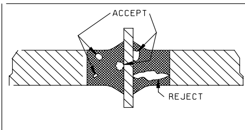
FIGURE 2009-7b. Subsurface bubbles.
