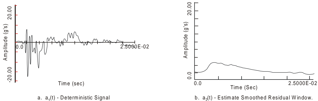
FIGURE 519.5B-10. Non-stationary model deterministic functions.
