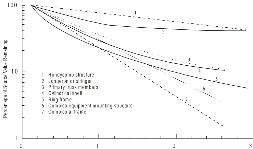
FIGURE 517-12. Peak pyroshock response vs distance from pyrotechnic source.
