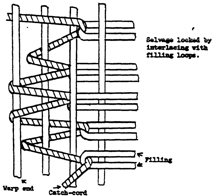
FIGURE 2. Catch-cord diagram.
