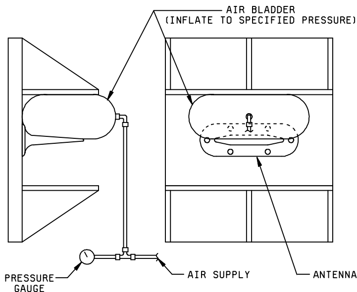
FIGURE 3. Static load test .
