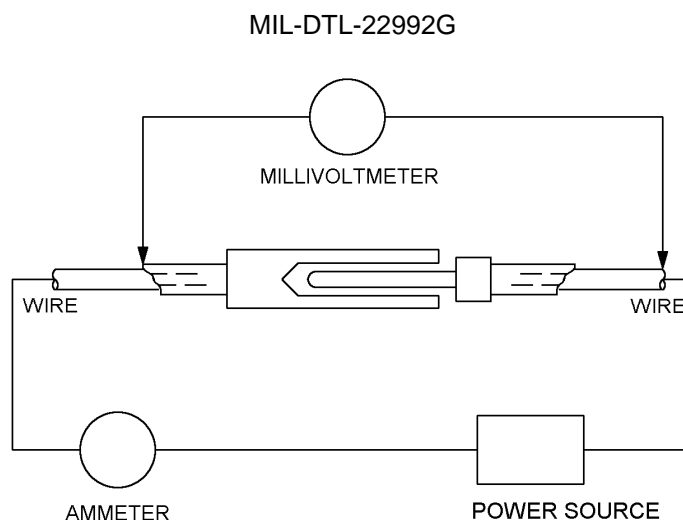
FIGURE 2. Wiring diagram for contact resistance test.
