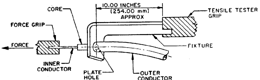
FIGURE 4. Typical test fixture for use with Semi-rigid cables.
