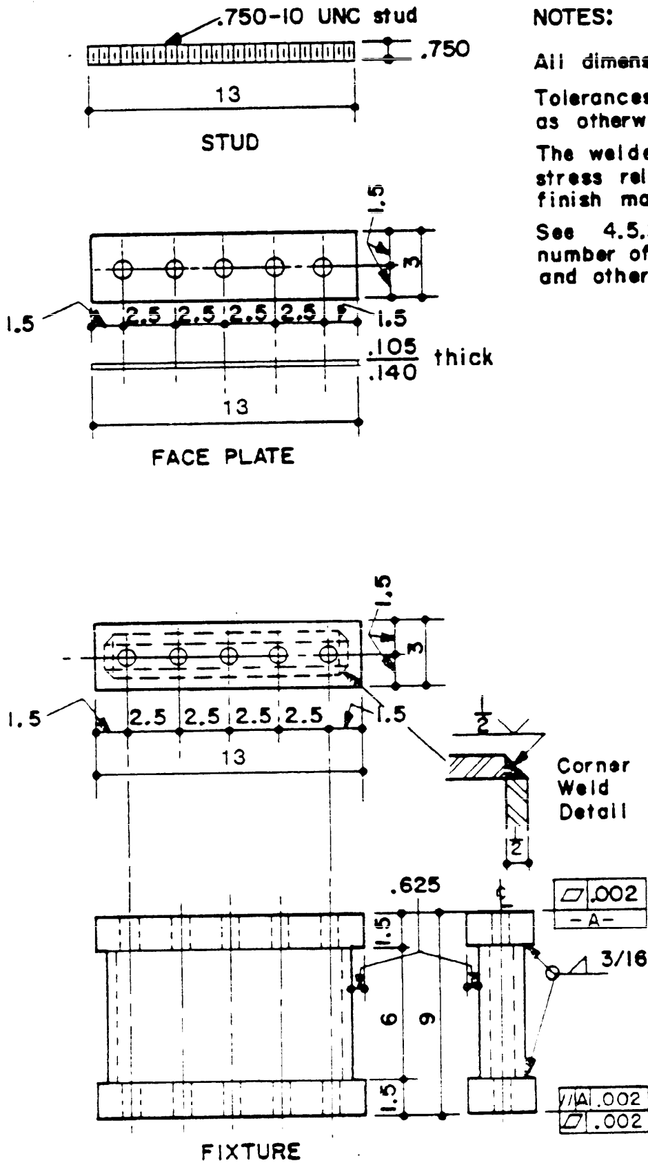
FIGURE 1. Test fixture.
