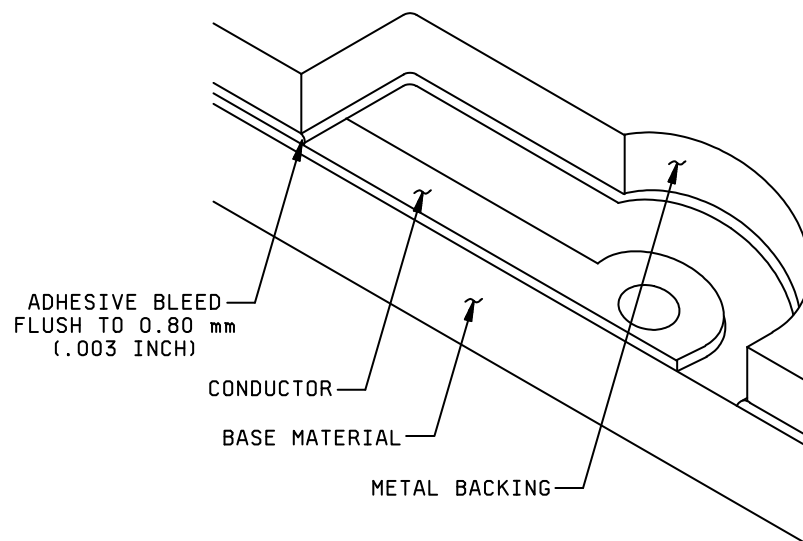
FIGURE 1. Adhesive bleed near conductor.
