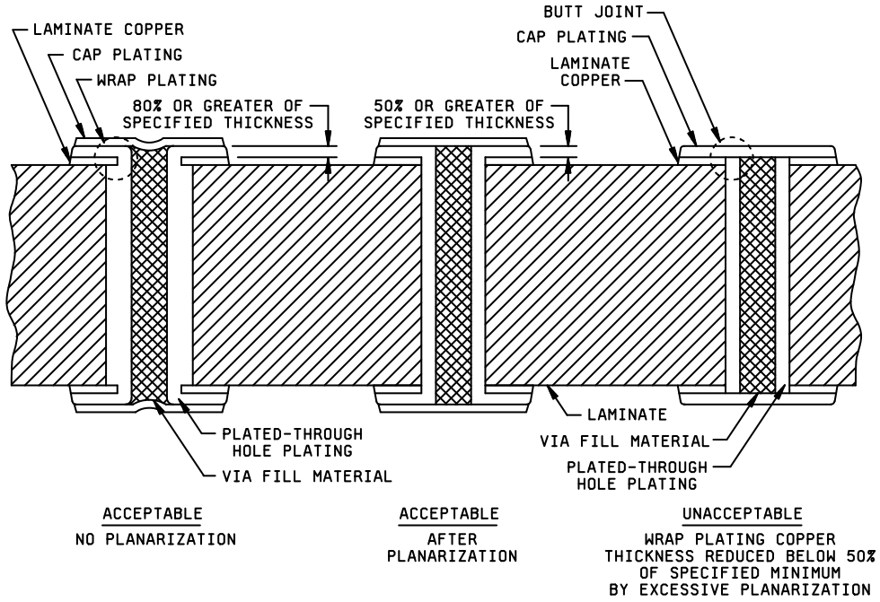
FIGURE 5. Plated-through hole wrap plating (continuous hole-knee-surface copper plating).
