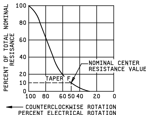
FIGURE 4. Counterclockwise taper.
