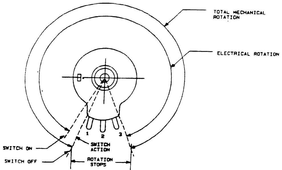
FIGURE 2. Definition of rotation (shaft end view).
