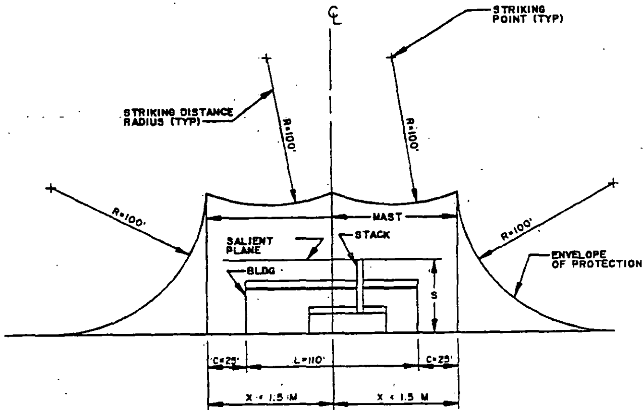
ELEV. SIDE VIEW
