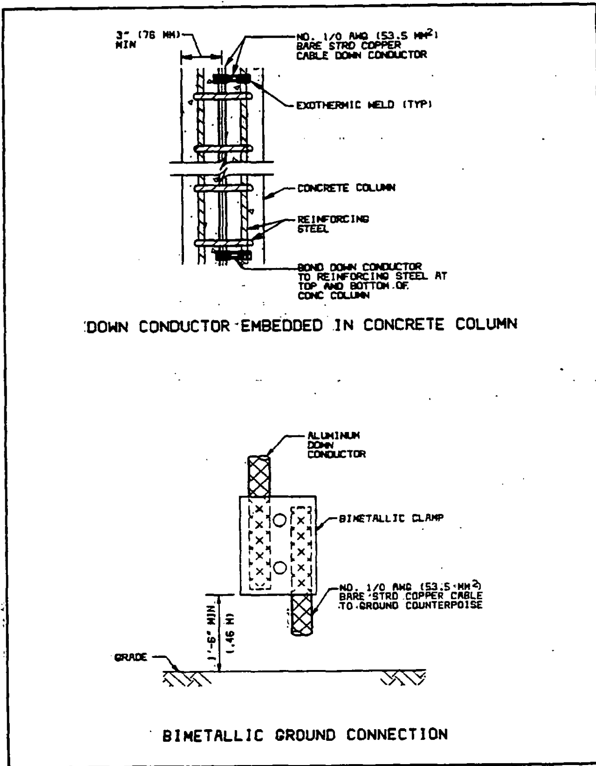
Figure 7 Other Grounding Details
