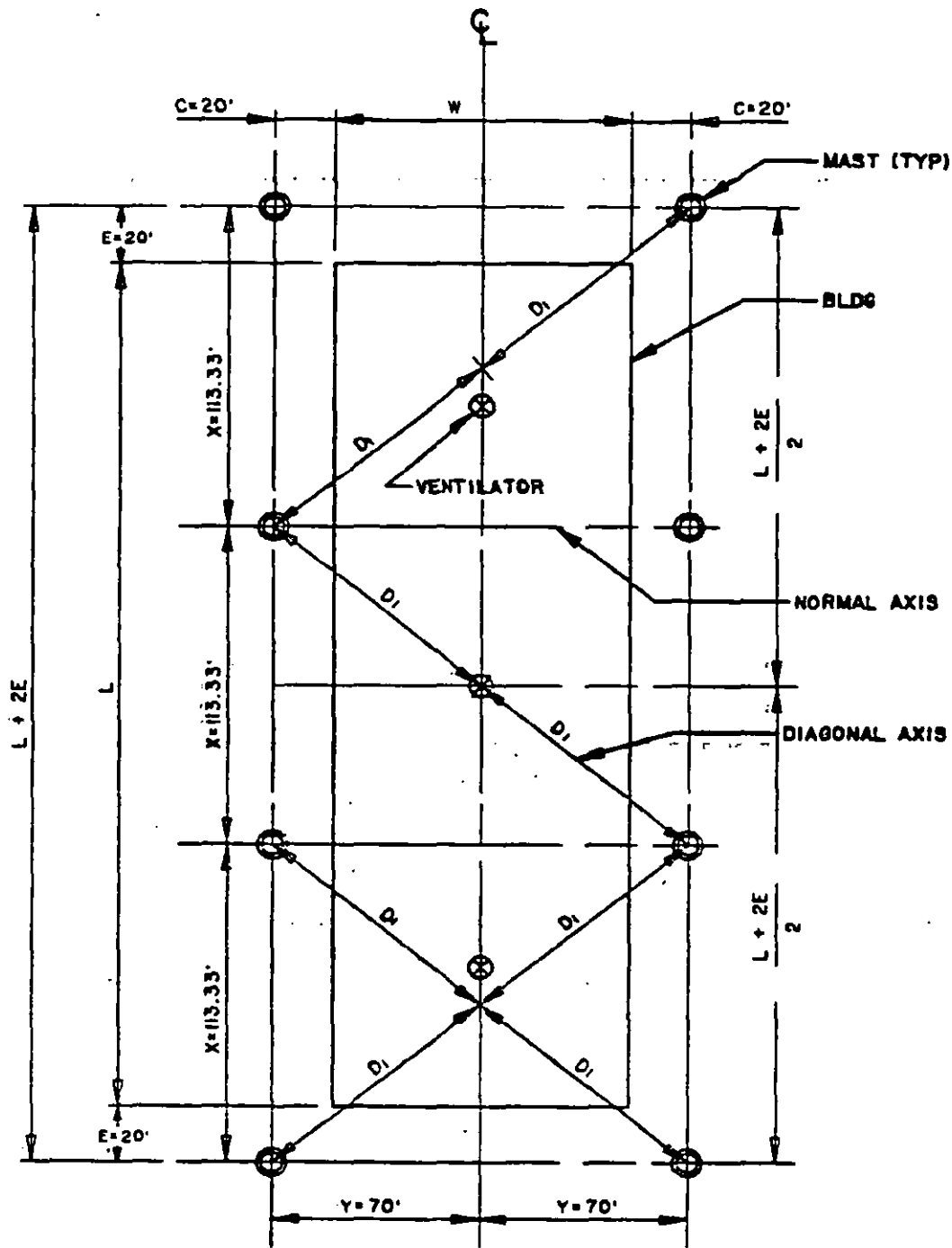
PLAN
