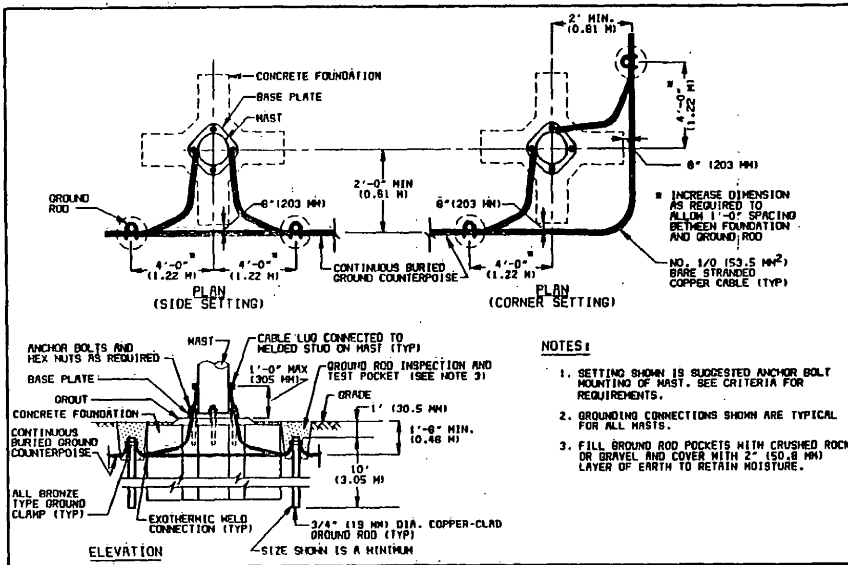
Lightning Mast Ground Connection Details Figure 2
