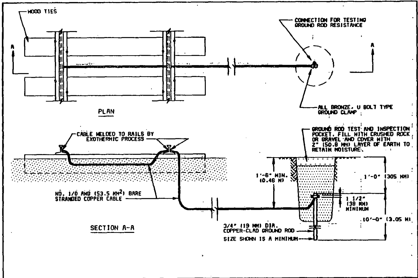
Figure 4 Bonding and Grounding of Railroad Track
