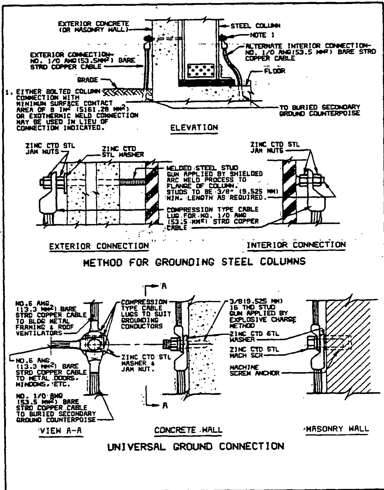
Figure 5 Concrete and Steel Ground Connections for Secondary System
