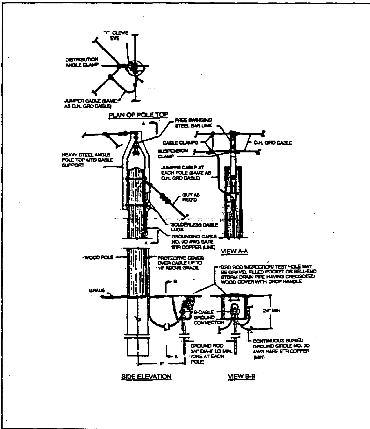
A-12 (PAGE 3 of 3) PRIMARY LIGHTNING PROTECTION DESIGN FOR ORDNANCE HANDLING FACILITIES
