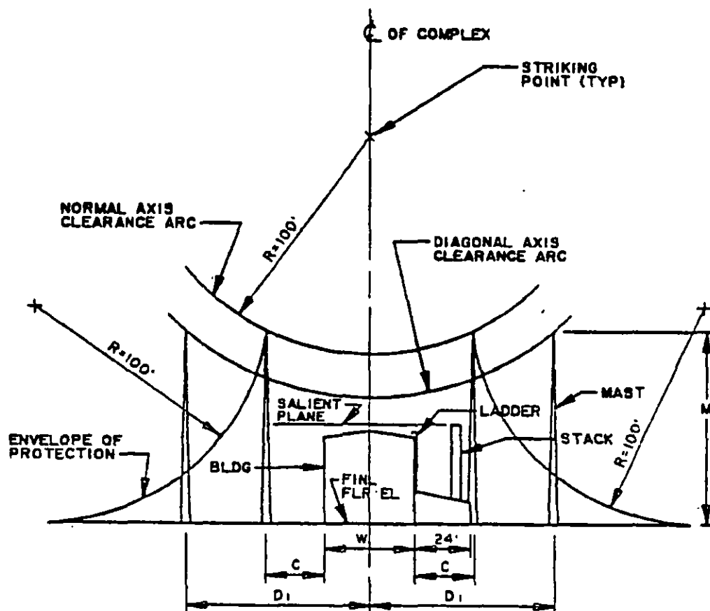
CLEARANCE ARC DIAGRAM
