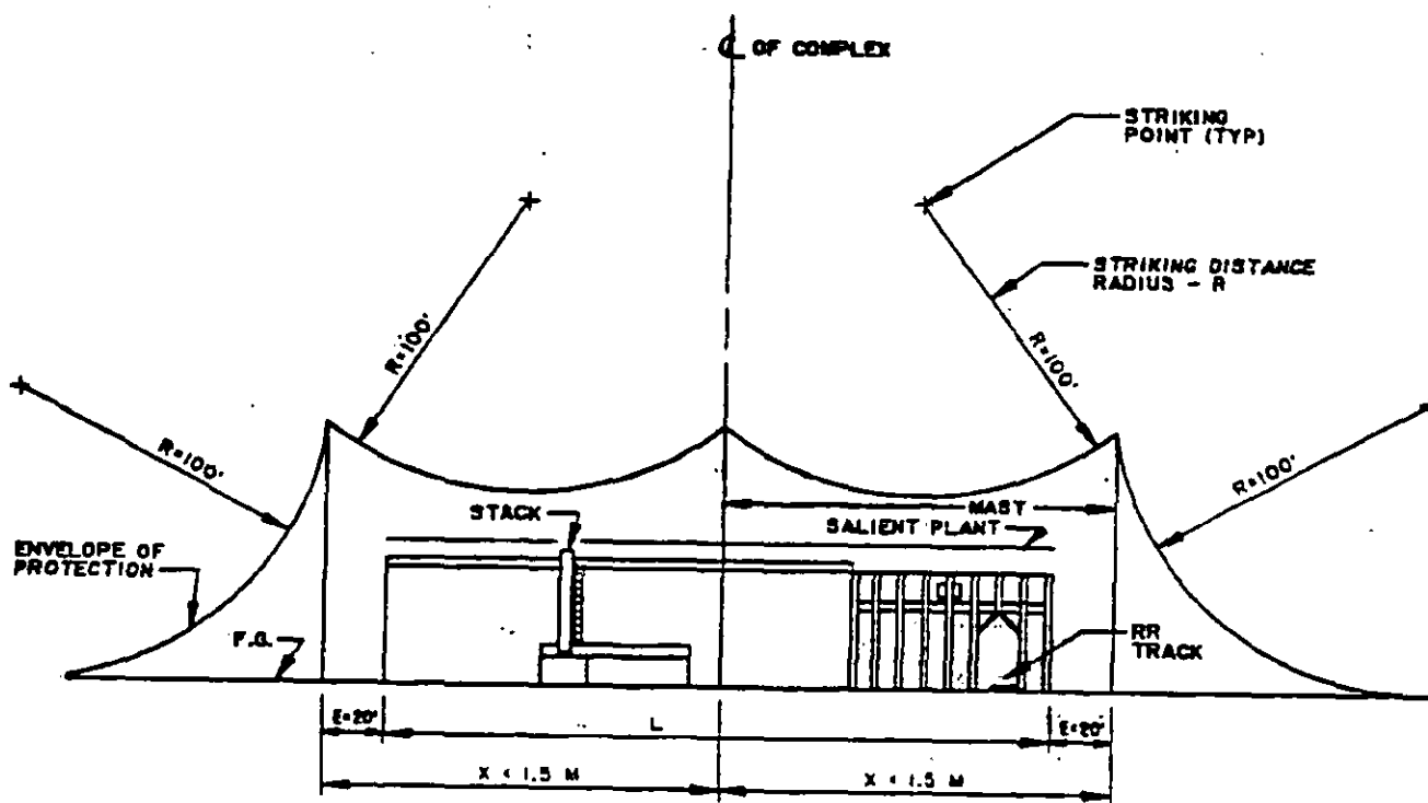
ELEV. SIDE VIEW
