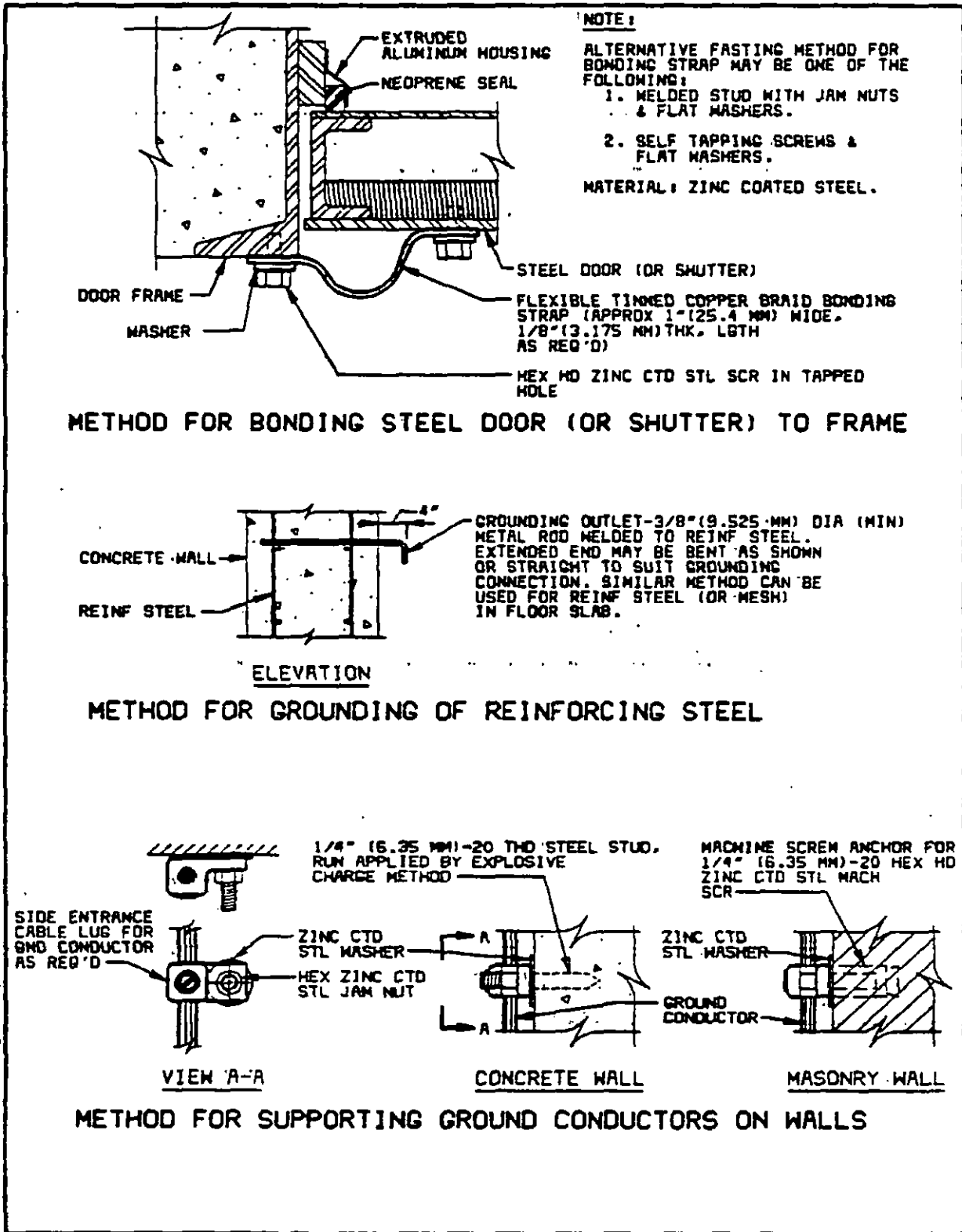
Figure 6 Other Grounding Details for Secondary System
