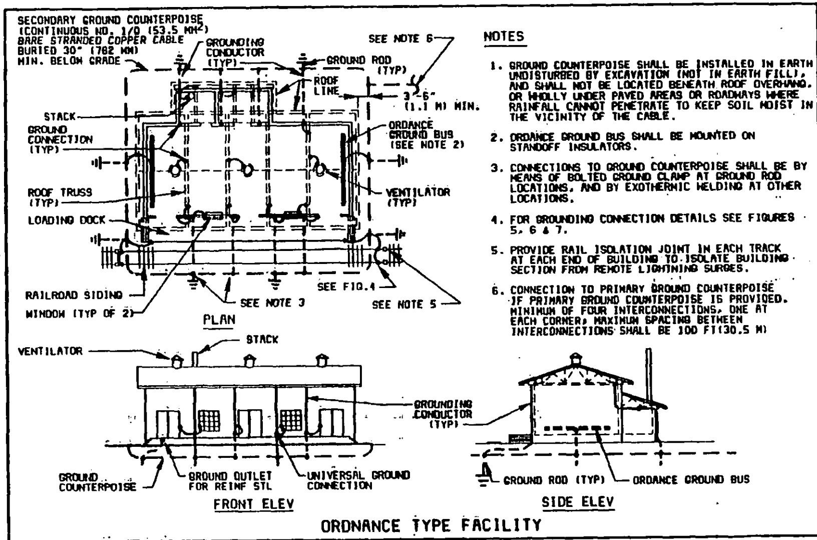
Figure 3 Secondary Lightning Protection or Grounding System
