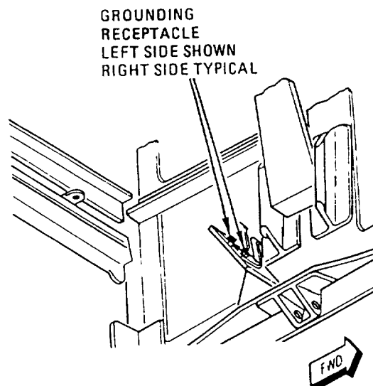
MAIN LANDING GEAR WHEELWELL
