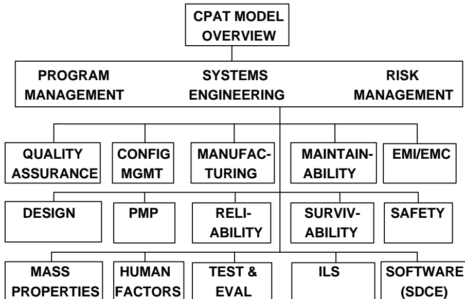
FIGURE 1. CPAT Model.
