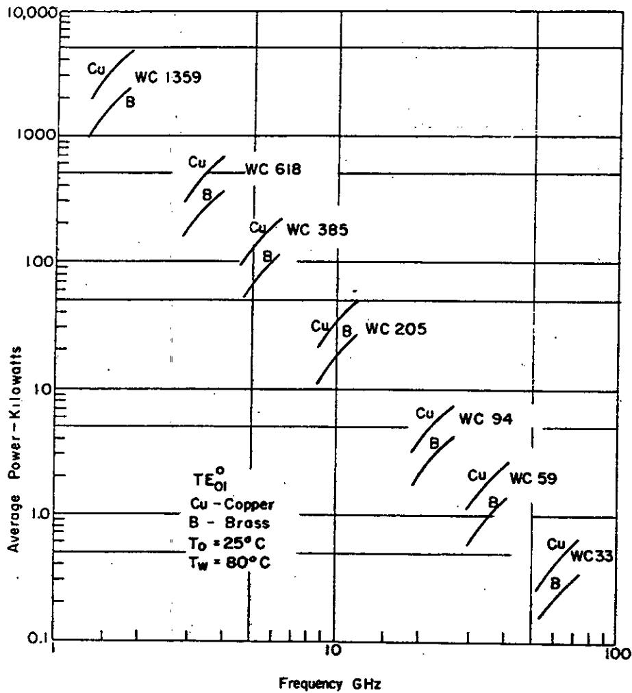
FIGURE 6.15. Average power capability of circular waveguides, TE_{01} mode, as a function of frequency.
