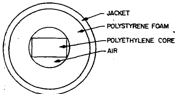
FIGURE 6.21. Typical dielectric waveguide.
