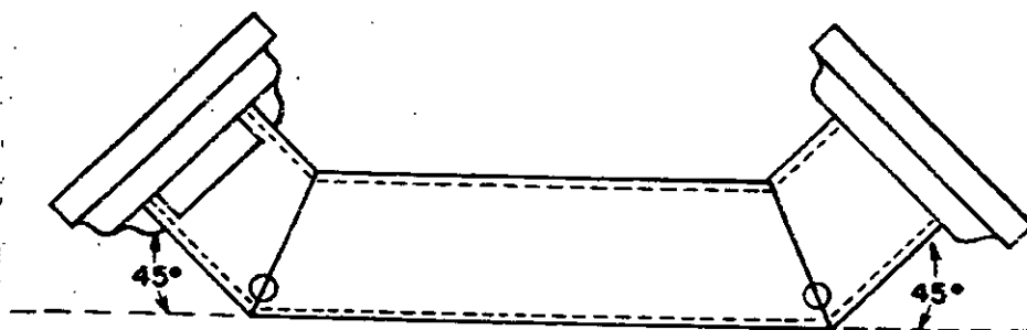
TYPICAL 90° CORNER UTILIZING THREE SECTIONS OF WAVEGUIDE
