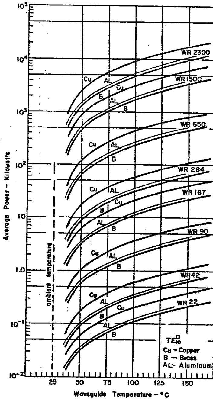
FIGURE 6.9. Average power capability of standard waveguides as a function of waveguide temperature.
