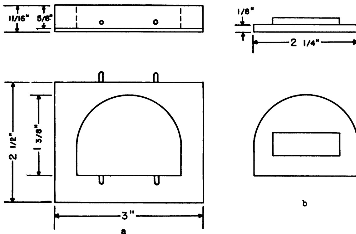
FIGURE 3810B - Cuvette used with Gardner photometric unit.
