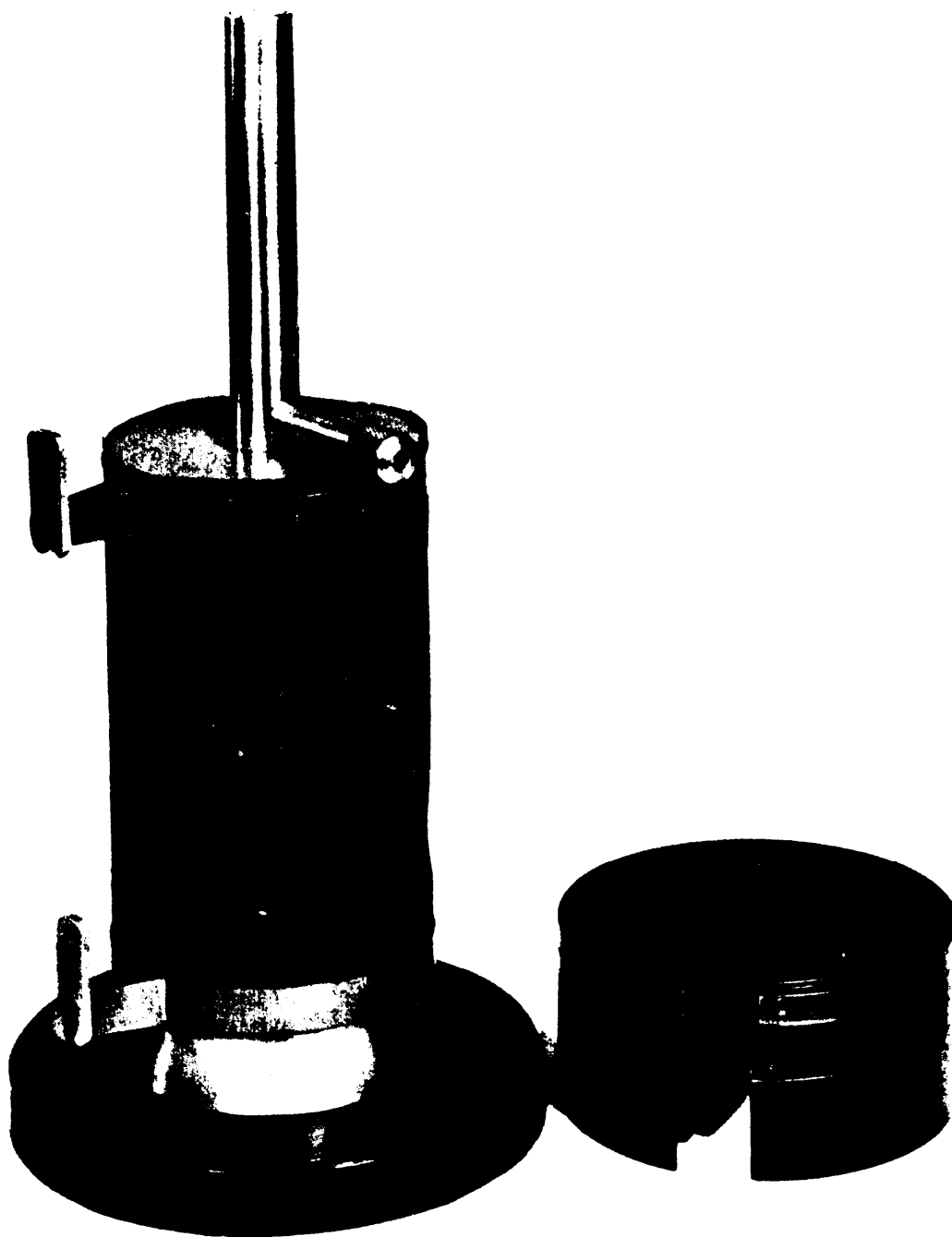
FIGURE 5214A - AATCC Wrinkle Tester
