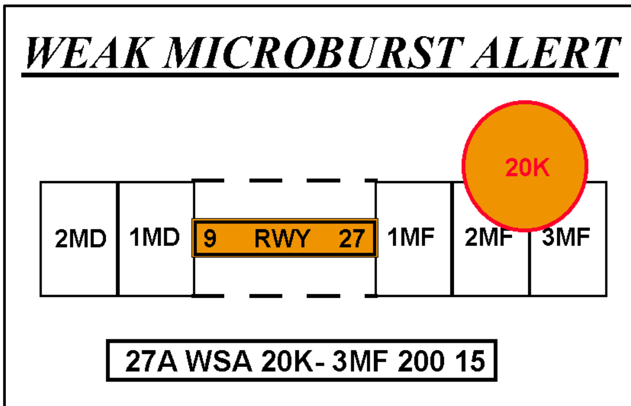
FIG 7-1-20 Weak Microburst Alert
