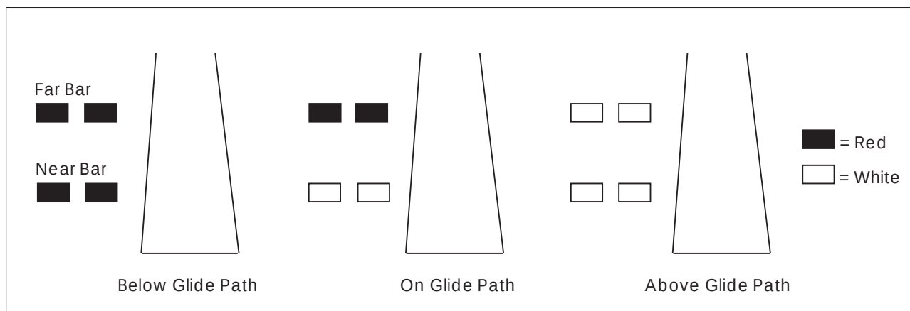
FIG 2-1-2 2-Bar VASI
