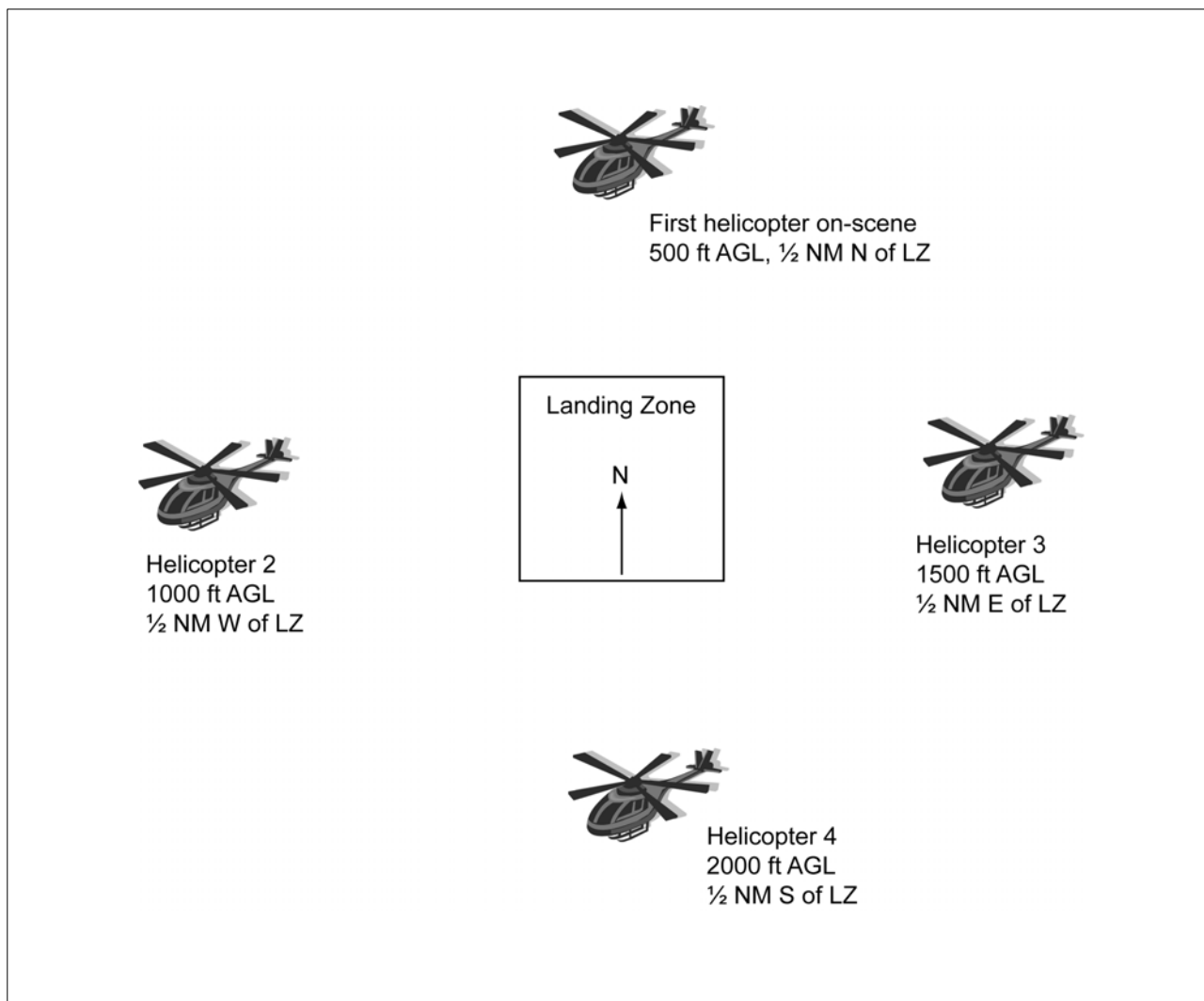
FIG 10-2-9 EMS Multiple Helicopter LZ/Heliport Operation
