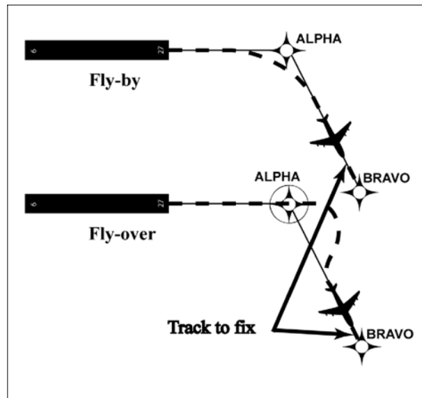
FIG 1-2-2 Track to Fix Leg Type
