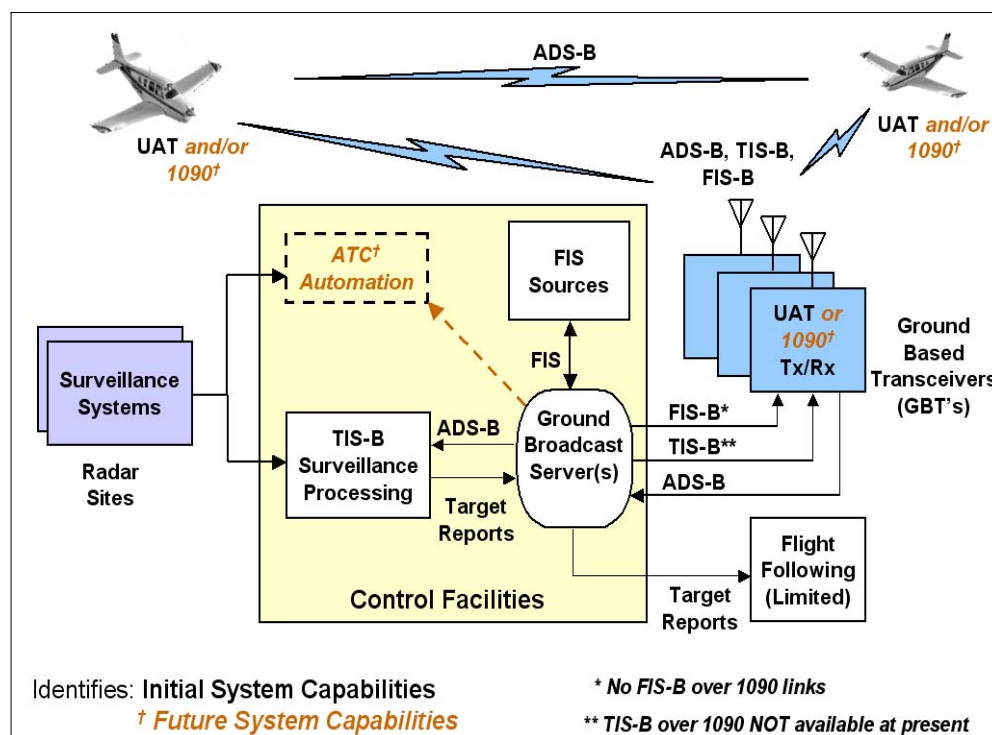
FIG 4-5-7 ADS-B, TIS-B, and FIS-B: Broadcast Services Architecture
