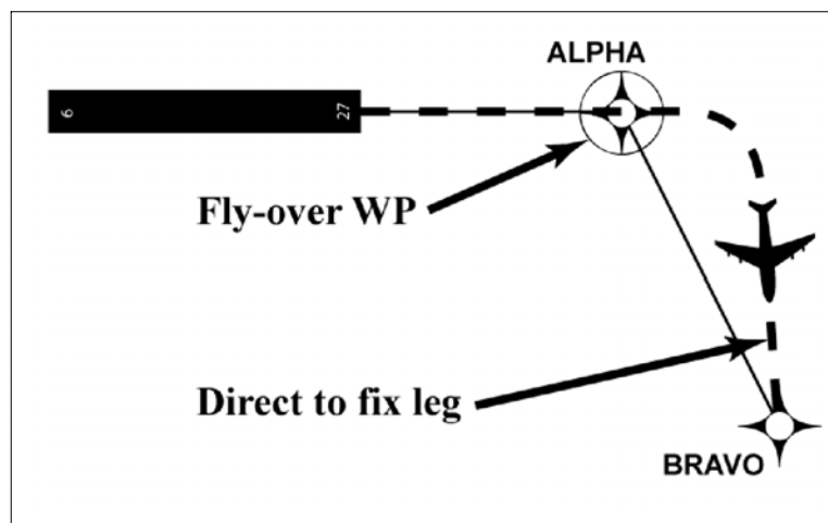
FIG 1-2-3 Direct to Fix Leg Type
