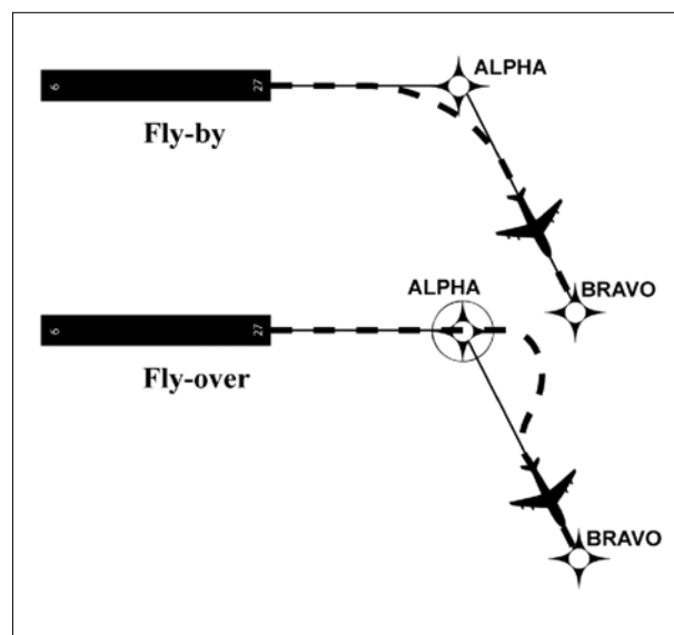
FIG 1-2-1 Fly-by and Fly-over Waypoints
