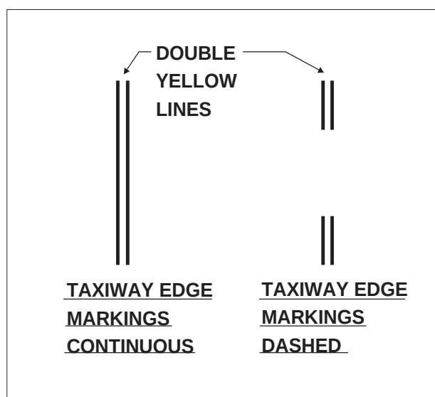
FIG 2-3-9 Dashed Markings
