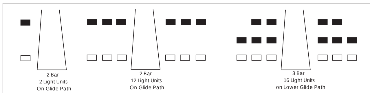
FIG 2-1-4 VASI Variations
