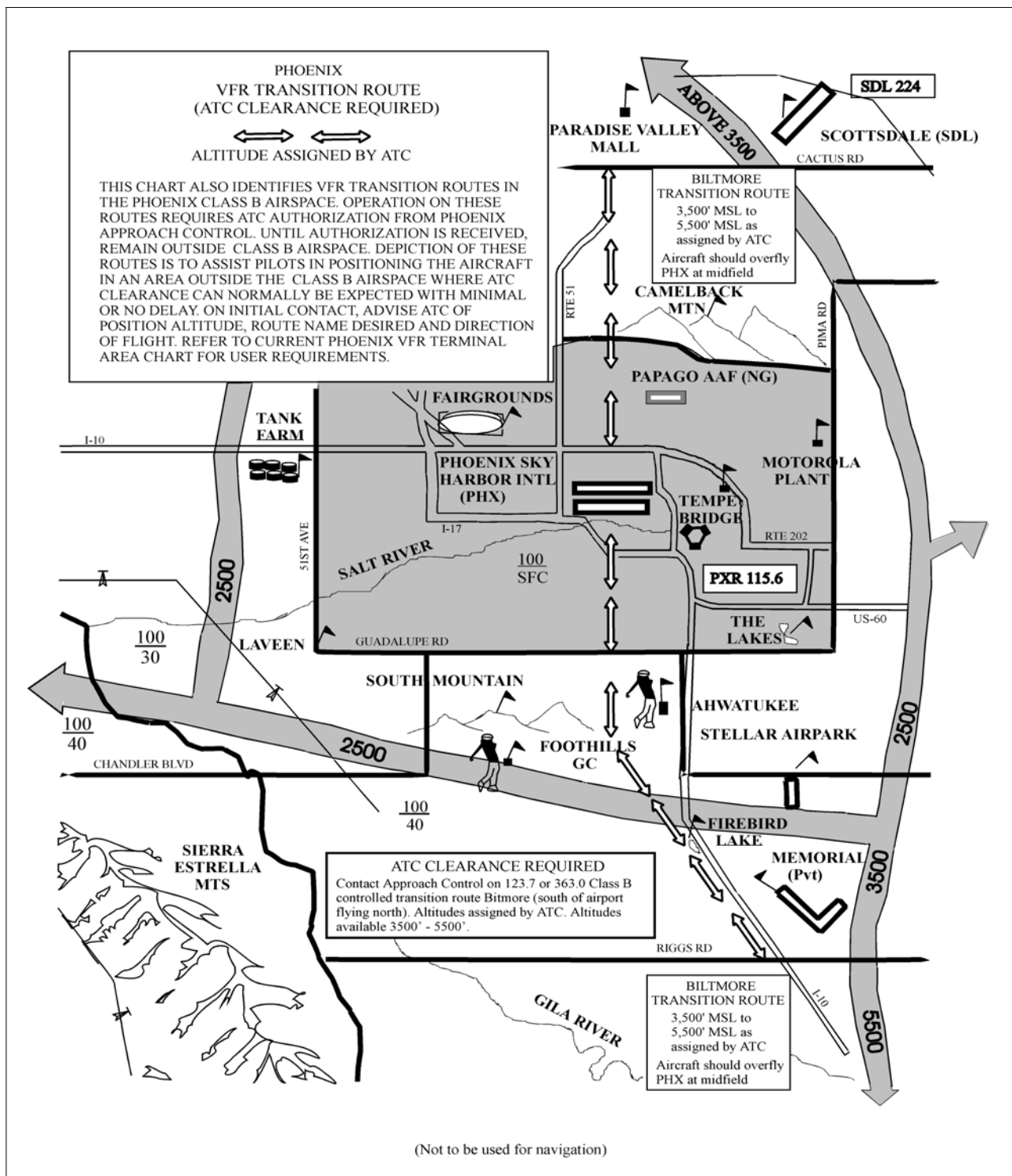
FIG 3-5-3 VFR Transition Route
