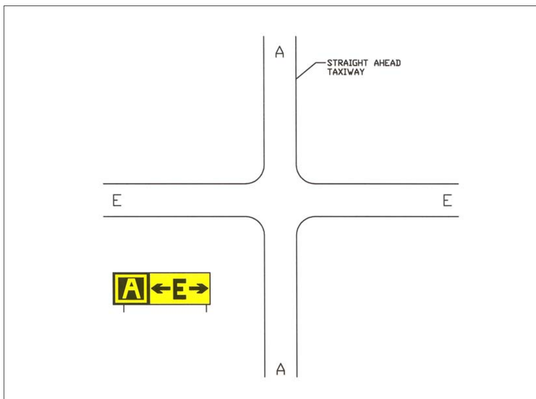
FIG 2-3-37 Direction Sign Array for Simple Intersection
