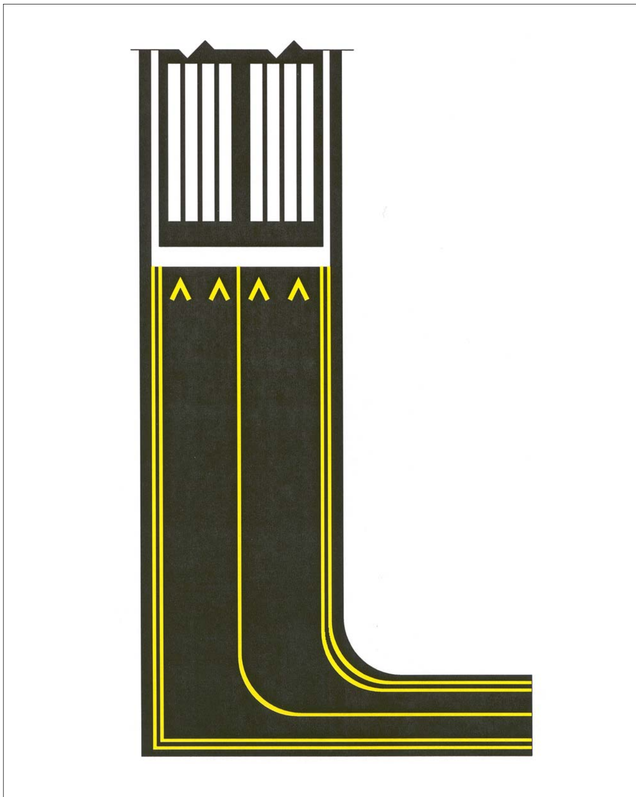
FIG 2-3-3 Relocation of a Threshold with Markings for Taxiway Aligned with Runway
