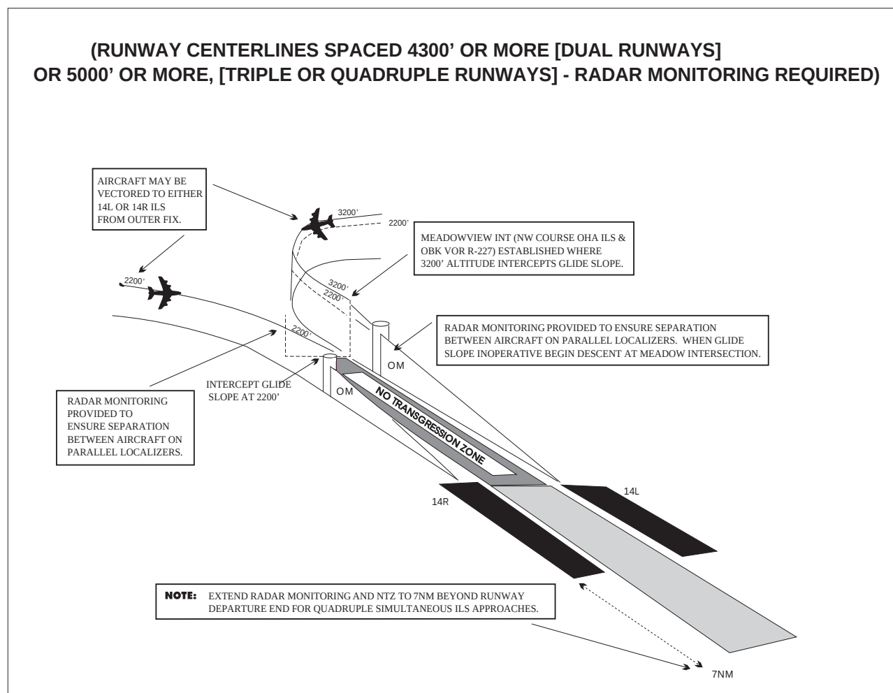
FIG 5-4-20 Simultaneous Parallel ILS Approaches
