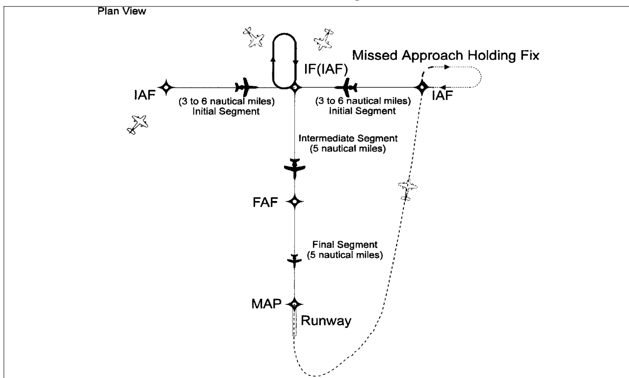
FIG 5-4-2 Basic “T” Design
