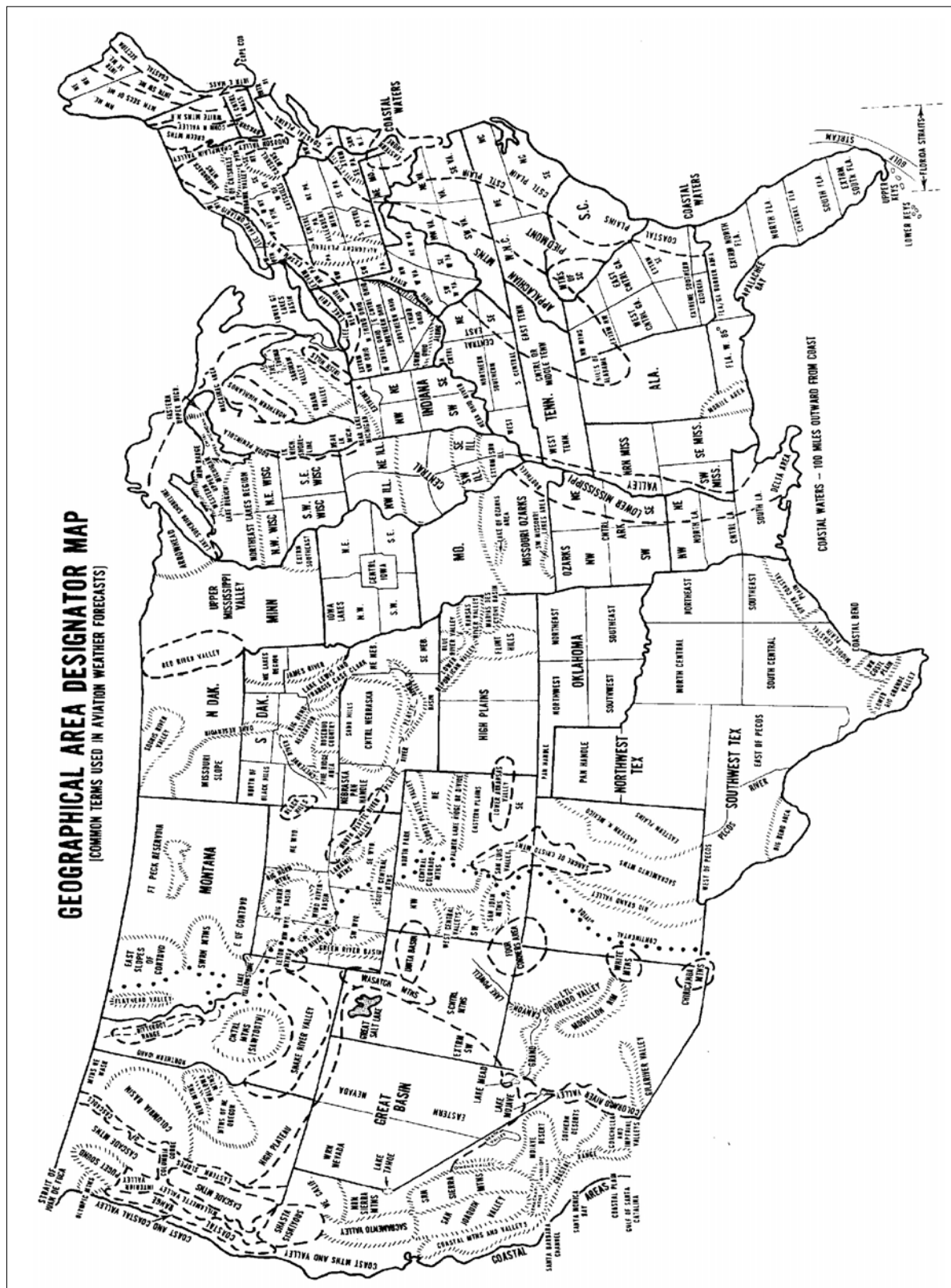
FIG 7-1-4 Geographical Areas and Terrain Features
