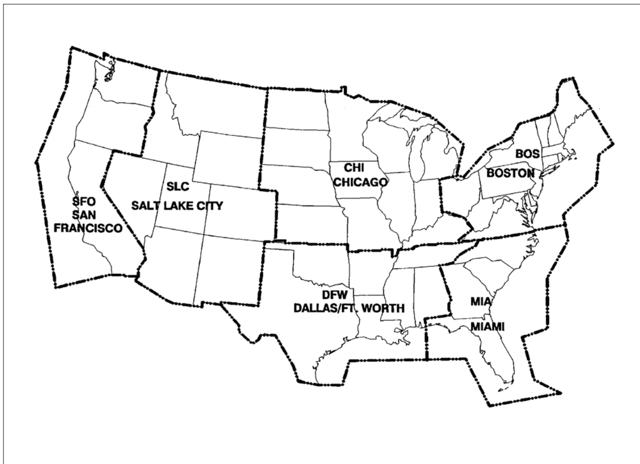
FIG 7-1-5 Aviation Area Forecasts FA Locations – Contiguous United States
