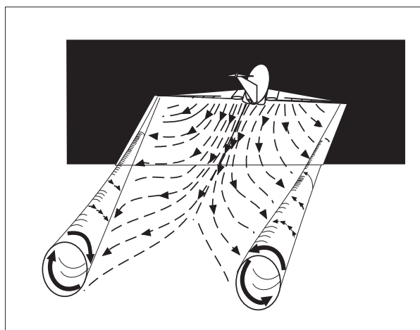
FIG 7-3-1 Wake Vortex Generation
