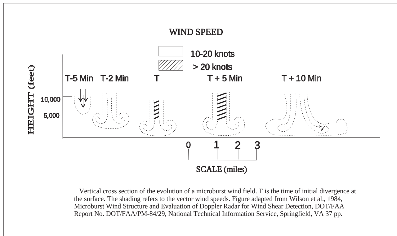
FIG 7-1-14 Evolution of a Microburst
