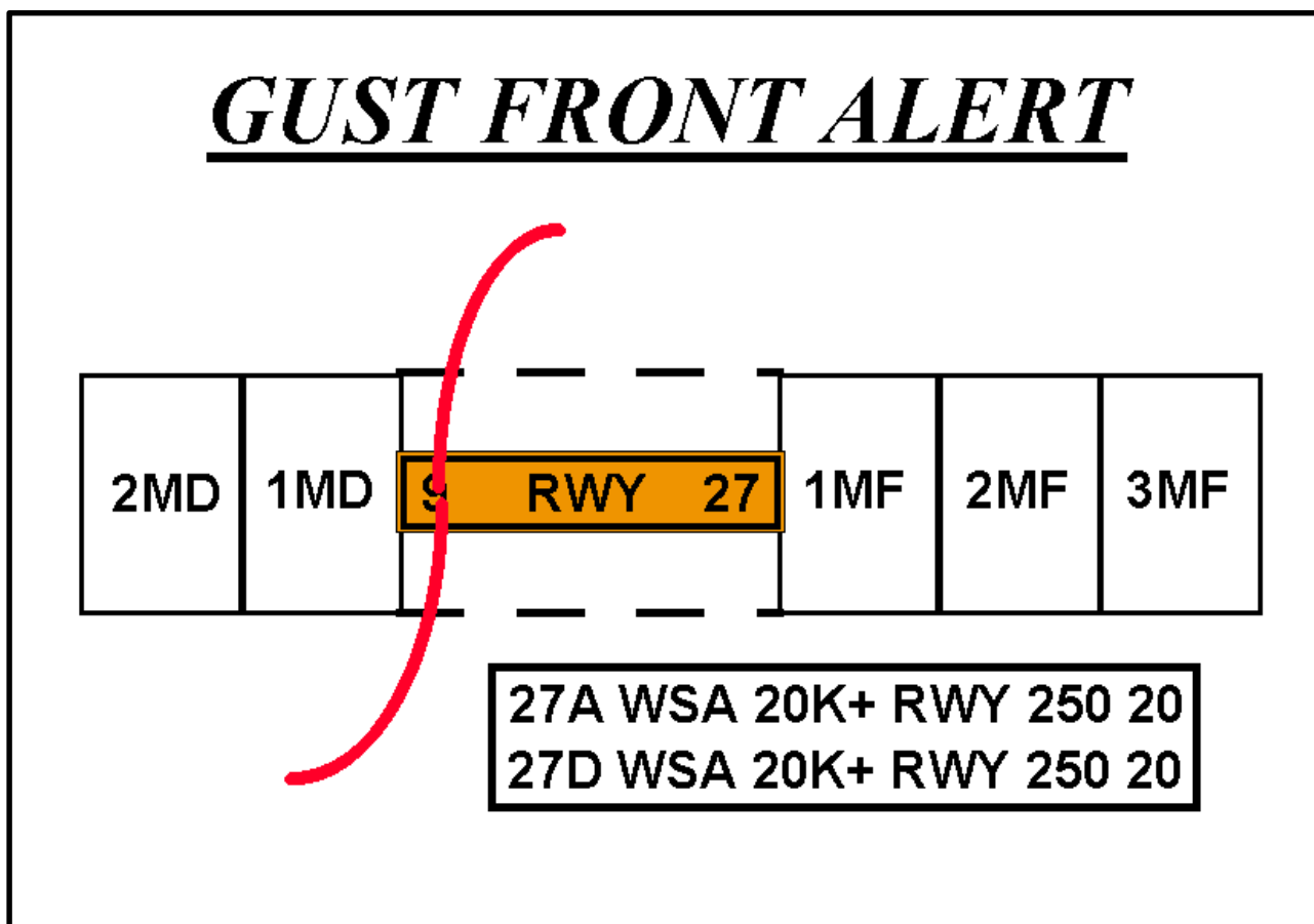
FIG 7-1-21 Gust Front Alert
