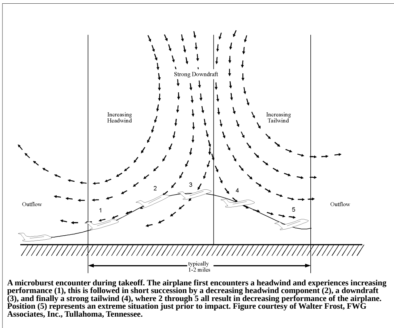
FIG 7-1-15 Microburst Encounter During Takeoff
