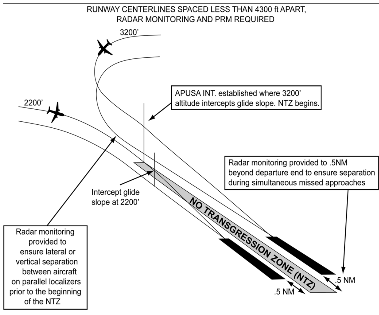
FIG 5-4-21 ILS PRM Approaches (Simultaneous Close Parallel)
