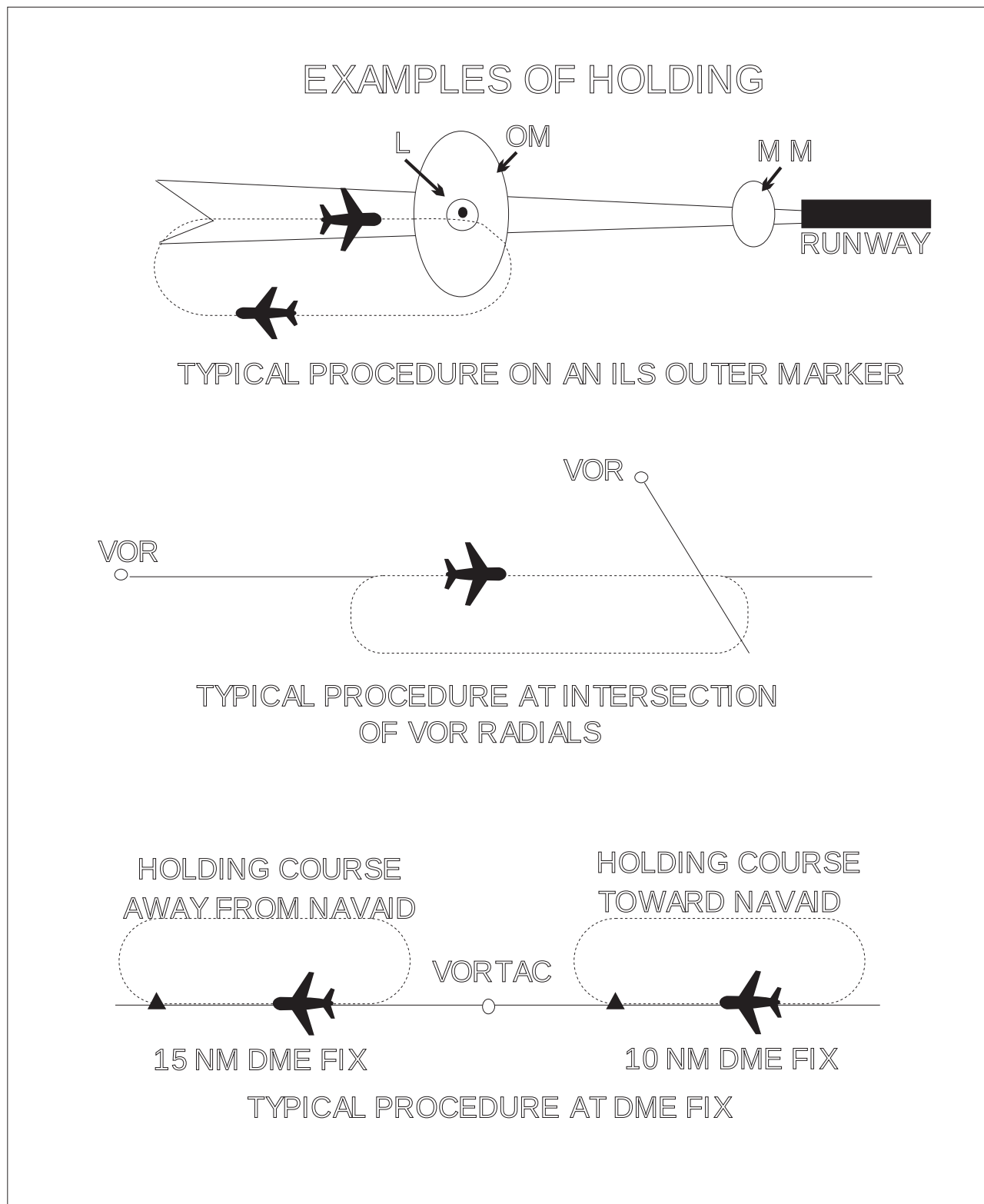
FIG 5-3-2 Holding Patterns
