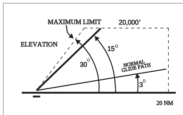
FIG 1-1-9 Coverage Volumes Elevation
