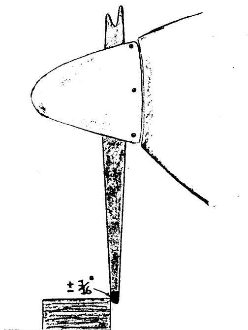
FIGURE 5 - Propeller Tracking
