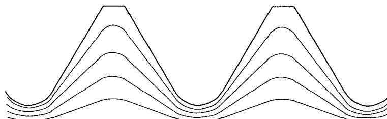
Figure 4: Example of a regular grain flow in a threaded surface
