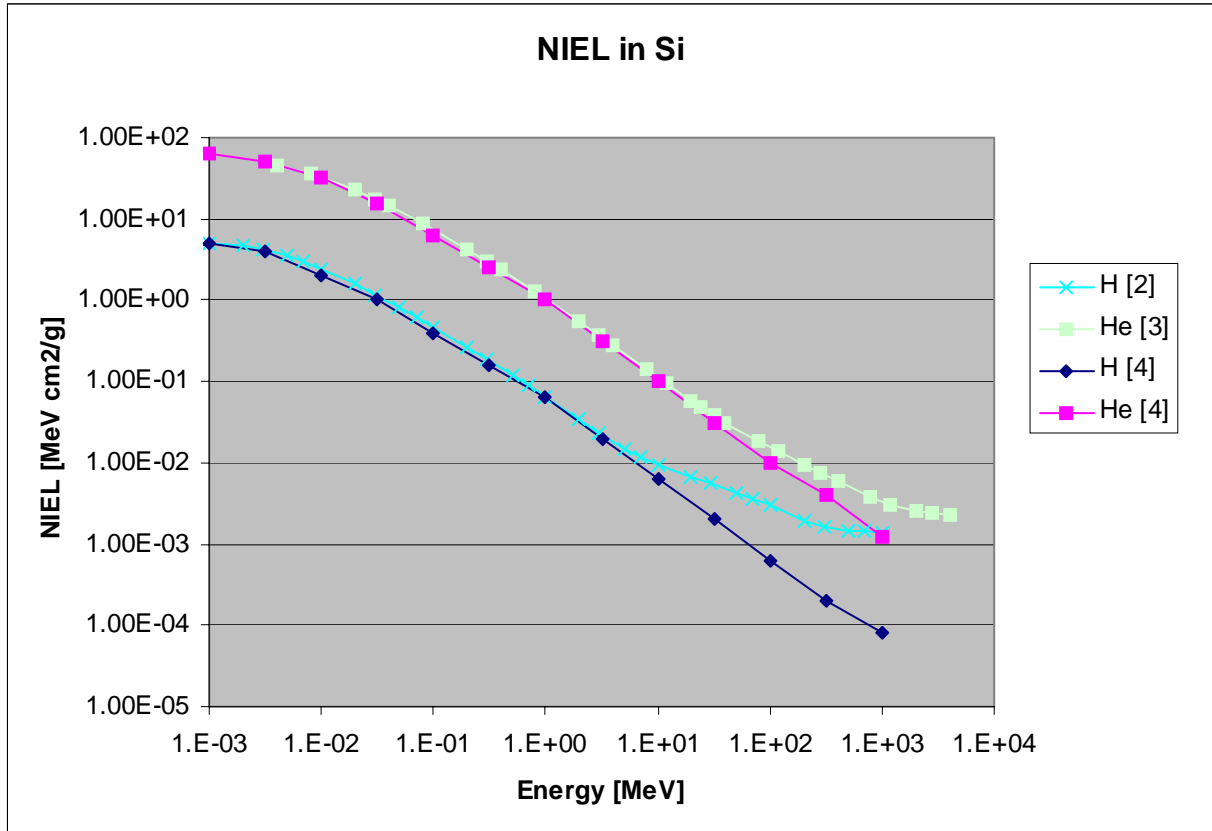
Figure 48. NIEL in Silicon for H and He from different data sources
