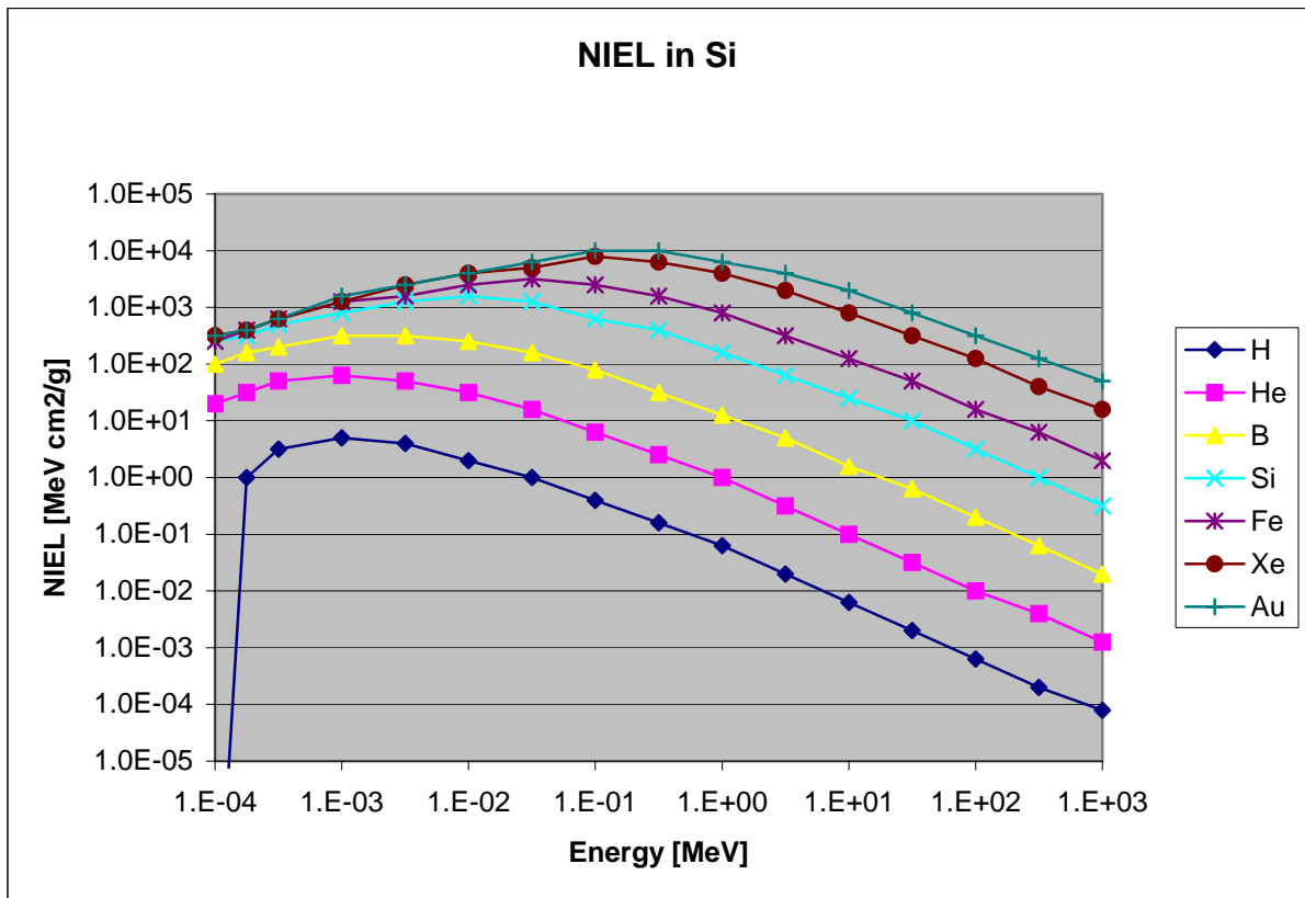
Figure 47. NIEL in Silicon for selected heavier ions
