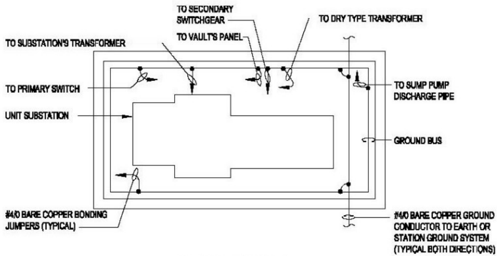
GROUNDING PLAN
