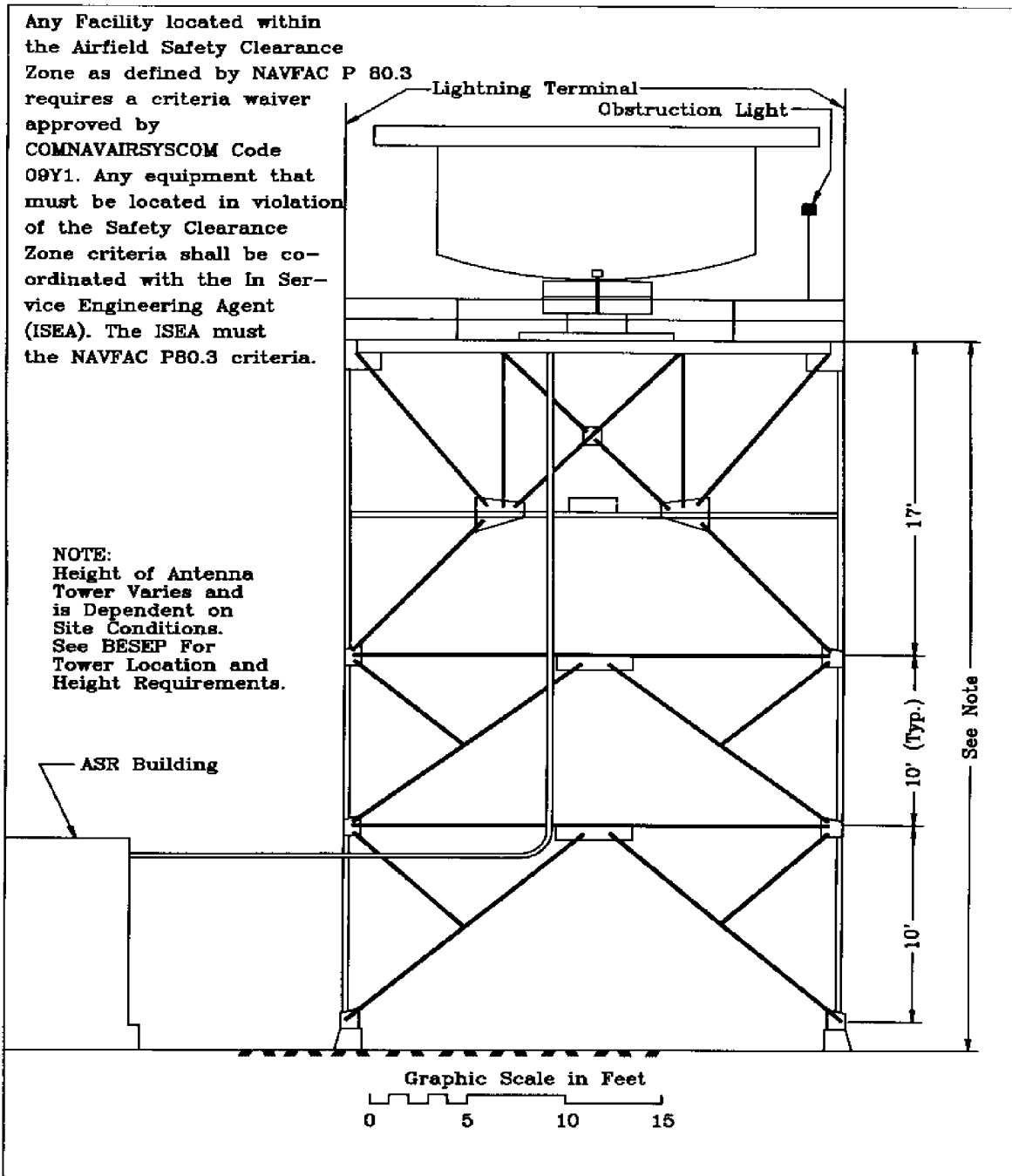
Figure 2 ASR Antenna Tower
