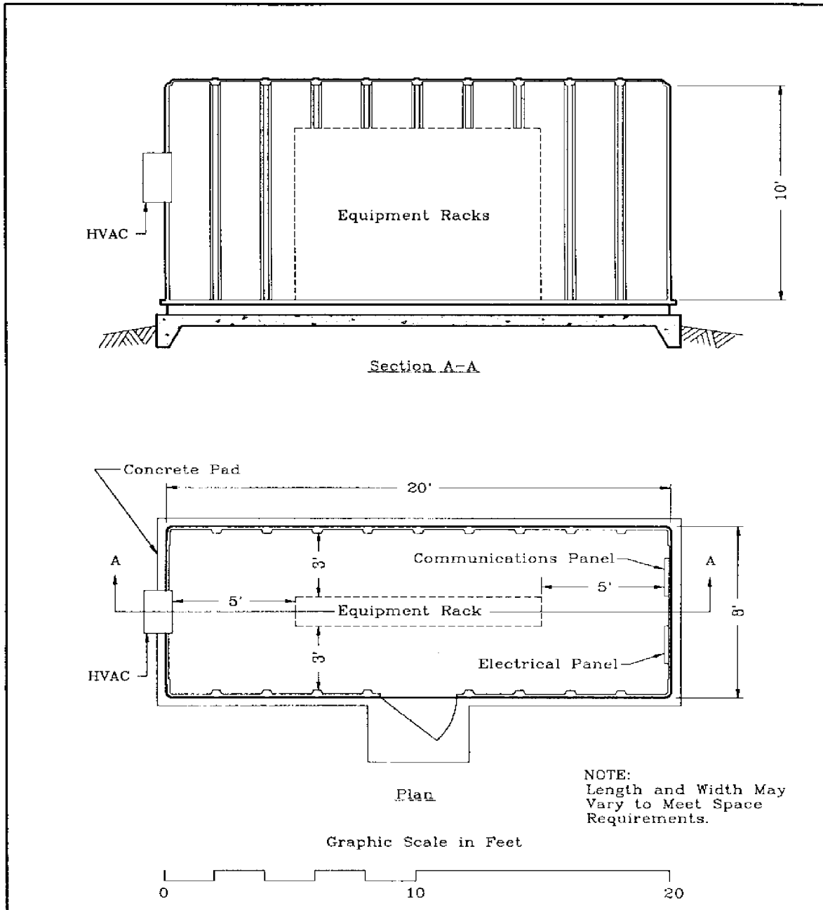
Figure 3 Prefabricated Building
