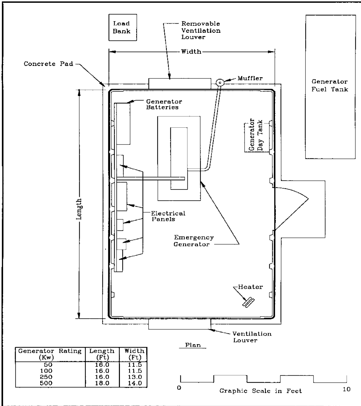
Figure 5 Prefabricated Indoor Emergency Generator Room Layout
