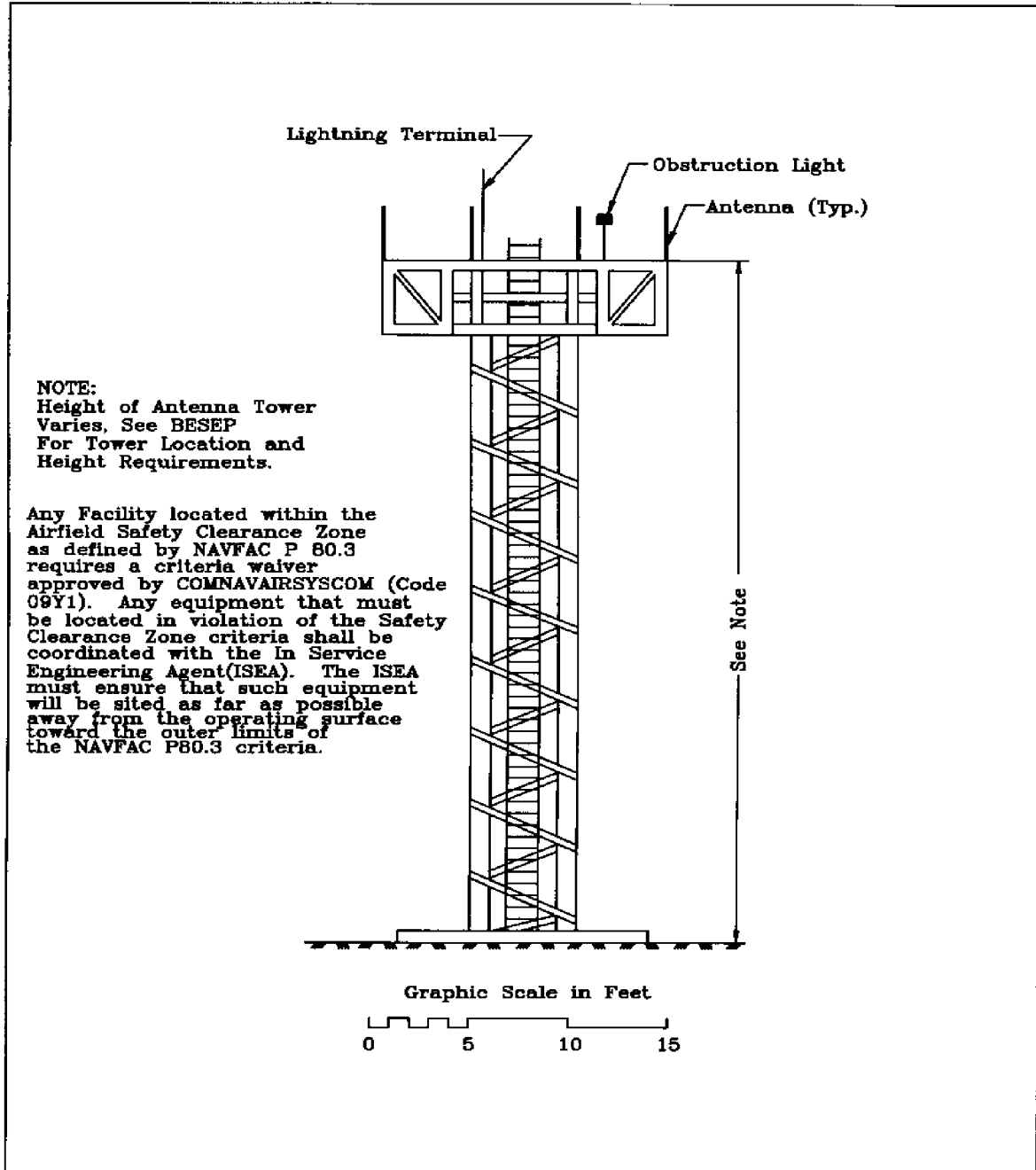
Figure 1 Radio Antenna Tower
