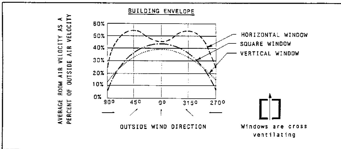
Figure 32 Window Shape Performance in Relation to Wind Direction
