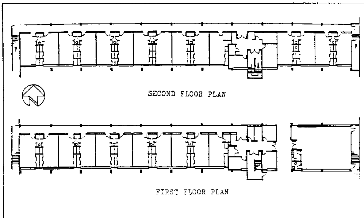
Figure D-2 Plans of Building #1031
