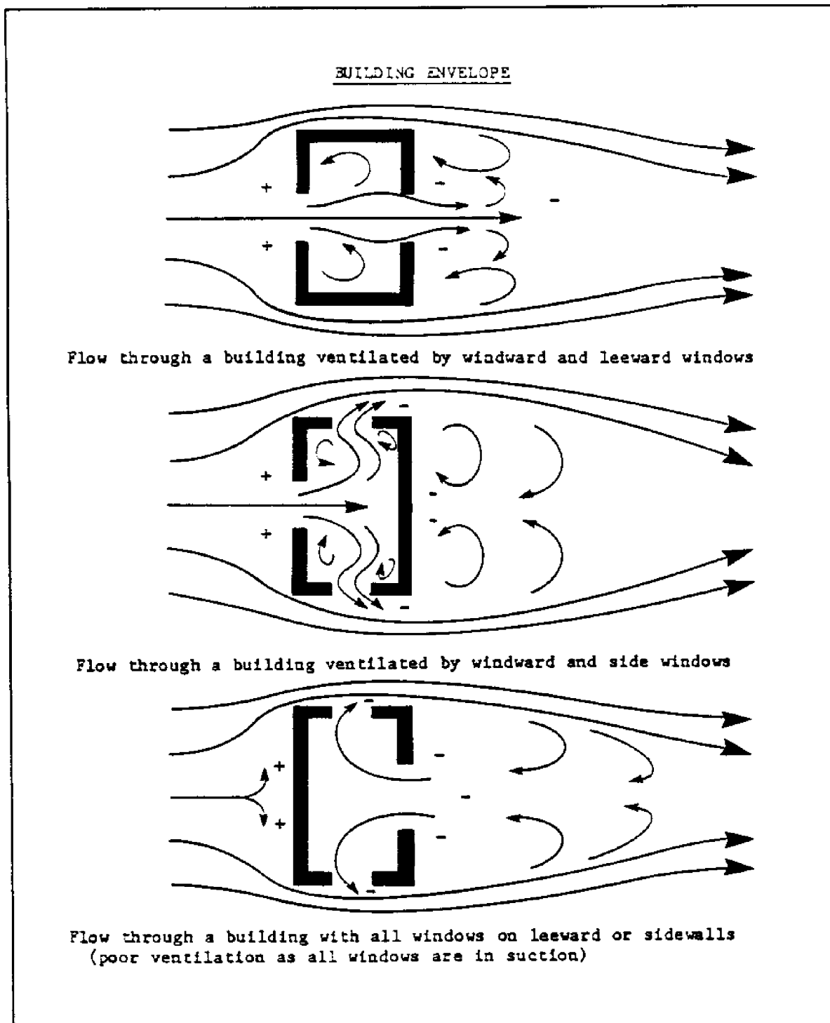
Figure 27 Air Flow Patterns and Pressure Zones
