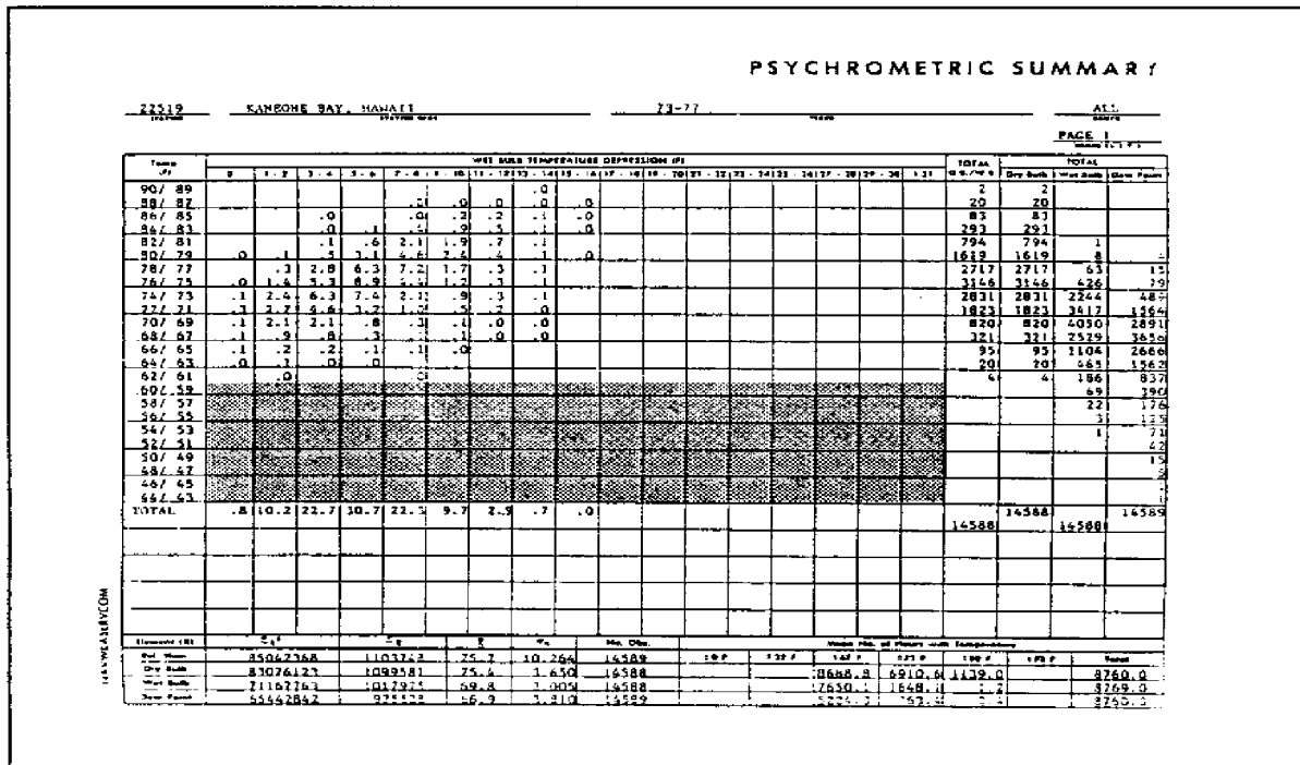
Figure B-8 Determining Requirement for Open or Infiltration-Resistant Envelope
