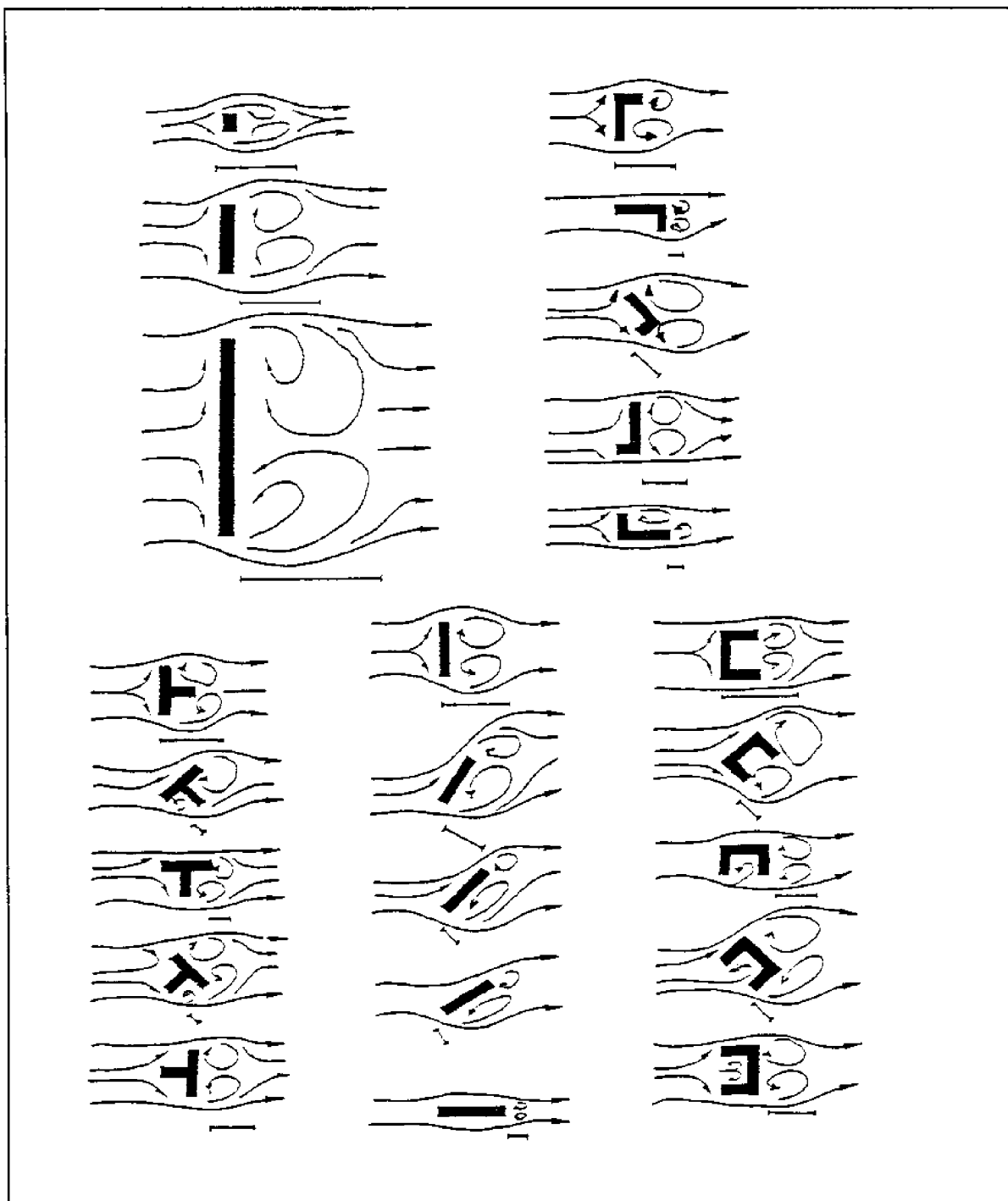
Figure 7 Effect of Wind Incidence Angle, and the Length and Shape of Obstructions on Downwind Wake
