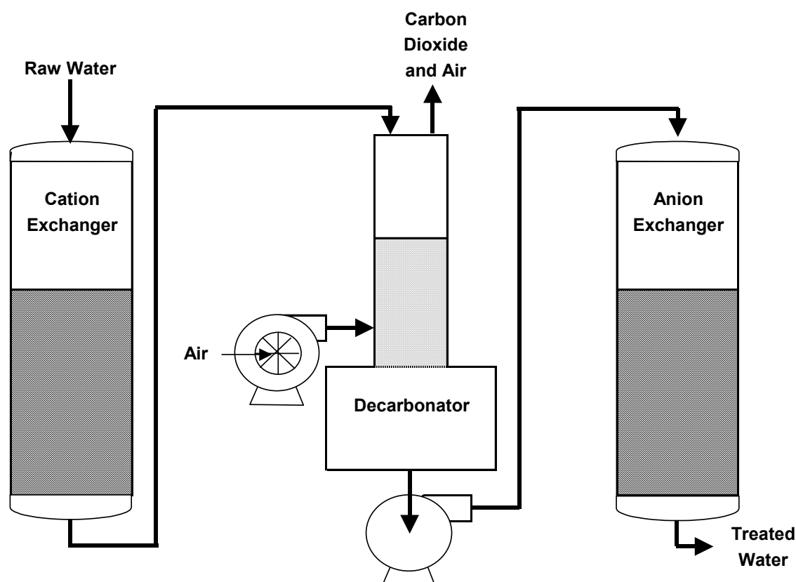
Figure 2-4. Demineralization Process
