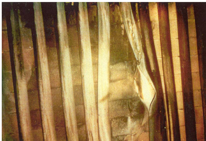
Figure 3-8. Failed Boiler Tube
