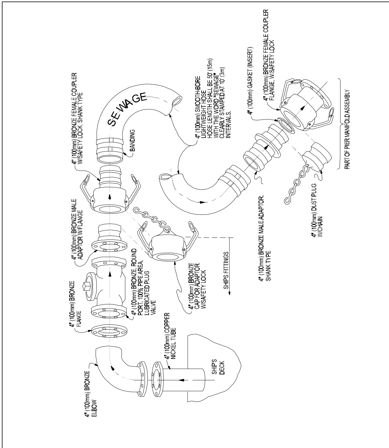
Figure 6 Ship-to-Shore Sewage Hose Components
