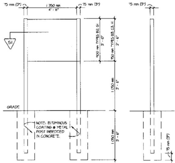
FRONT ELEVATION AND SECTION: TYPES B2, B3, C3, G1, H2 SCALE: 1/4"=1'-0"
