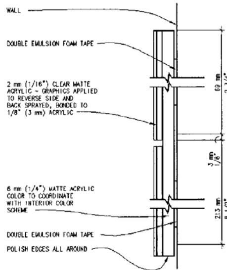
S4 ALTERNATE DETAIL, SIGN TYPE CC2, MULTIPLE
