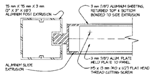
S4 ALT. HORIZONTAL SECTION (EXTRUDED POST)
