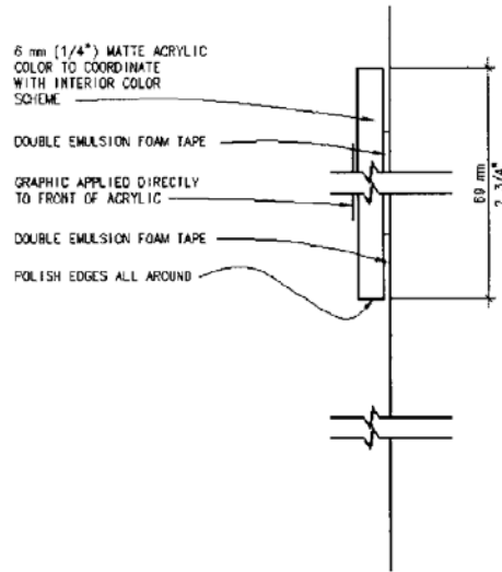
S3 VERTICAL SECTION, TYPE CC2
