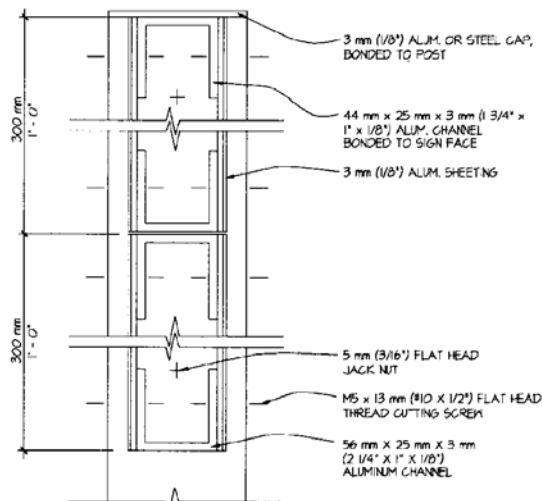
S3 VERTICAL SECTION
