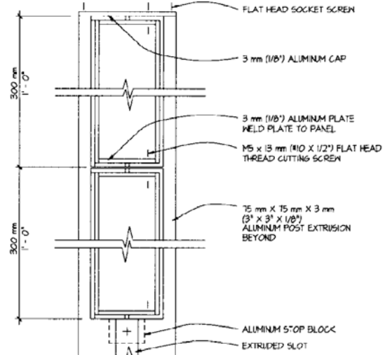
S5 ALTERNATE VERTICAL SECTION
