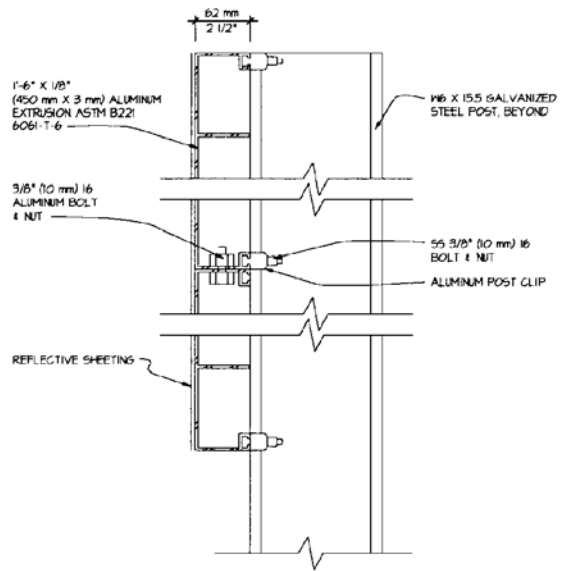
S2 VERTICAL SECTION SCALE 1 1/2"=1'-0"
