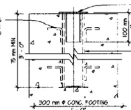
S4 PIPE SLEEVE SECTION
