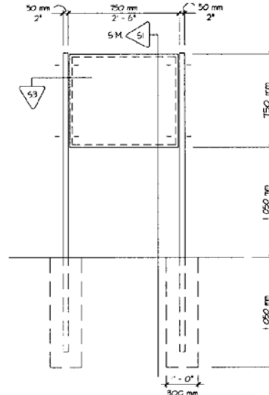
FRONT ELEVATION: SIGN TYPE F2, F3
