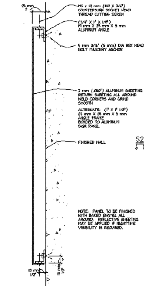
S1 VERTICAL SECT: SIGN TYPES B4 C54 FREESTANDING SIGN
