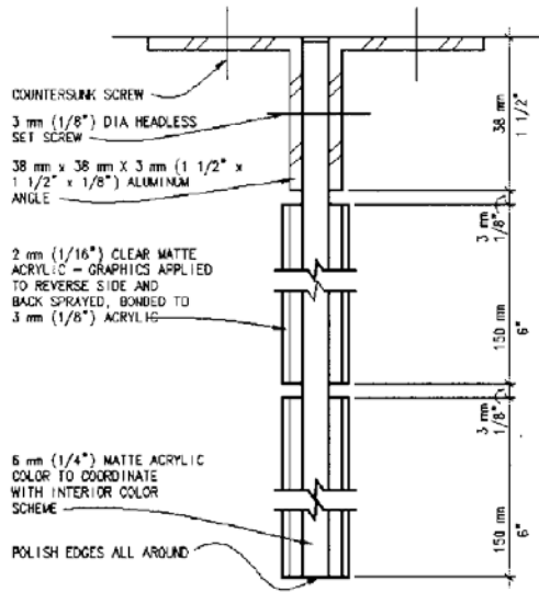
S2 ALTERNATE DETAIL, SIGN TYPE CC1, MULTIPLE
