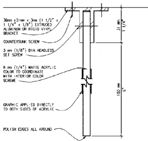
S1 VERTICAL SECTION, TYPE CC1
