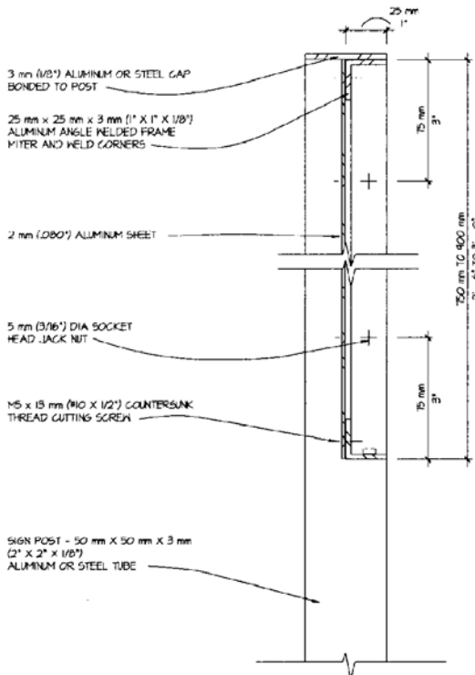
S2 VERTICAL SECTION
