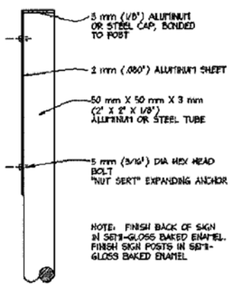
S4 FREESTANDING SIGN
