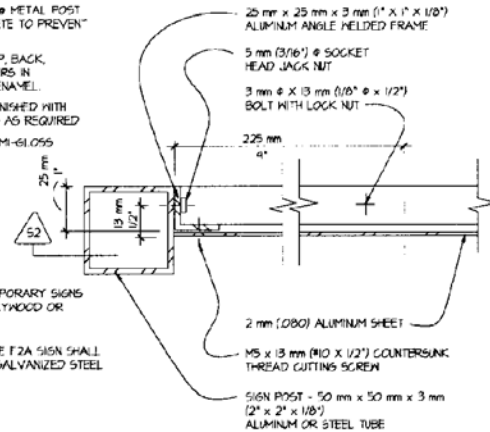
S3 HORIZONTAL SECTION
