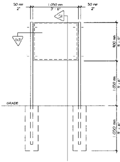
FRONT ELEVATION: SIGN TYPE F2
