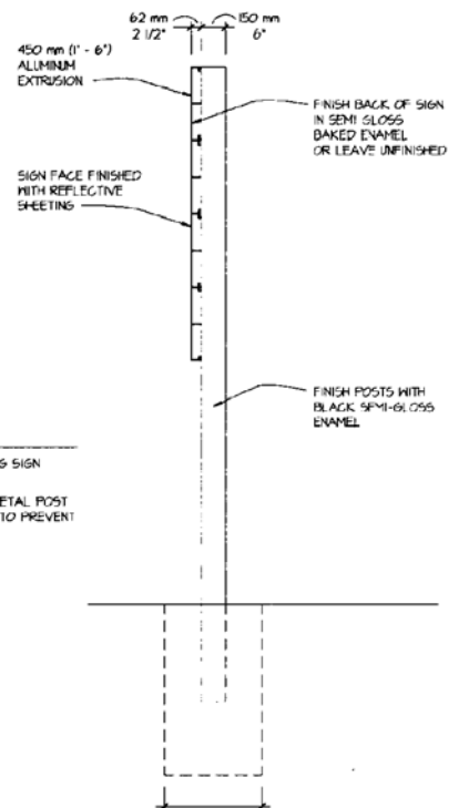
SECTION SCALE 1/4"=1'-0"
