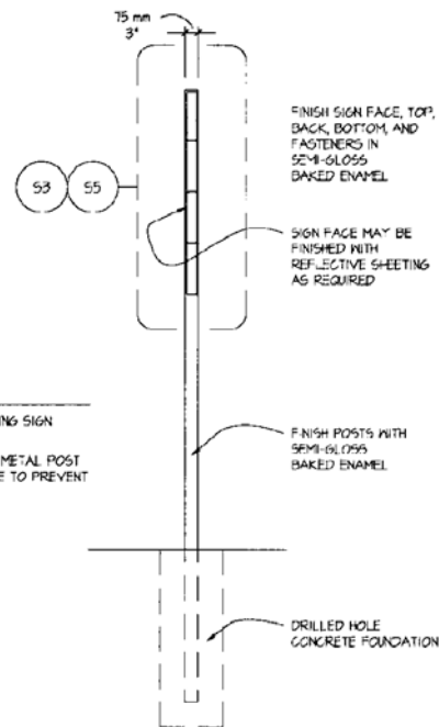
S1 VERTICAL SECTION
