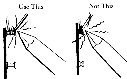
Figure 4-26. Terminals Should Be Long Enough to Prevent Damage to Insulation During Repairs
