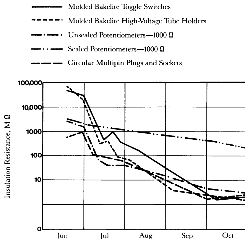
Figure 10-7. Reduction in Insulation Resistance of Typical Electronic Components Exposed For Five Months in Tropical Jungle
