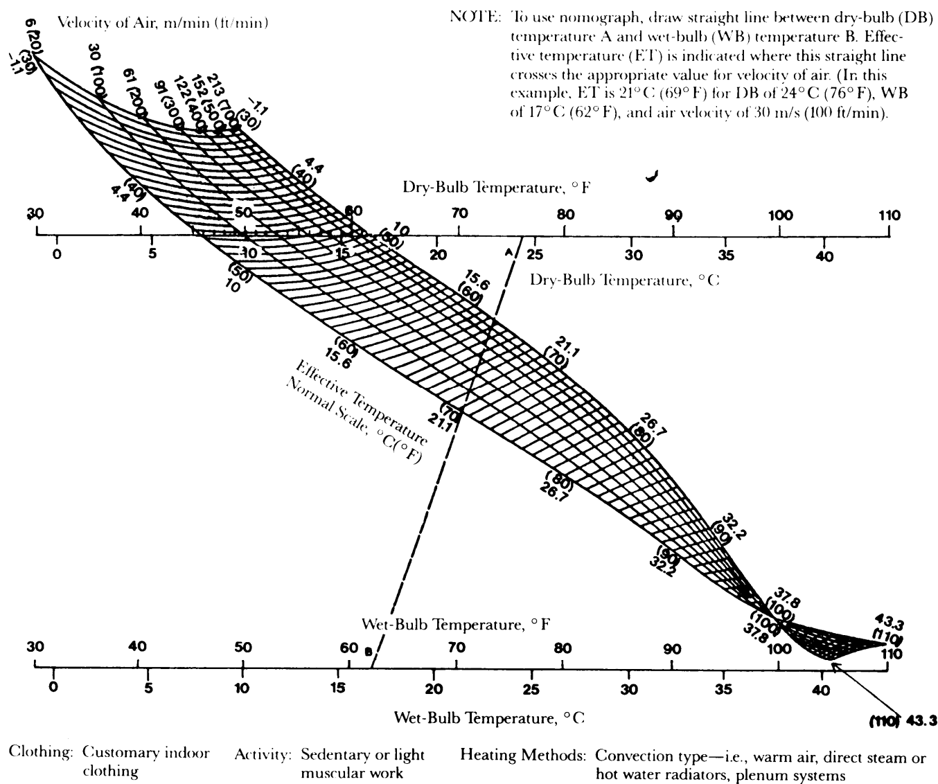
Figure 10-2. Deriving Effective Temperature
