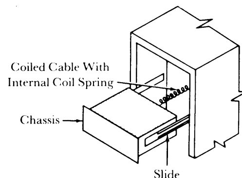
Figure 4-29. Methods for Recoiling Service Loops in Sliding Chassis (Ref. 3)
