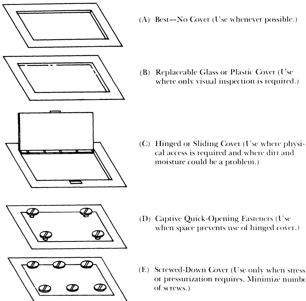
Figure 4-1. Types of Covers and Accesses (Ref. 3)
