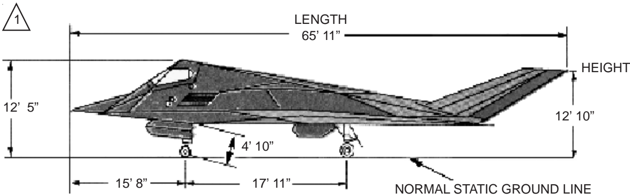
FIGURE 2. Example of aircraft dimensions.
