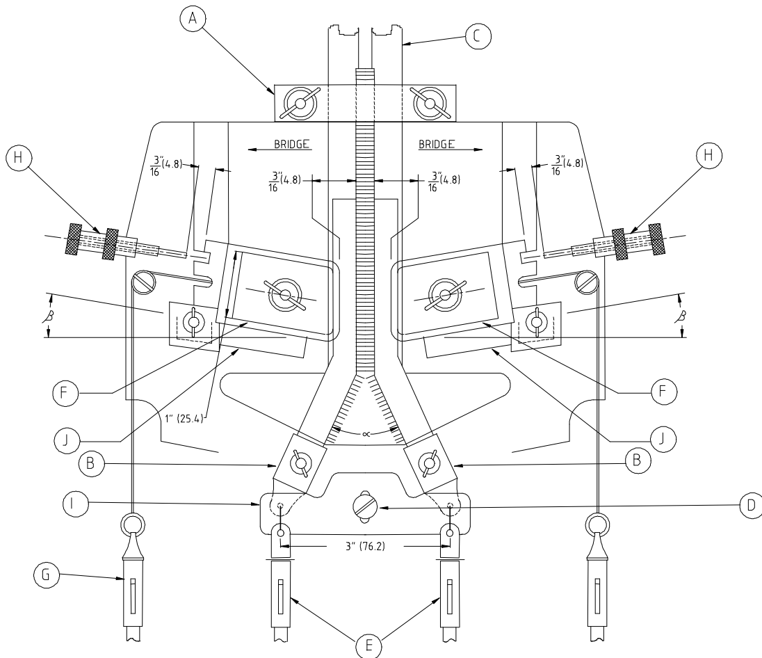
Fig. VIII- Endurance Machine
