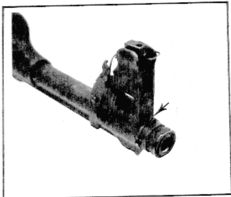
FIGURE 51. LOCKING PLUNGER
