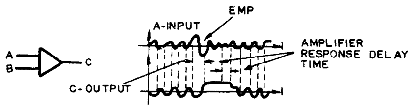
(c) AMPLIFIER UPSET
