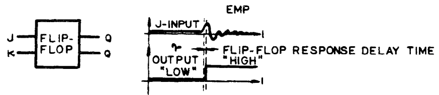
(a) FLIP - FLOP UPSET
